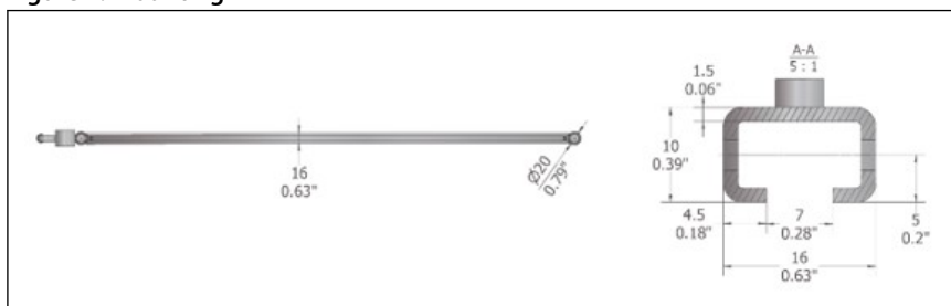
Figure 2: Mounting
