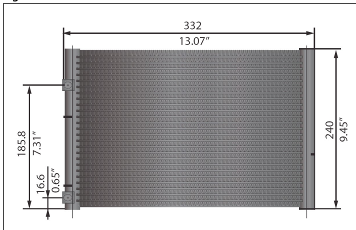
Figure 1: Dimensions
