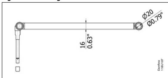
Figure 2: Mounting
