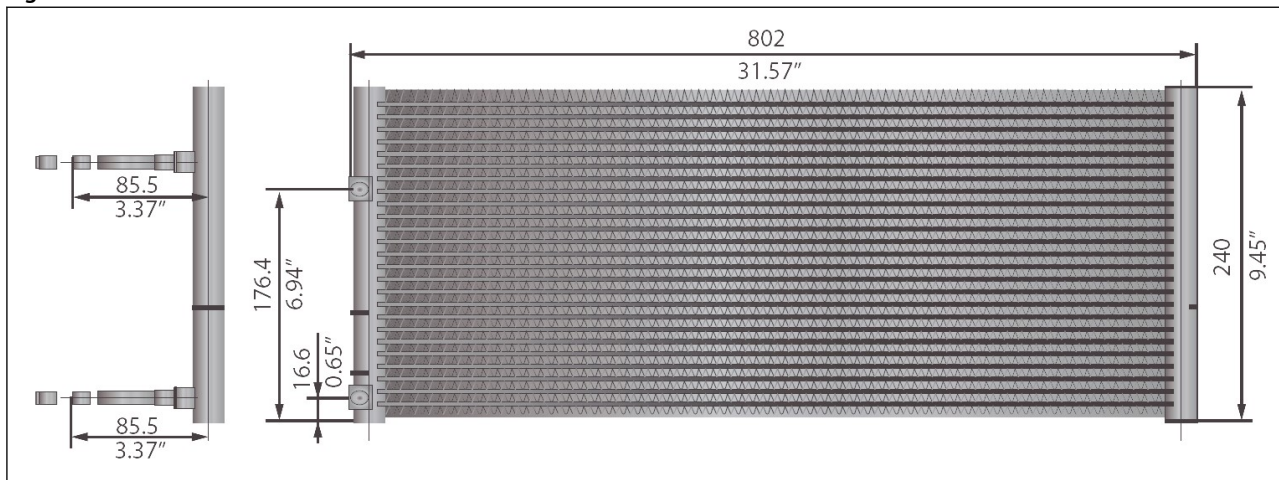
Figure 1: Dimensions
