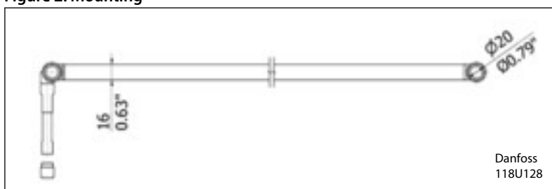
Figure 2: Mounting
