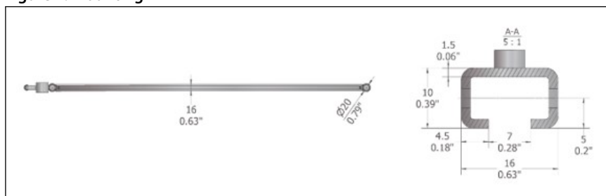
Figure 2: Mounting
