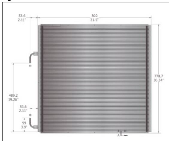
Figure 1: Dimensions
