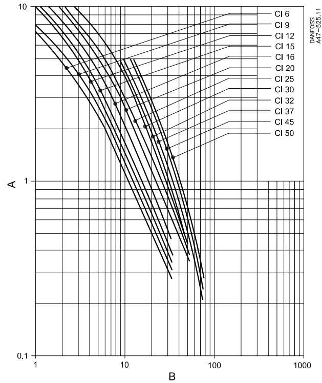
Contactors CI 6/9/12/15, CI 16/20/25/30, CI 37/45/50, load categories AC-1
