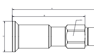
Figure 2 Socket
