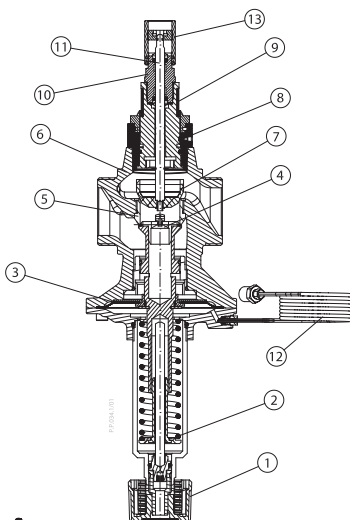
Abb. 13: AB-PM DN 40–50
