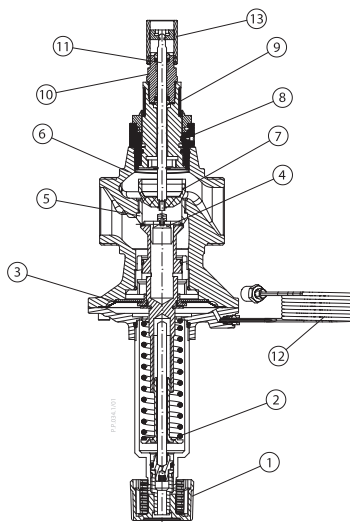
Obr. 13 AB-PM DN 40–50
