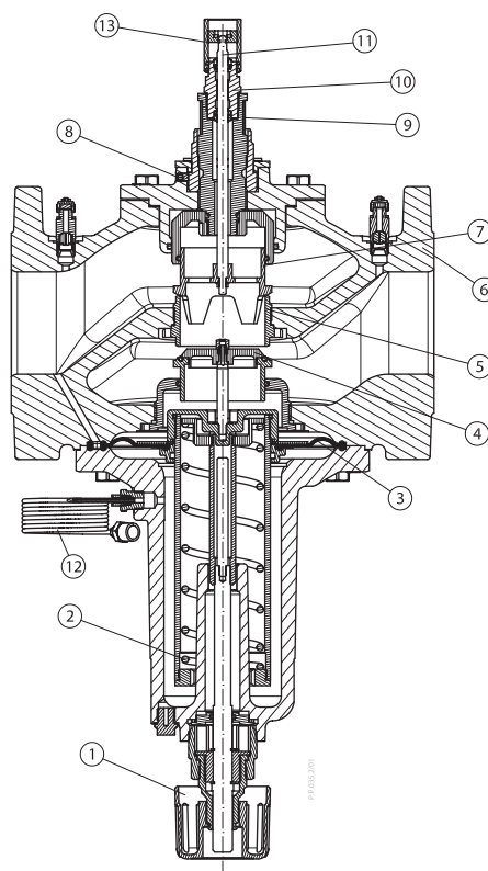
Obr. 14 AB-PM DN 65–100
