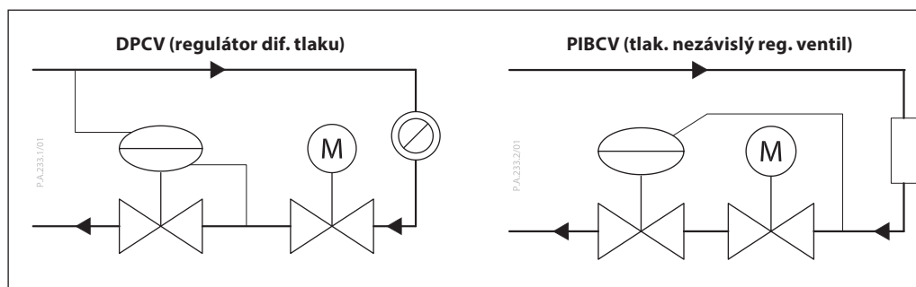
Obr. 14 AB-PM DN 65–100
