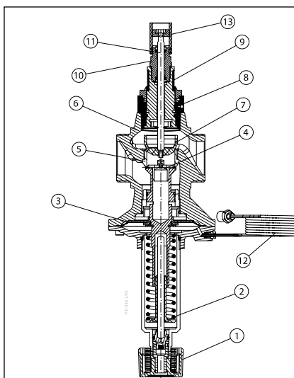
Fig. 13 AB-PM DN 40 – 50
