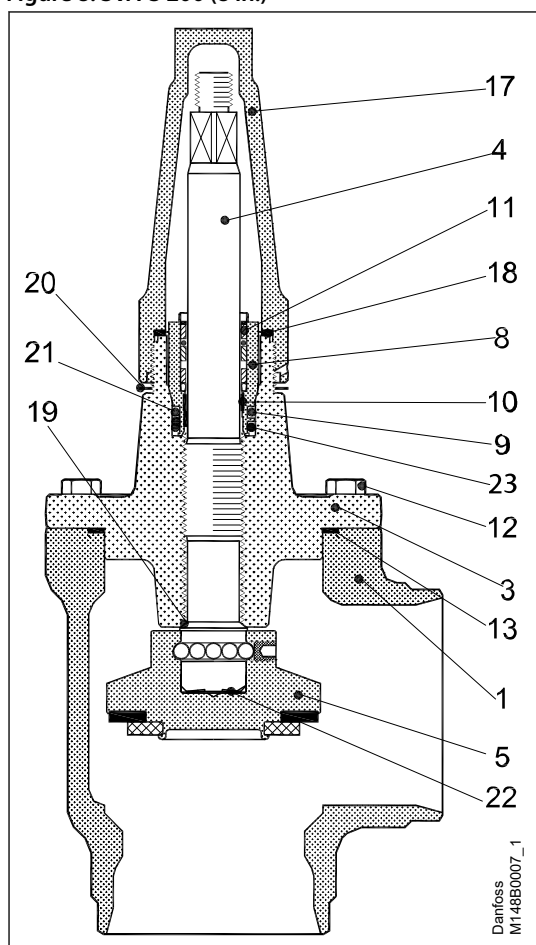
Figure 8: SVA-S 200 (8 in.)
