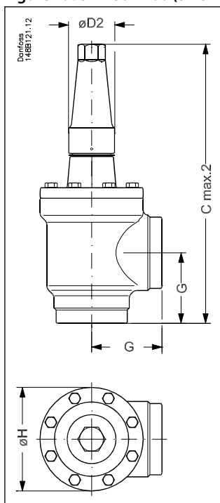
Figure 19: SVA 80 - 200 (3 - 8 in.) angleway version with cap
