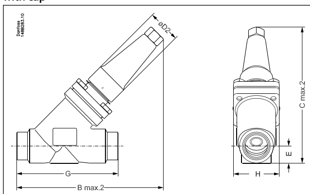
Figure 16: SVA 15 - 40 (½ - 1½ in.) straightway version with cap
