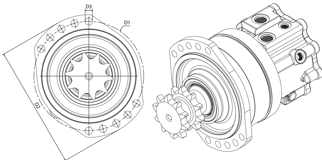
S54: 10-hole oval mounting flange - 60 degrees rotation
