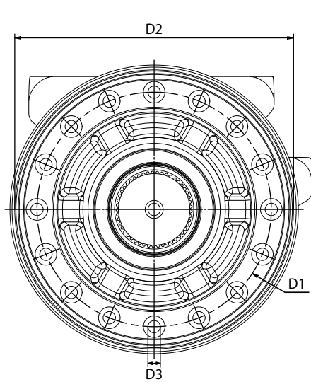
S09: 16-hole circular mounting flange
