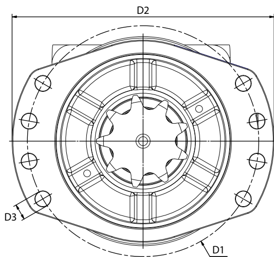
S11: 8-hole oval mounting flange - Parallel
