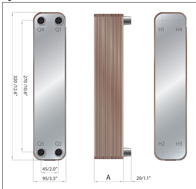
Figure 1: Dimensions
