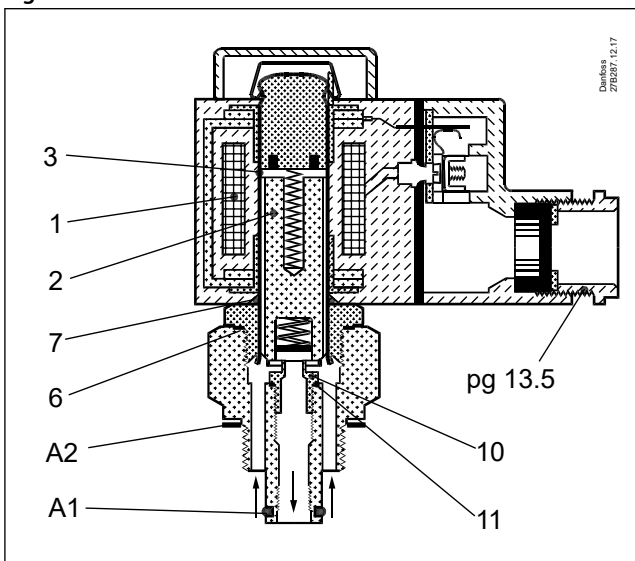
Figure 11: EVM
