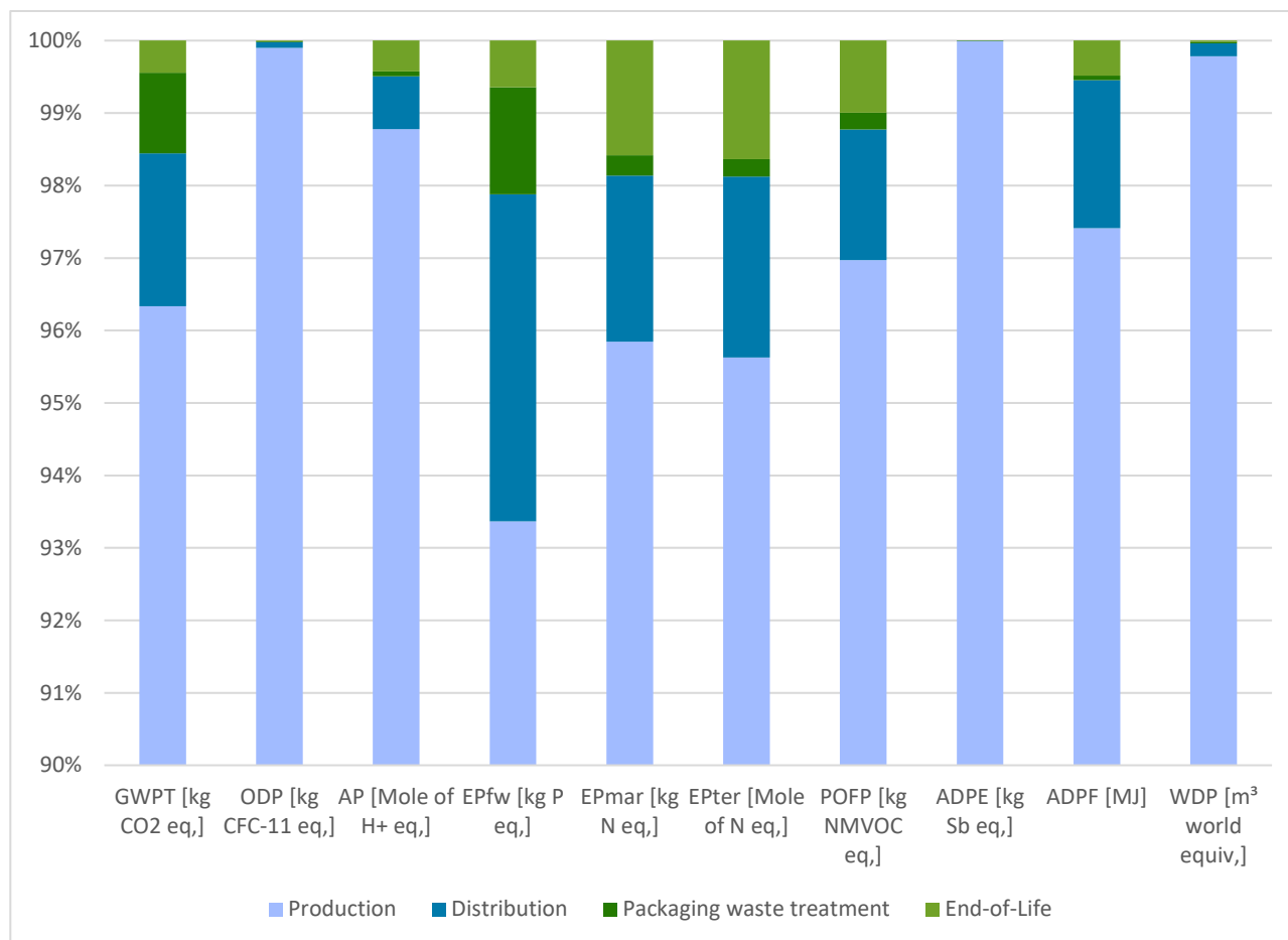
Figure 4: Breakdown of environmental impacts by life cycle stages (Average of Landfill and Recycling End-of-Life scenario/only Landfill scenario) See Table 5 and 6 for descriptions of environmental impact indicators).
