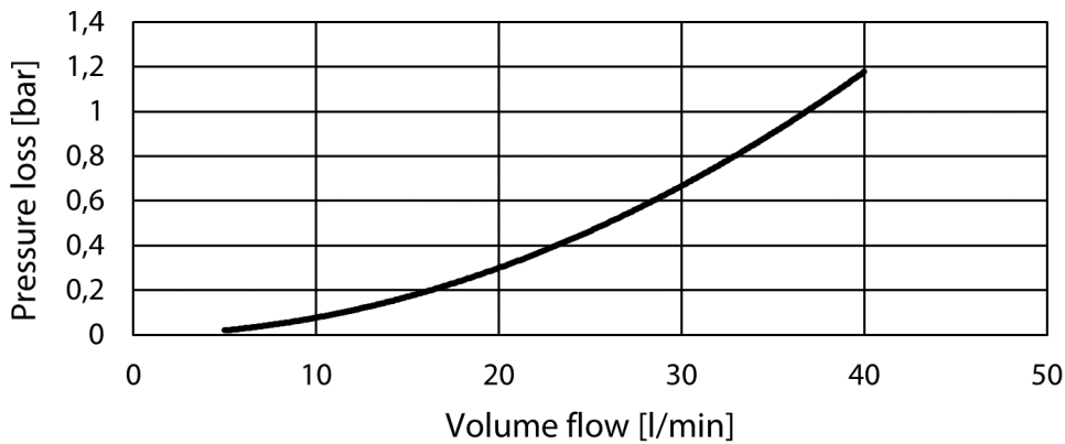
Picture 1 Pressure loss vs coolant flow
