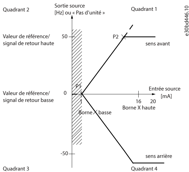
Illustration 48: Dimensions de la zone morte
