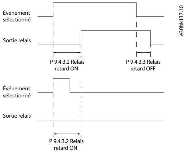
Illustration 82: Relais, retard ON
