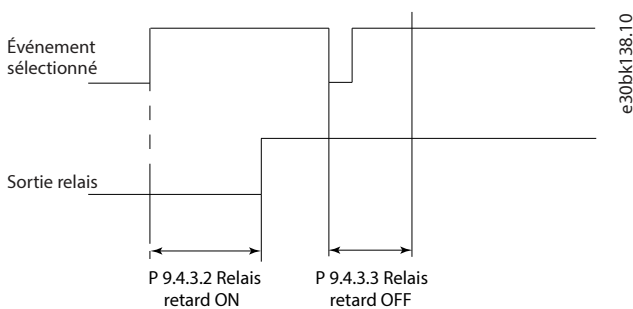
Illustration 83: Relais, retard OFF
