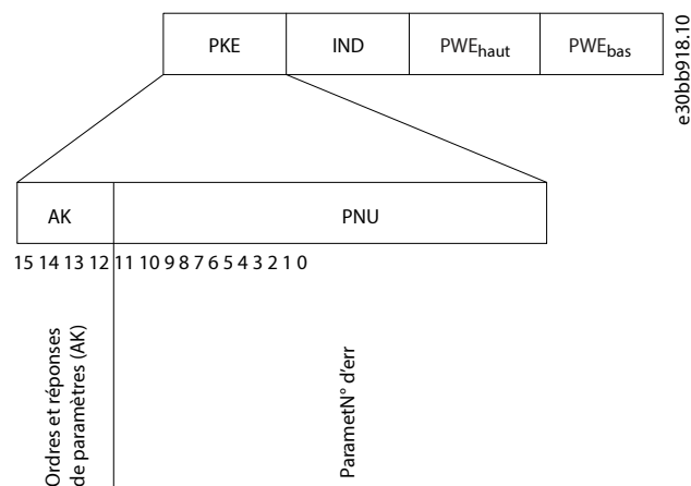
Illustration 60: Champ PKE
