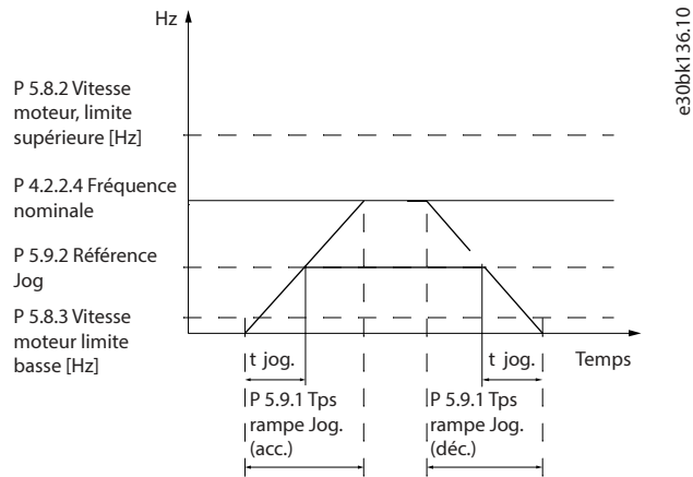
Illustration 77: Tps rampe Jog.
