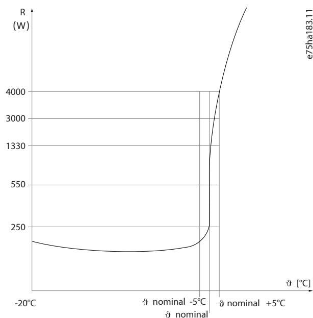
Illustration 72: Profil PTC
