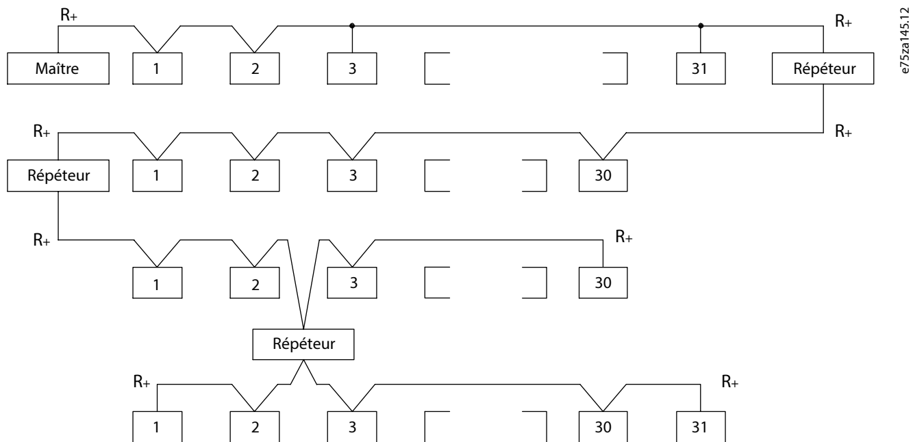
Illustration 51: Interface bus RS485
