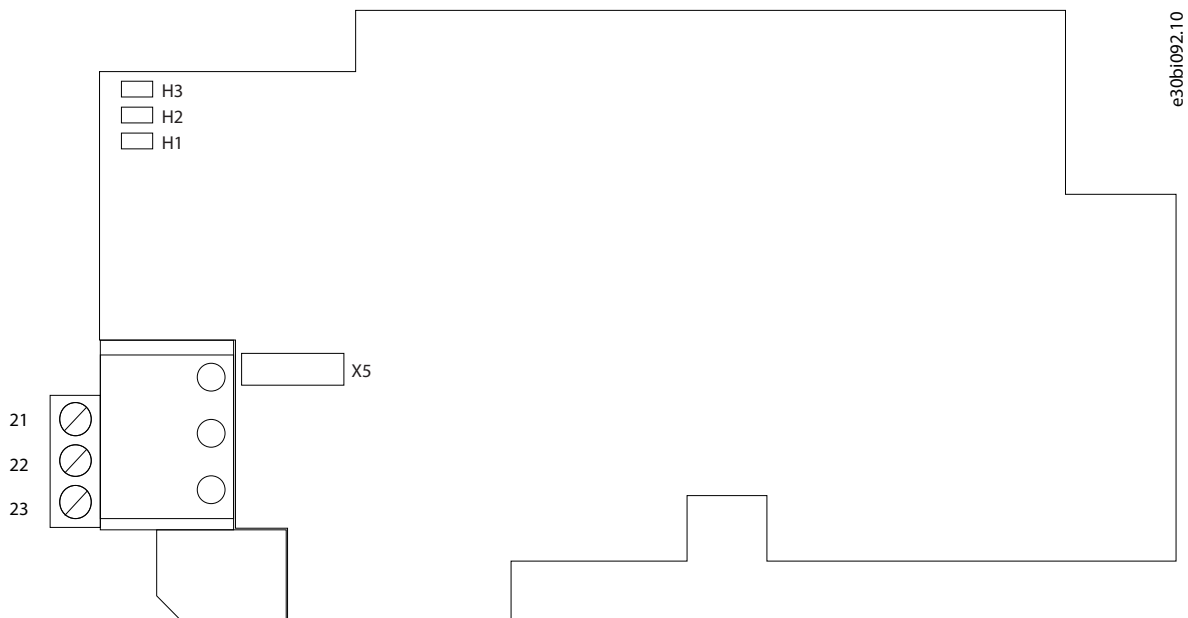
Illustration 40: The OPTC4 Option Board Layout
