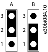
Illustration 36: The Settings of the Jumper X1, Cable Shield Grounding, Positions A, B, and C.
