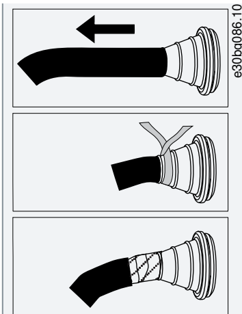
Illustration 2: IP55
