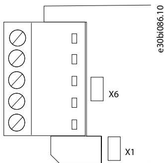
Illustration 17: Jumper Locations on OPTC3/C5
