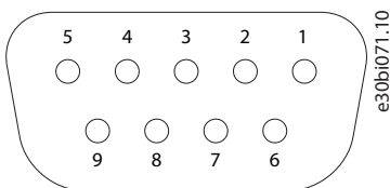
Illustration 7: The Sud-D9 Connector
