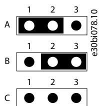
Illustration 33: The Settings of the Jumper X7 on 70CVB01124 (141X3915) and 70CVB01555 (141X4133), Bus Terminal Resistor, Positions A, B, and C
