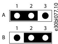
Illustration 13: The Settings of the Jumper X13, Termination Resistor, Positions A and B
