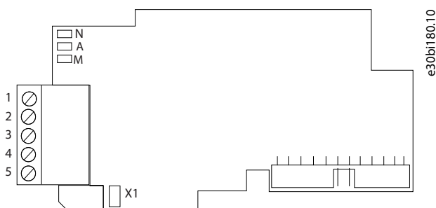
Illustration 52: LED Indications on VACON® OPTC7 Option Board
