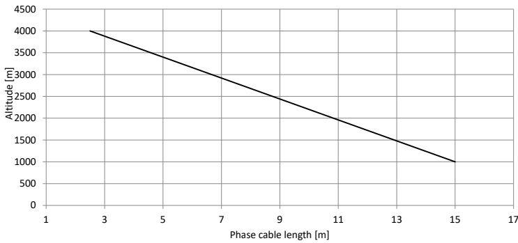
Picture 2 Allowed altitudes vs phase cable length
