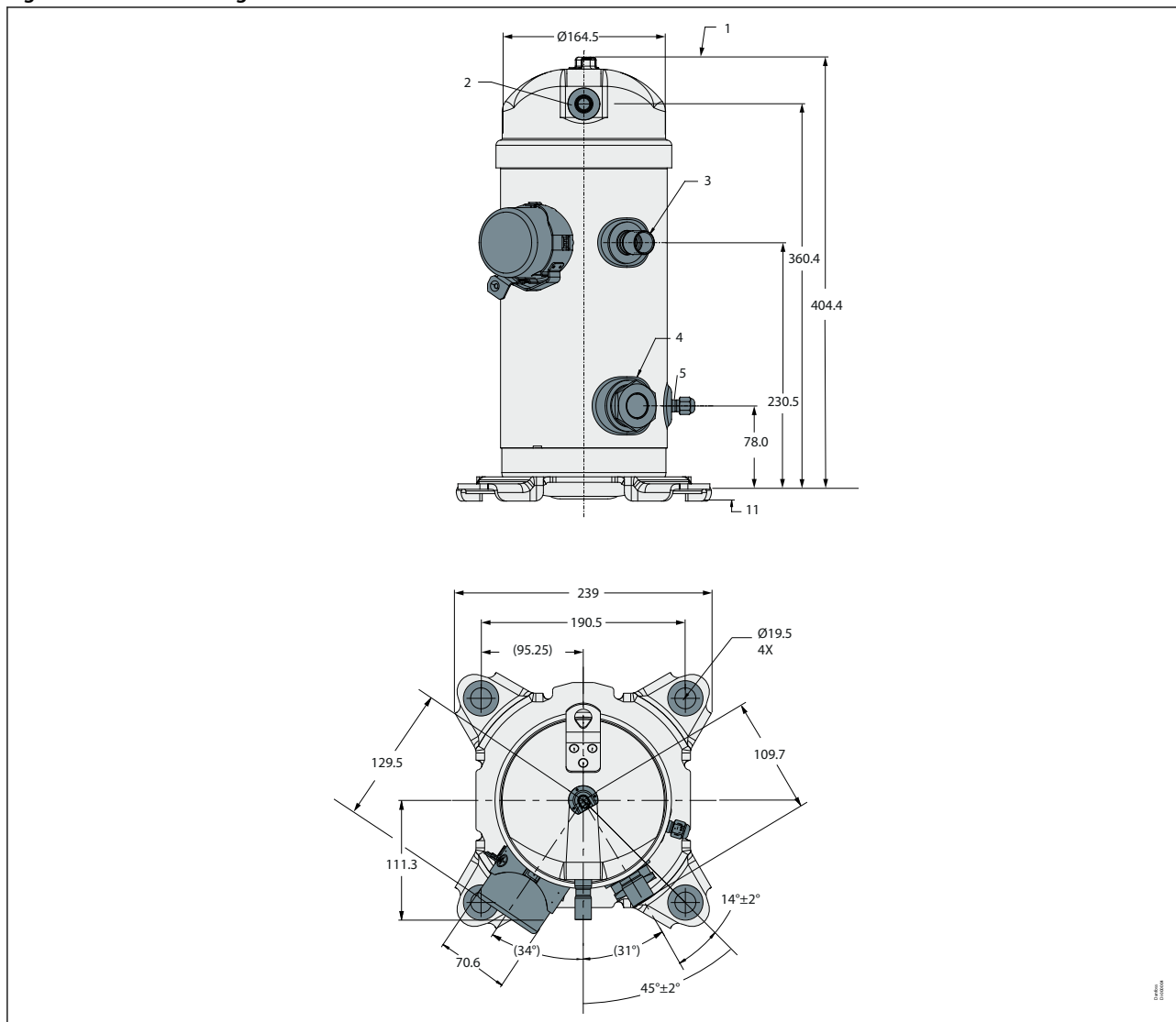
Figure 6: Outline drawing
