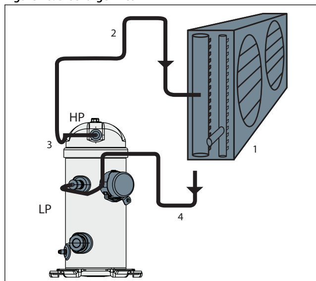
Figure 16: Discharge lines
