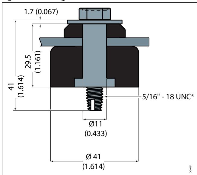
Figure 13: Mounting
