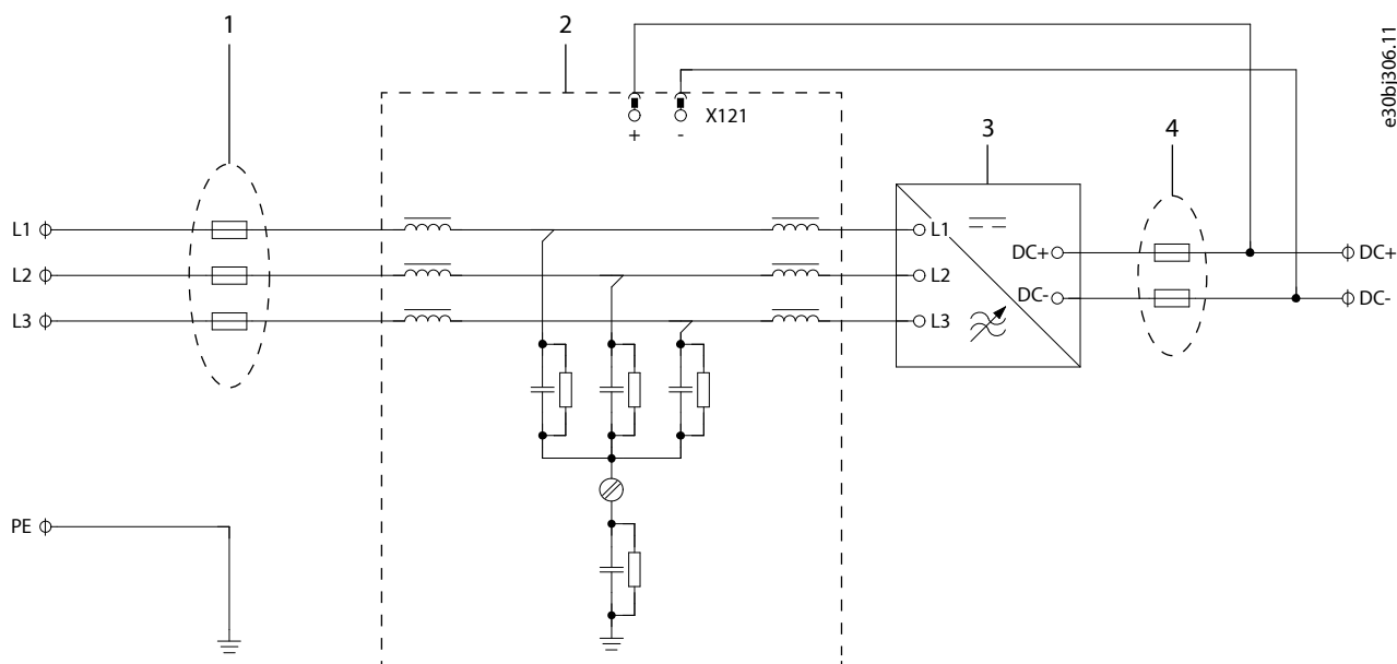
Figure 34: Diagram of the LCL Filter Fan Supply
