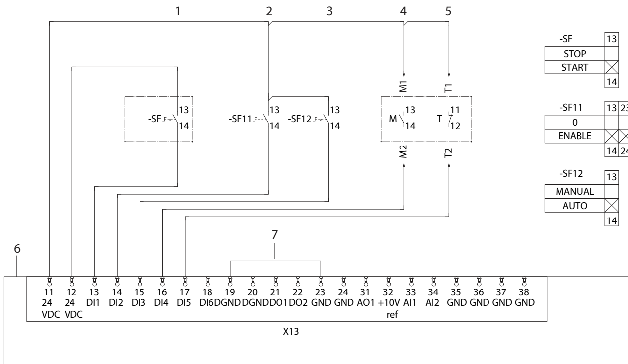
Figure 119: Pre-charging Control Wiring Diagram
