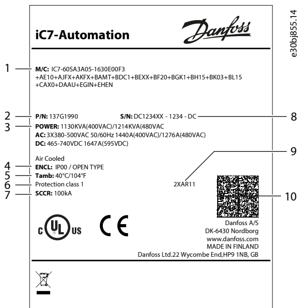
Figure 10: Product Label for iC7 Series Air-cooled System Modules
