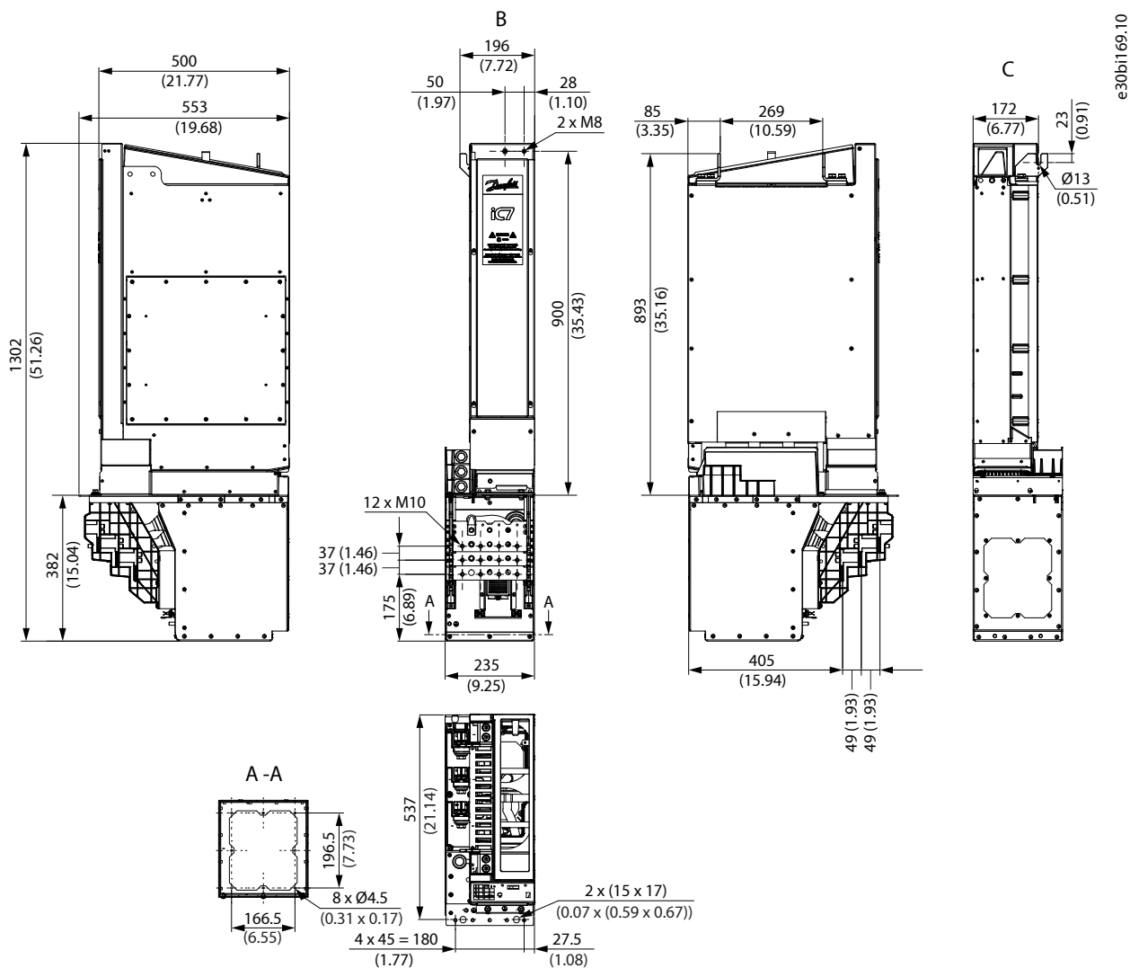
Figure 78: Dimensions of the Inverter Module in mm (in), IR10 with Short Integration Unit (+AE01)
