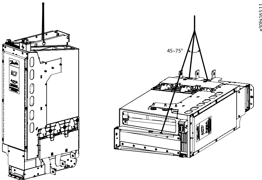
Figure 3: Lifting the Upper Part of the LCL Filter
