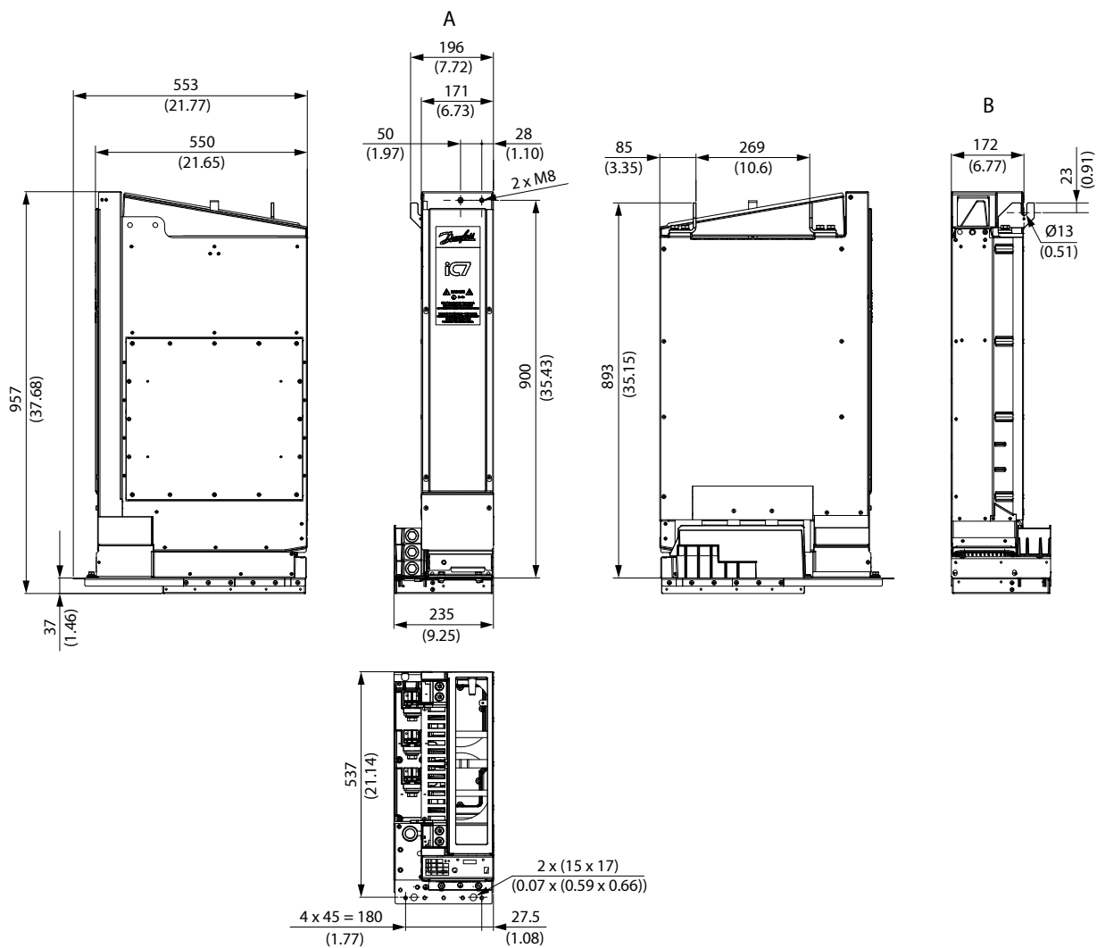
Figure 82: Dimensions of the AFE Module, AR10, with the Short Integration Unit (+AE01) in mm (in)
