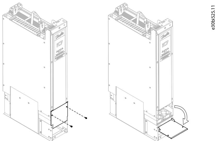
Figure 71: Releasing and Opening the Fan Cover
