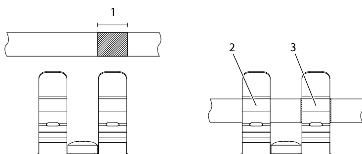
Figure 66: Stripping the Cable and Using the Grounding Plates
