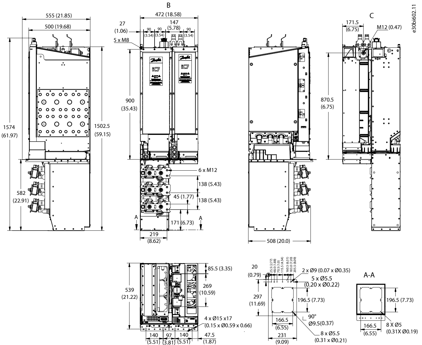
Figure 88: Dimensions of the LCL Filter, LCL11, and the AFE Module, AR11, with the Short Integration Unit (+AE01) in mm (in)
