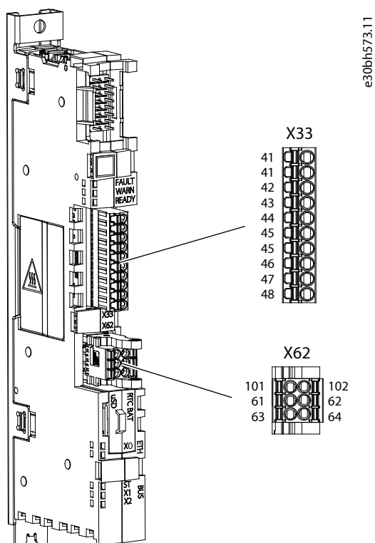
Figure 53: Control Board Terminal Block and Terminal Numbering
