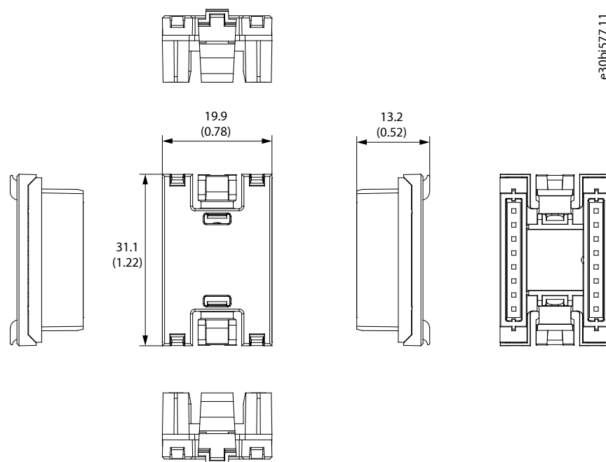
Figure 105: Dimensions of the Option Connector in mm (in)
