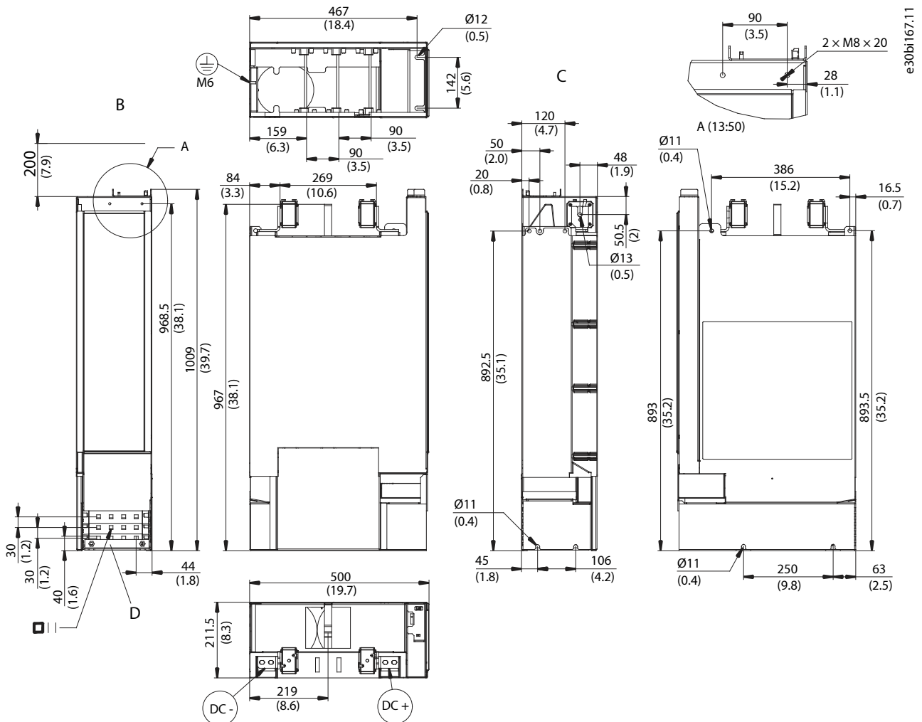
Figure 76: Dimensions of the Inverter Module in mm (in), IM11
