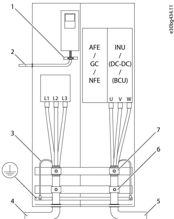
Figure 30: Cabling Principle
