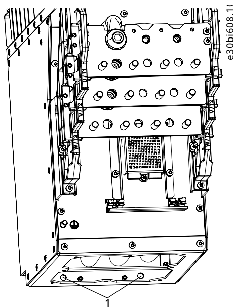
Figure 17: Bottom Screws of the Short Integration Unit, IR10, IR11
