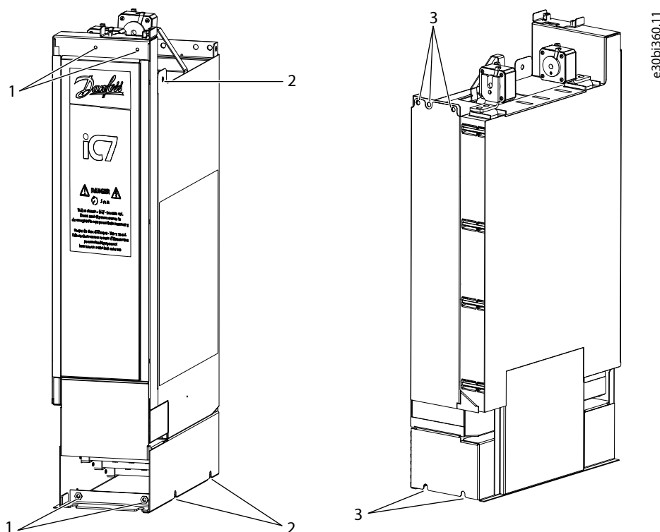
Figure 12: Mounting Holes for IM10, IM11, AM10, AM11
