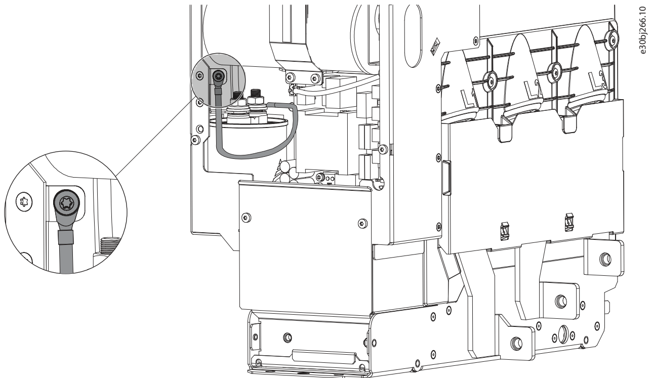
Figure 38: EMC Protection Level 4
