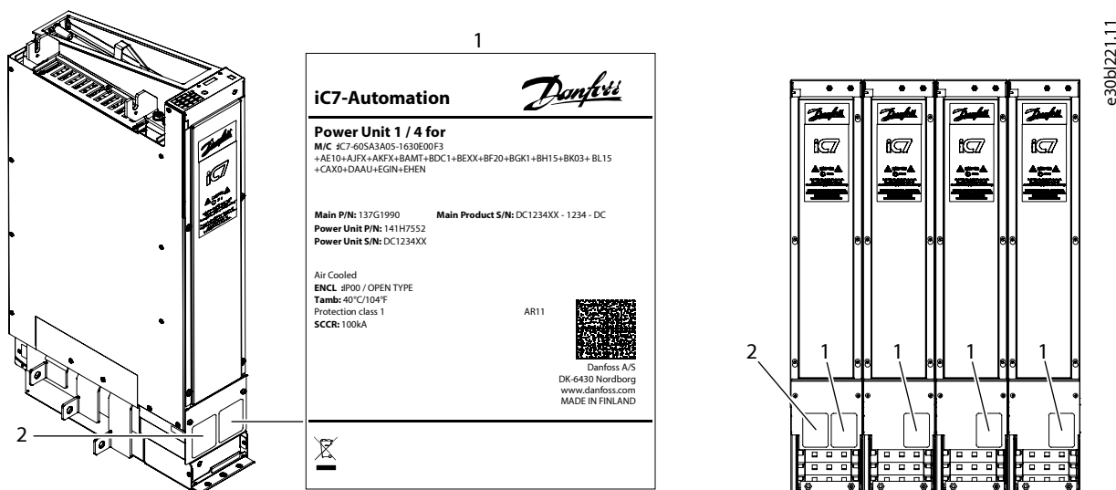
Figure 7: Locations of the Labels on System Modules
