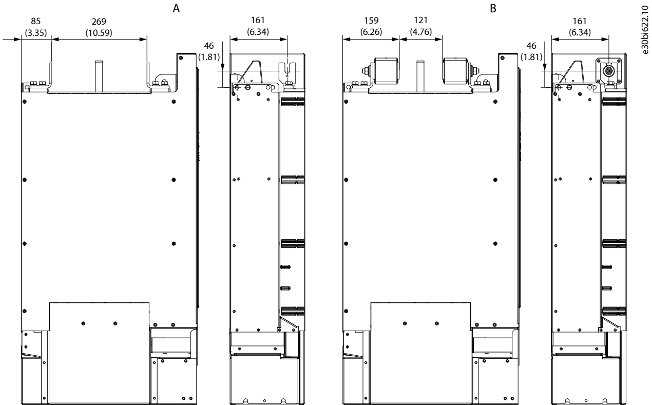
Figure 99: Dimensions for DC Fuses, IM11, in mm (in)
