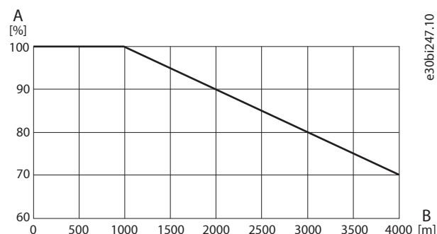
Figure 124: Output Current Derating vs. Installation Altitude
