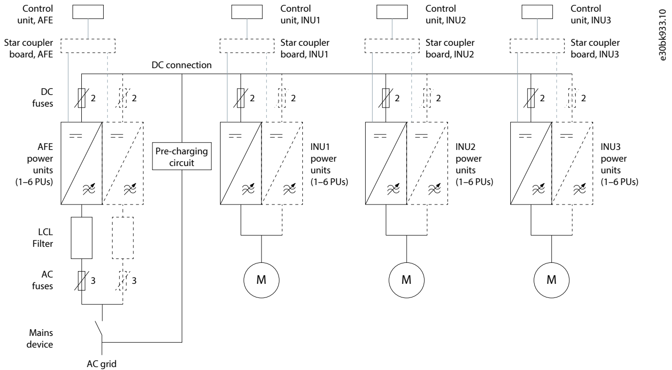
Figure 41: DC Connections of a Drive Lineup
