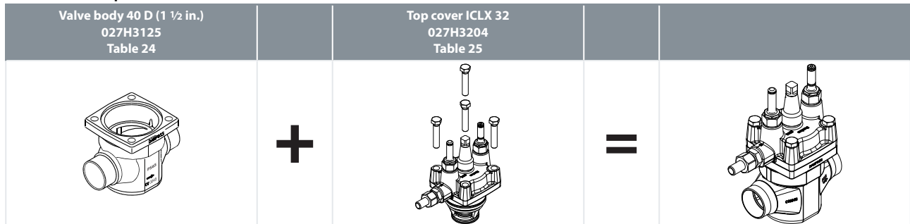
Figure 15: ICV 32
