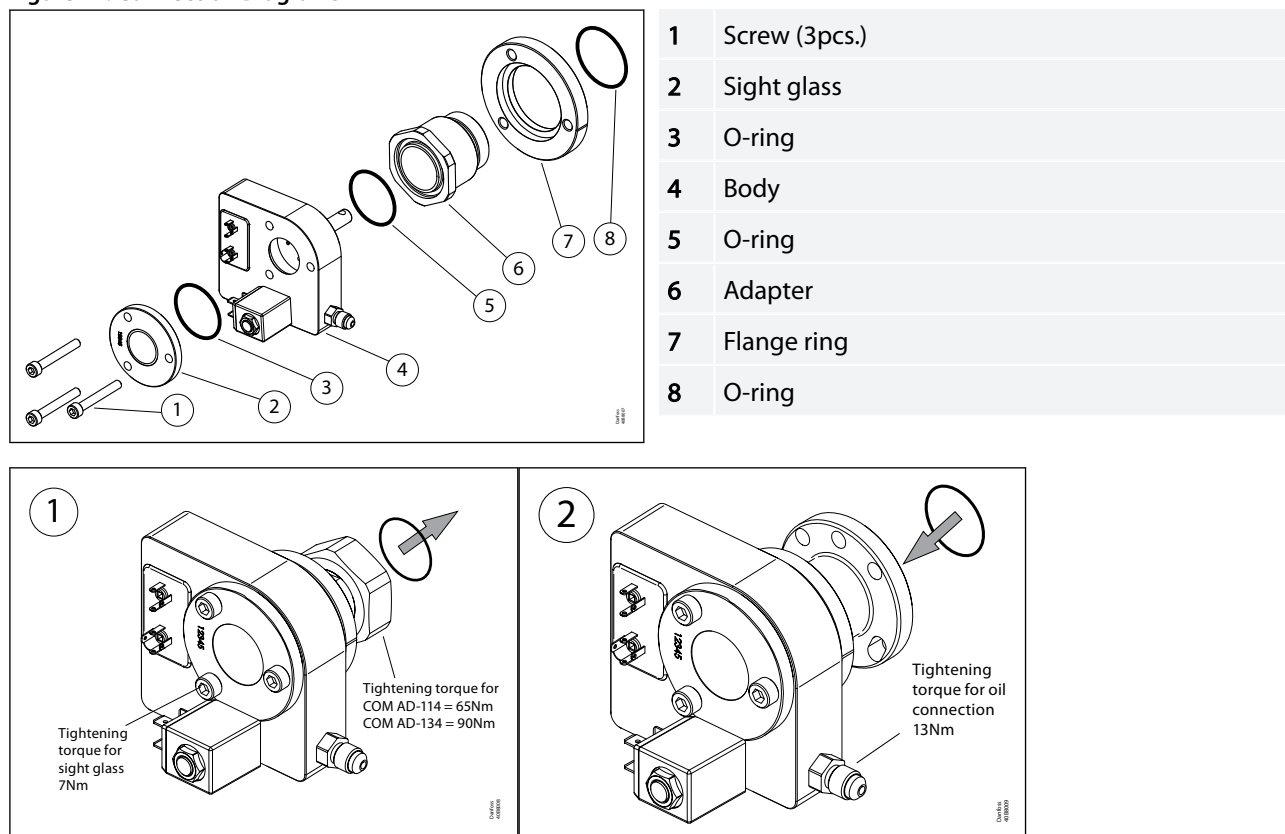
Figure 14: Connection Diagrams
