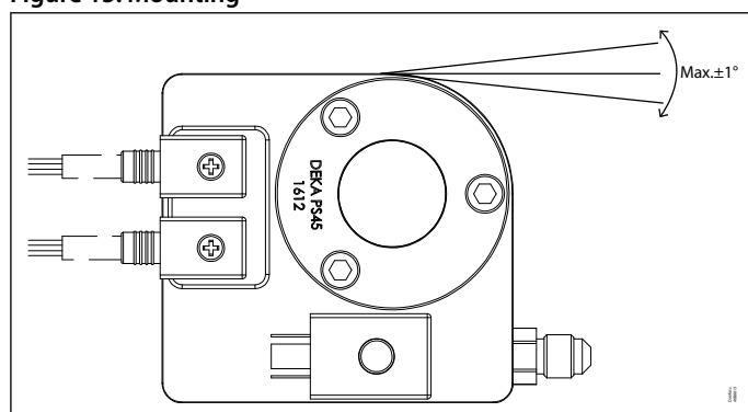
Figure 15: Mounting
