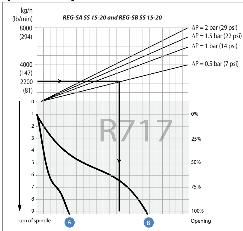
Figure 13: Flow rate diagram
