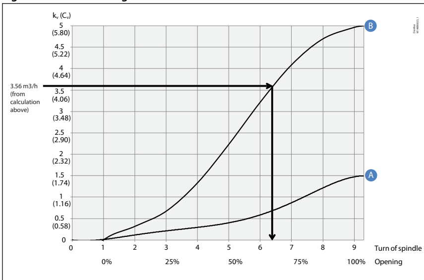
Figure 15: Flow rate diagram
