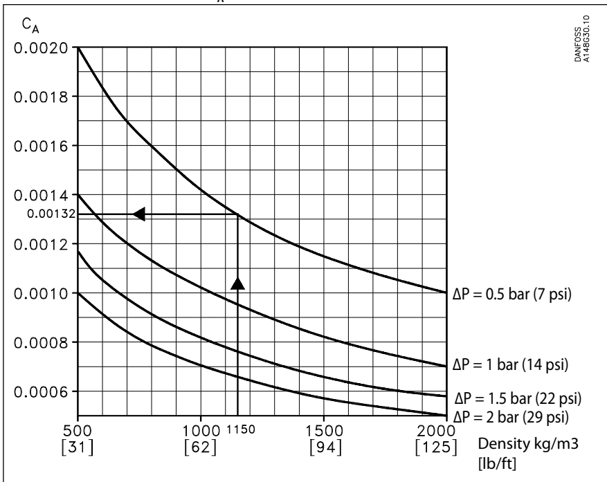
Figure 15: Flow rate diagram
