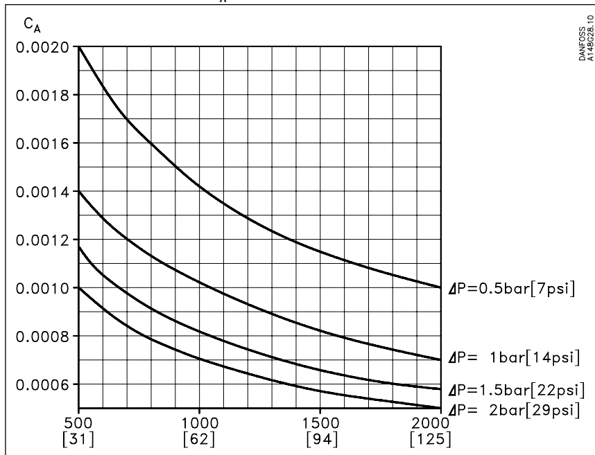
Figure 12: Calculation factor C_A
