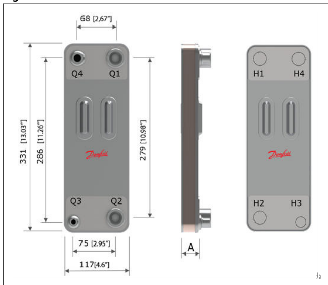
Figure 2: Dimensions
