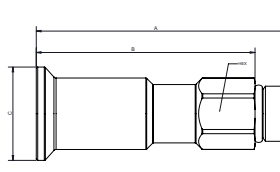
Figure 2 Socket
