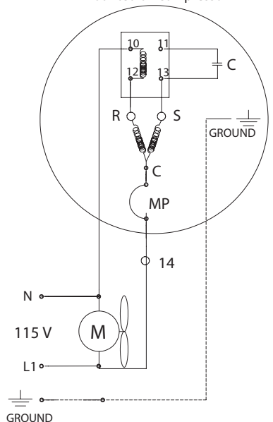
Mounted on compressor
