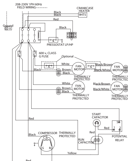
USE COPPER CONDUCTORS ONLY POWER SUPPLY THRU FUSED DISCONNECT
