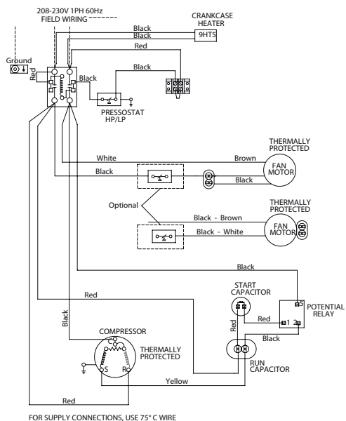
USE COPPER CONDUCTORS ONLY POWER SUPPLY THRU FUSED DISCONNECT
