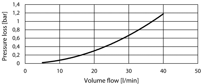
Picture 1 Pressure loss vs coolant flow
