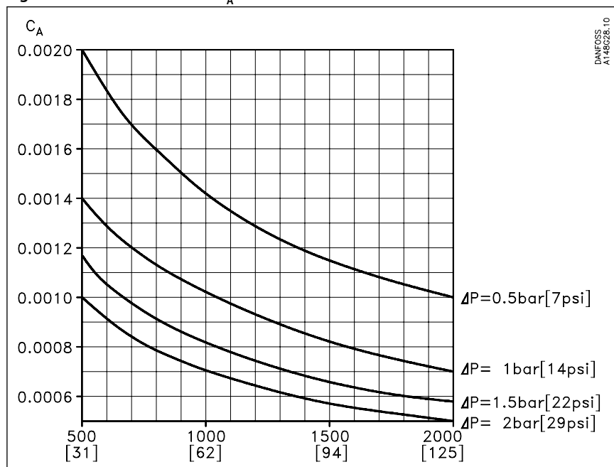
Figure 12: Calculation factor C_A
