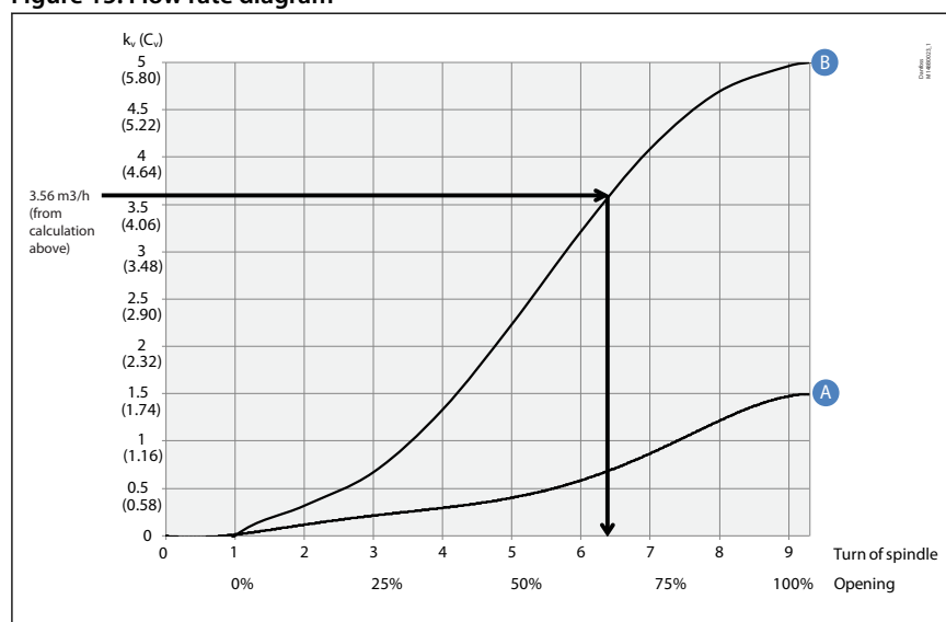
Figure 15: Flow rate diagram
