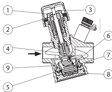
AB-QM DN 15-32
