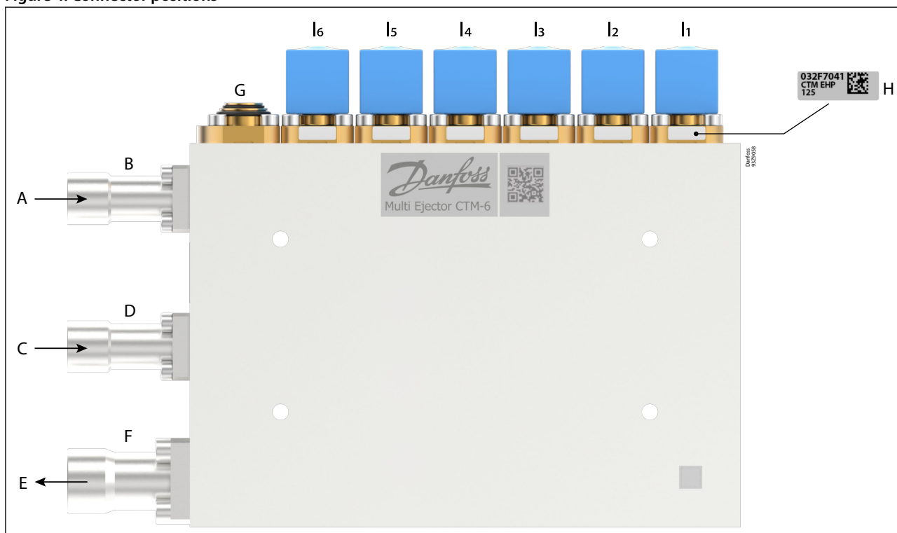
Figure 4: Connector positions
