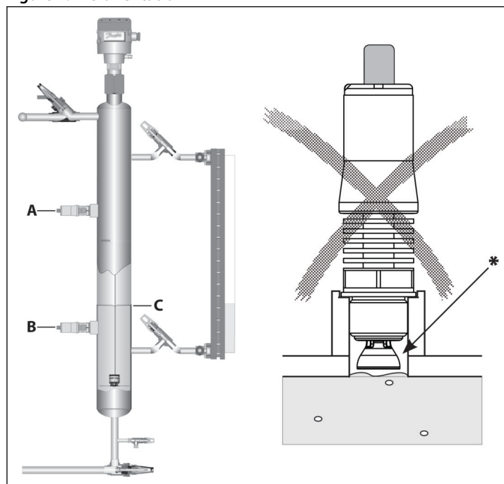
Figure 2: LLS orientation
