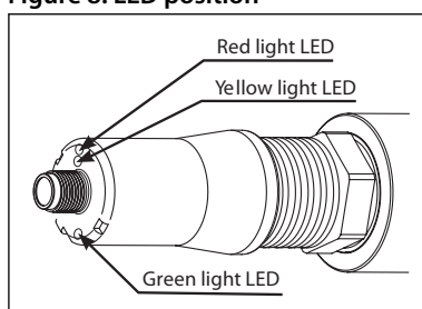
Figure 8: LED position
