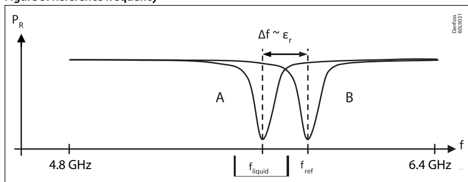
Figure 3: Reference frequency
