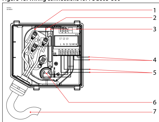
Figure 13: Wiring connections for PSG605-800
