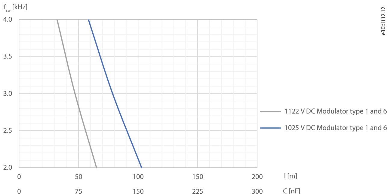
Figure 106: Safe Operation Area: 416 A Common-mode Filter, Low Output Frequency Range, 100% Flow
