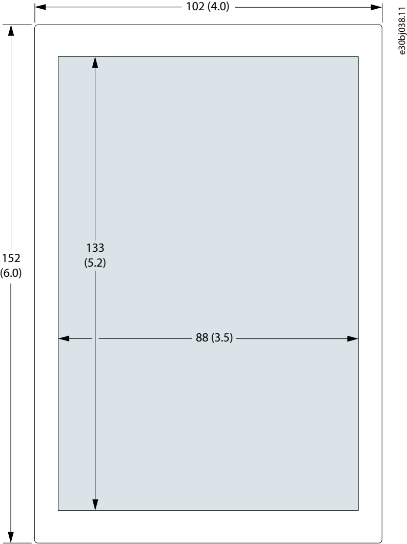
Figure 184: Flush Mounting Kit Drilling Template, mm (in)
