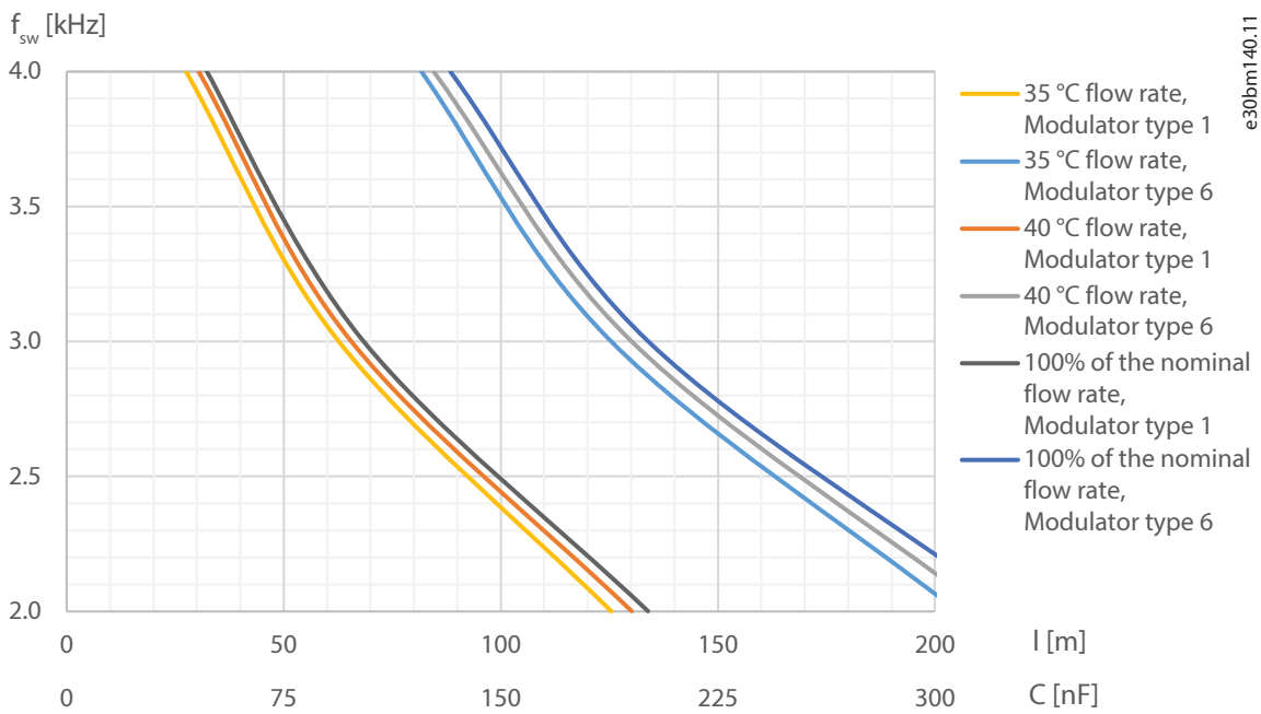
Figure 89: Safe Operation Area with Different Flow Rates: 416 A dU/dt Filter, 1025 V DC
