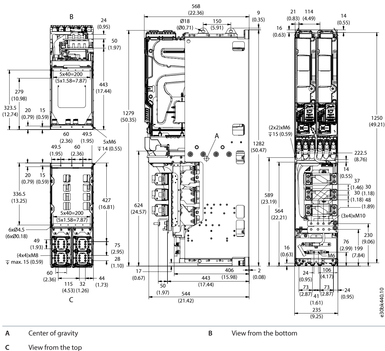
Figure 158: Dimensions of DC/DC Converter, DR12L, in mm (in)
