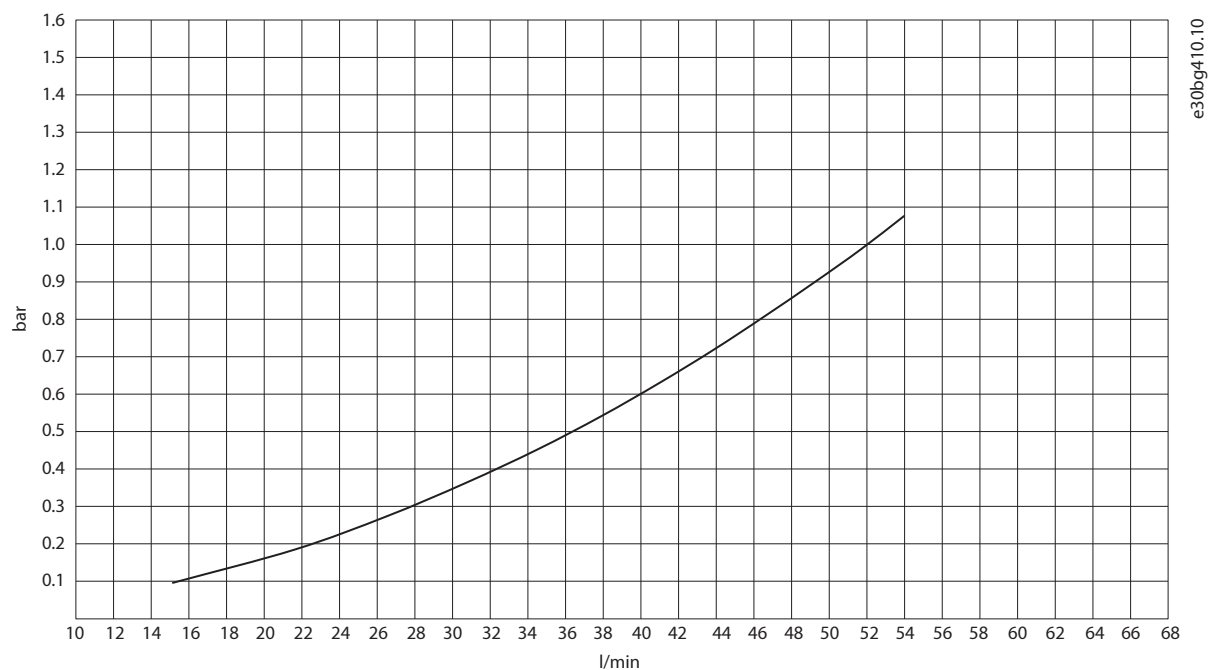
Figure 36: Unit Pressure Drop with Water, AFE AR12L and INU IR12L with Sine-wave Filter (+AES1)
