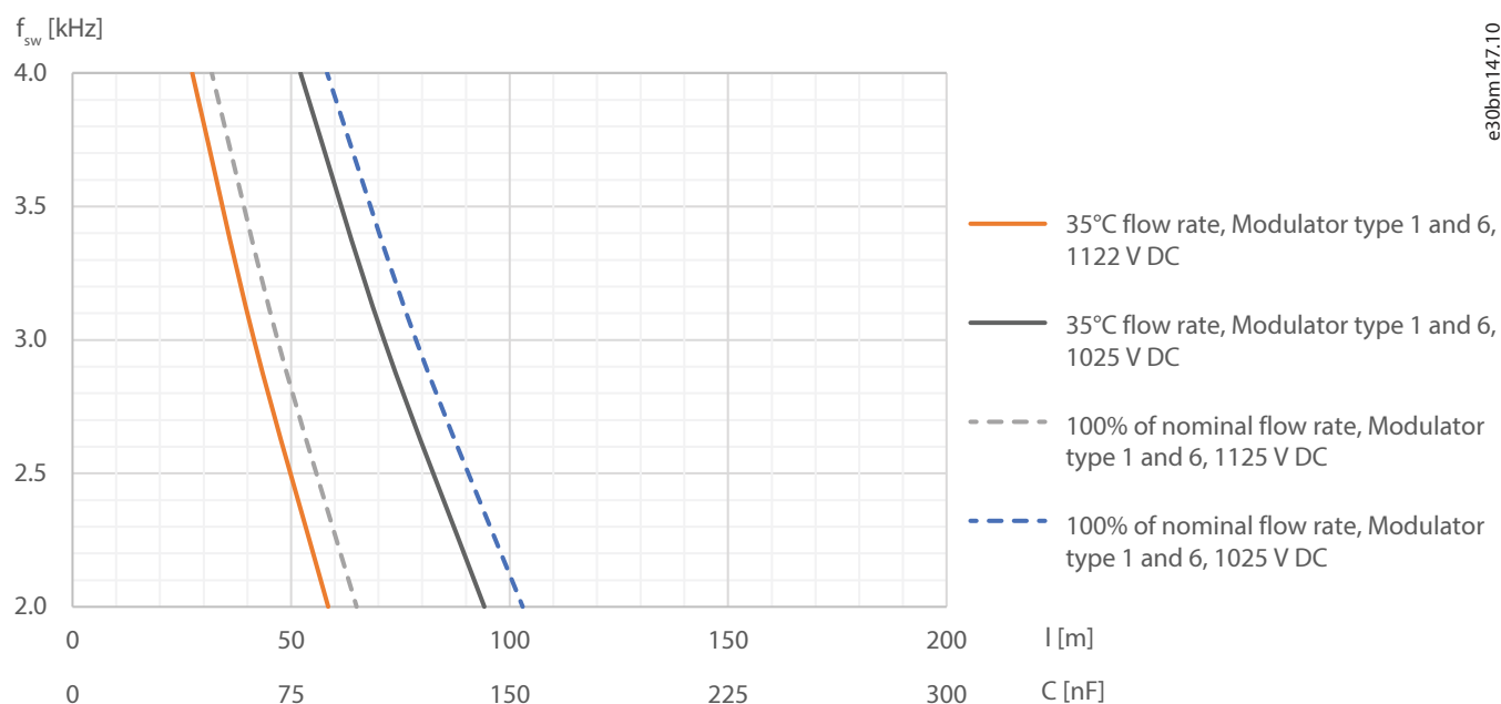
Figure 107: Safe Operation Area: 416 A Common-mode Filter, Low Output Frequency Range, with Different Flow Rates
