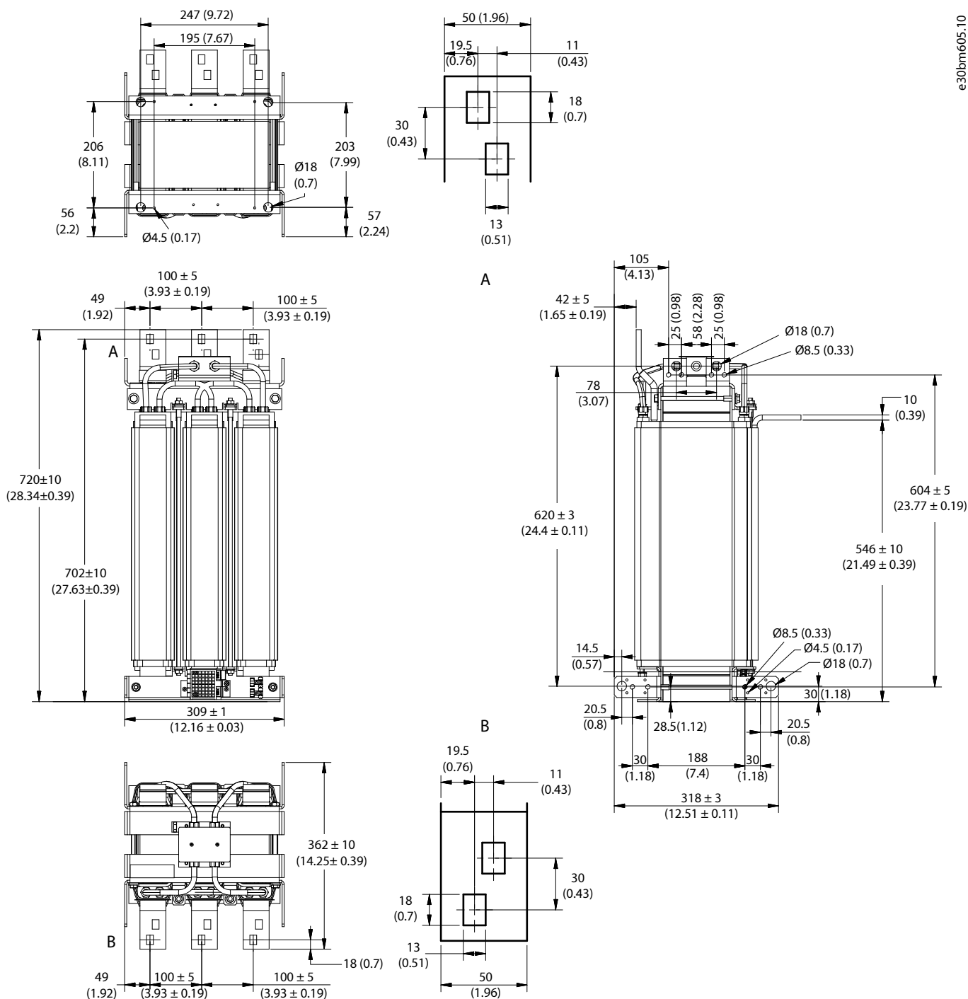
Figure 164: Dimensions of the L Filter, 2300 A
