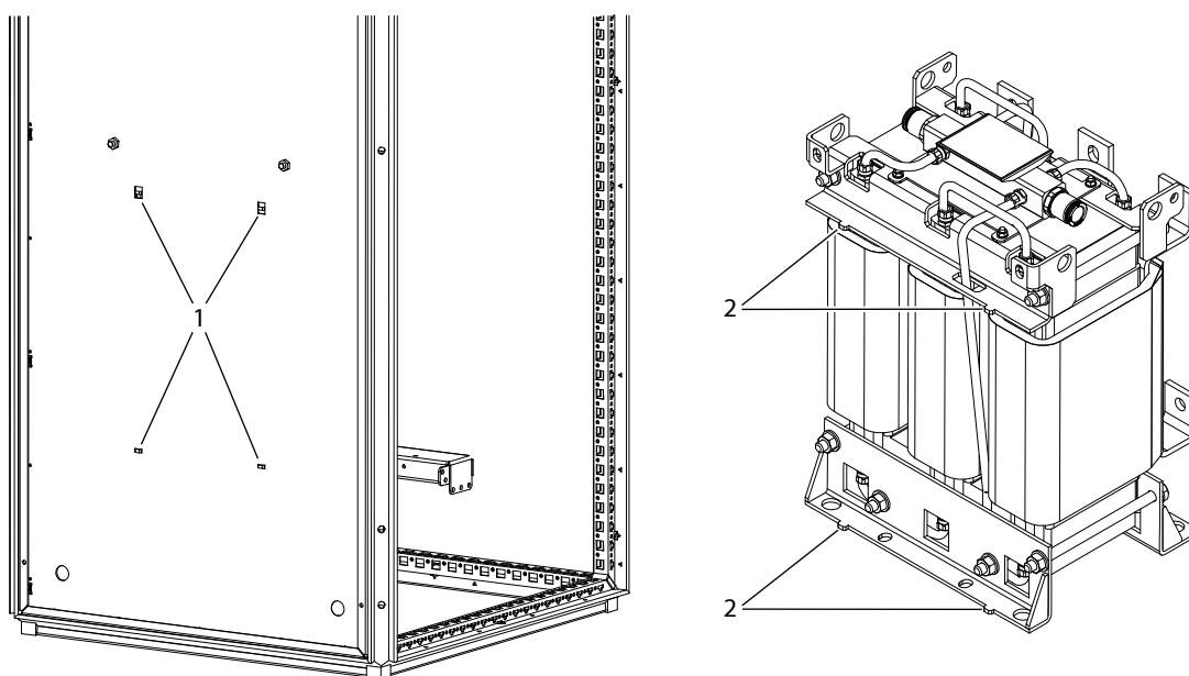
Figure 20: Aligning the Filter Pins with the Back Wall
