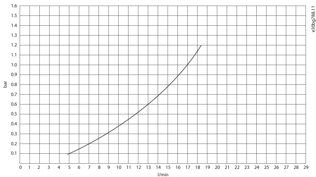
Figure 41: Pressure Drop with Water, Sine-wave Filter OF7S1SM (+AE51), 800 A
