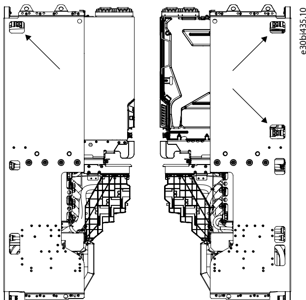
Figure 146: Cooling Connectors on the System Module
