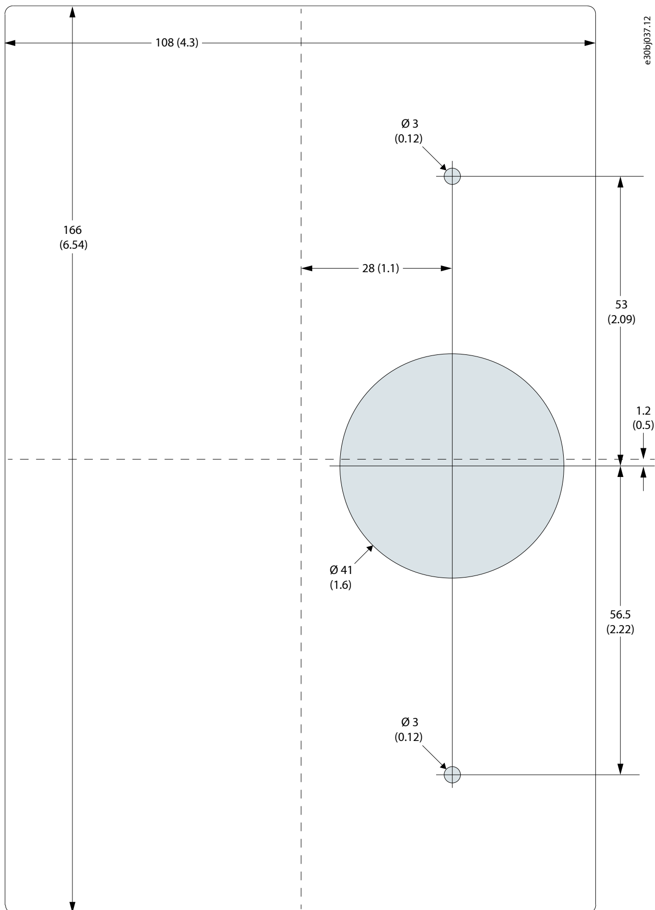
Figure 185: Surface Mounting Kit Drilling Template, mm (in)
