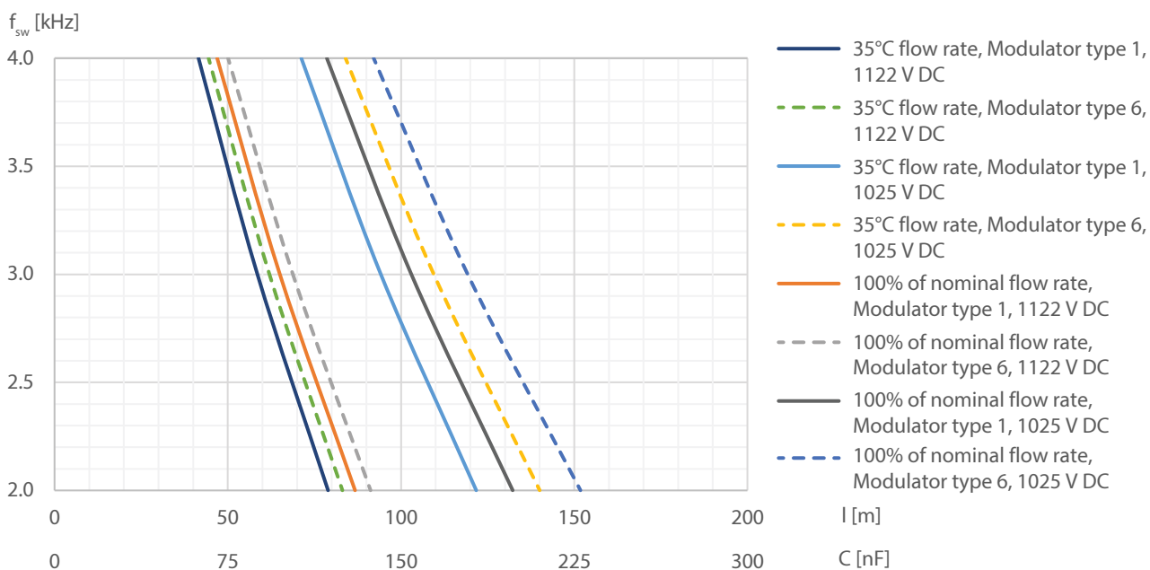
Figure 105: Safe Operation Area: 416 A Common-mode Filter, with Different Flow Rates
