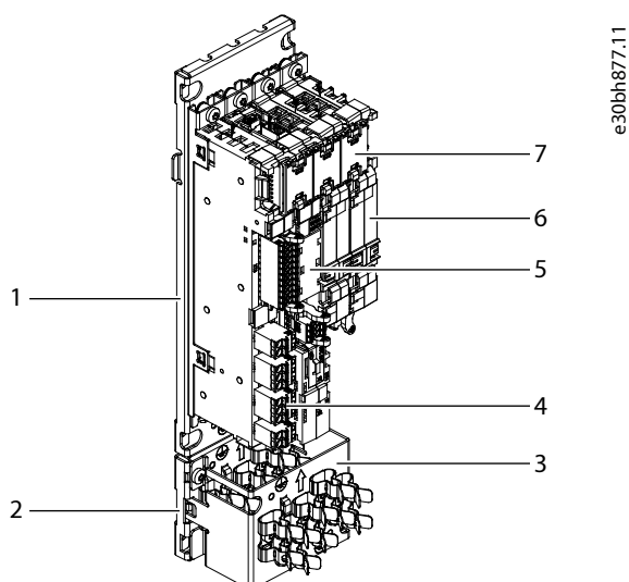
Figure 118: Example of the Modular Control Unit
