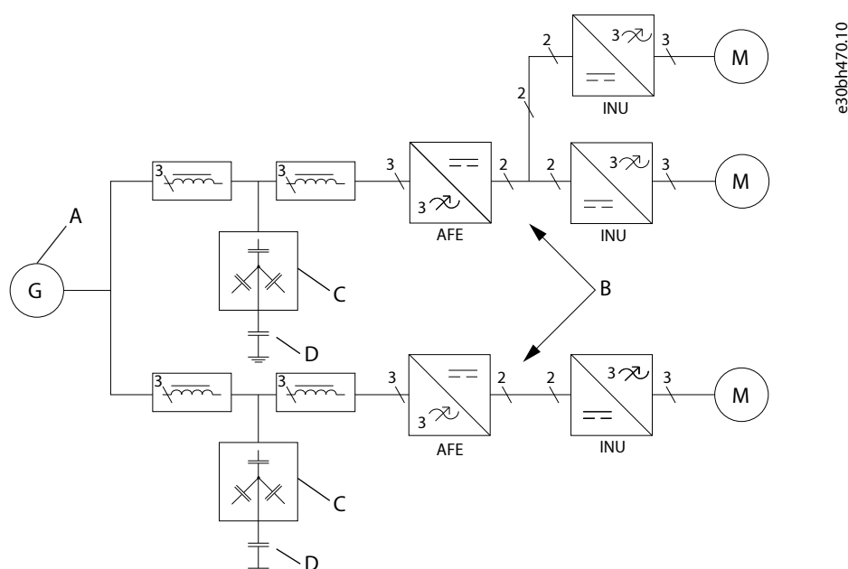
Figure 77: AFE Modules in IT System
