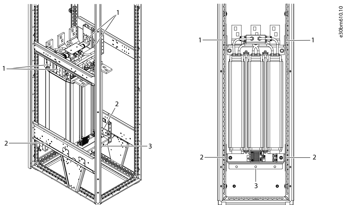
Figure 22: Installing the L Filter into a Cabinet (1640 A, 2300 A)
