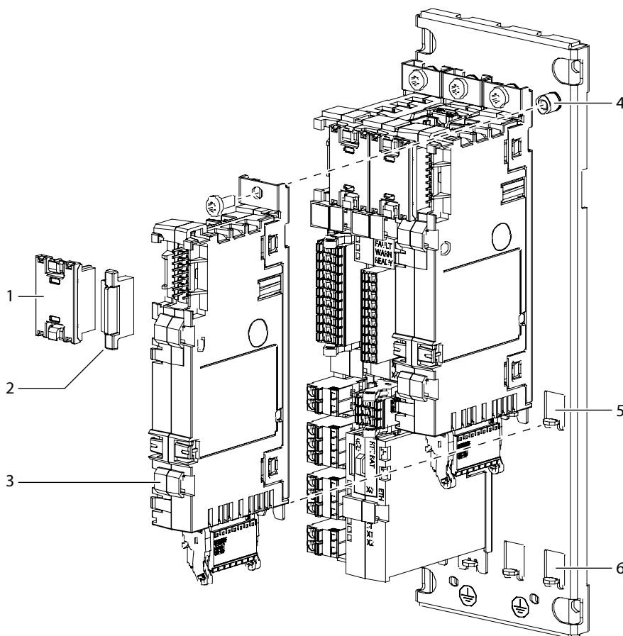
Figure 132: Installing a Board to the Modular Control Unit Mounting Plate
