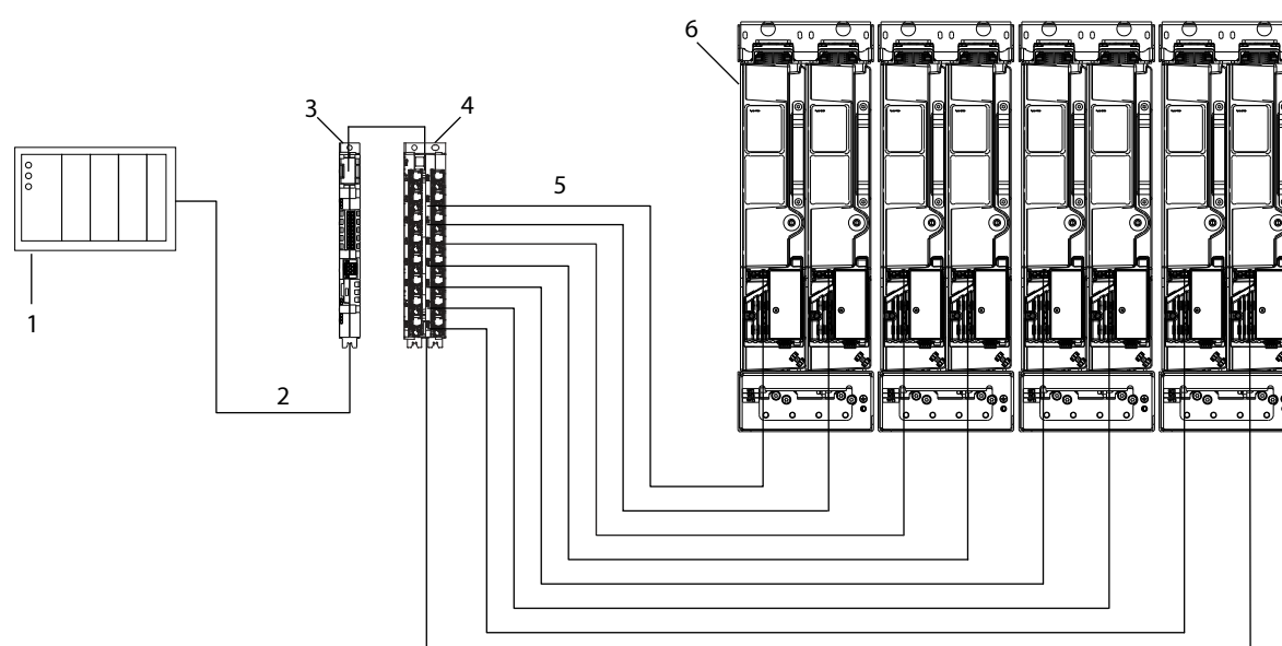
Figure 133: Connecting the Fieldbus Cable and the Fiber Cables
