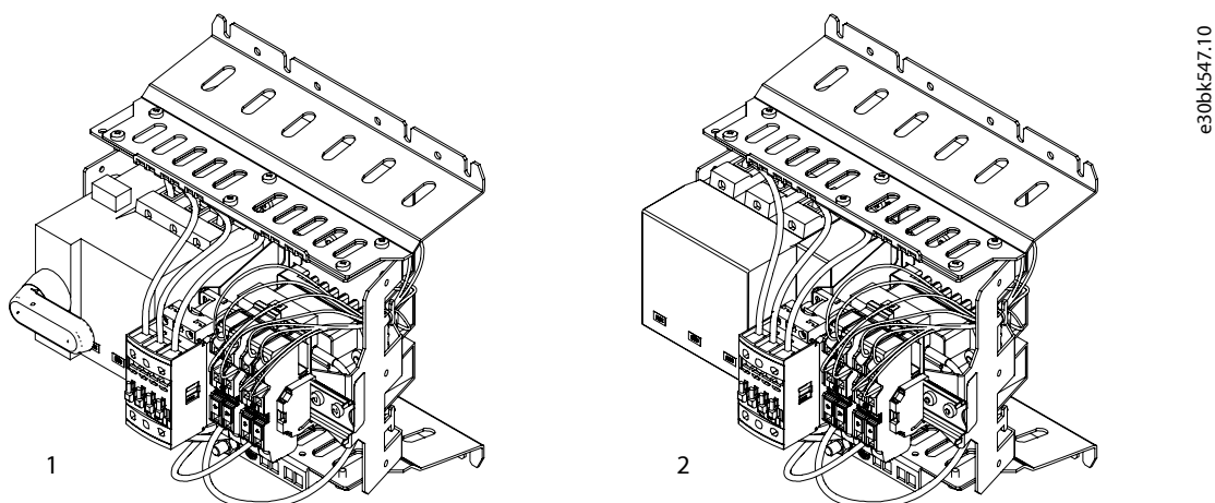
Figure 113: Pre-charging Units
