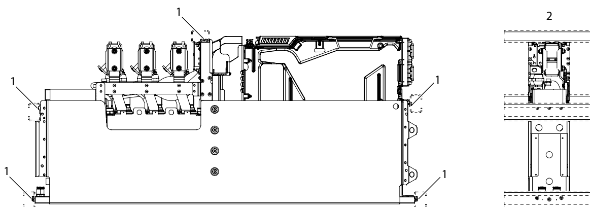
Figure 19: Mounting Holes of the System Module with the Integration Unit on its Backside
