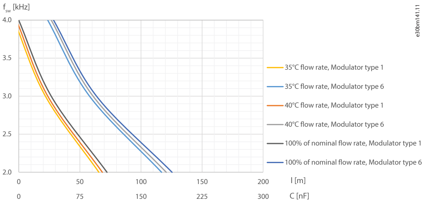
Figure 90: Safe Operation Area with Different Flow Rates: 416 A dU/dt Filter, 1122 V DC
