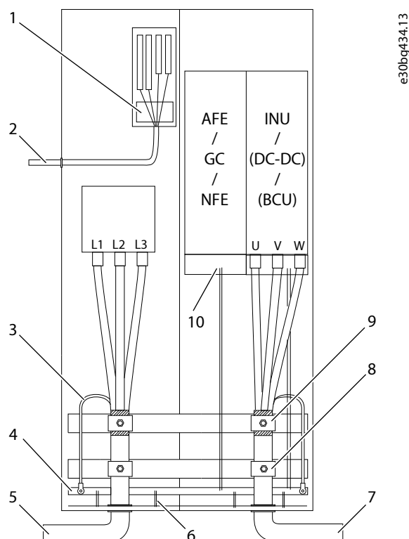
Figure 69: Cabling Principle
