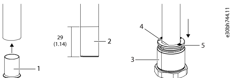
Figure 50: Inserting a Pipe into the Cooling Circuit Connector, mm (in)
