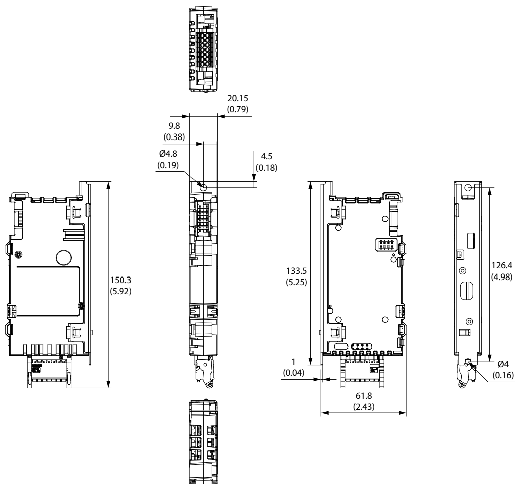
Figure 176: Dimensions of an Option Board in mm (in)
