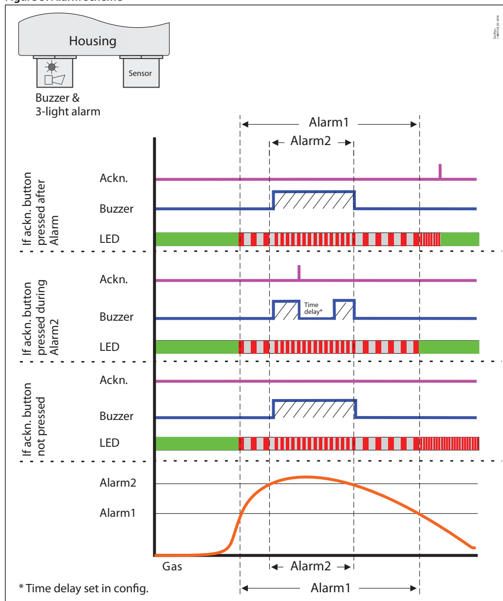
Figure 5: Alarm scheme
