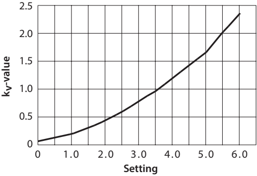
Flow characteristics
