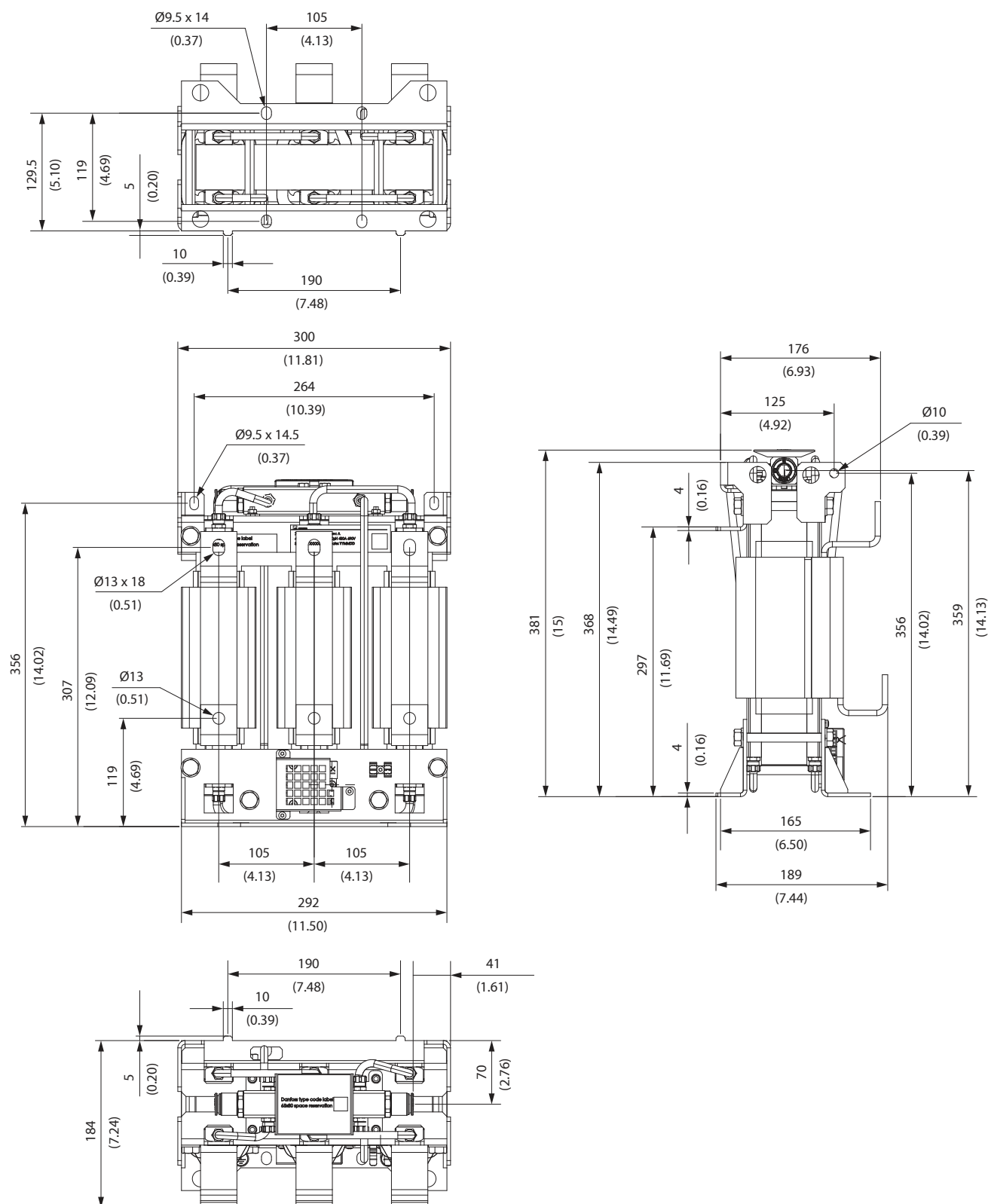
Figure 6: Dimensions of the L Filter, 400 A
