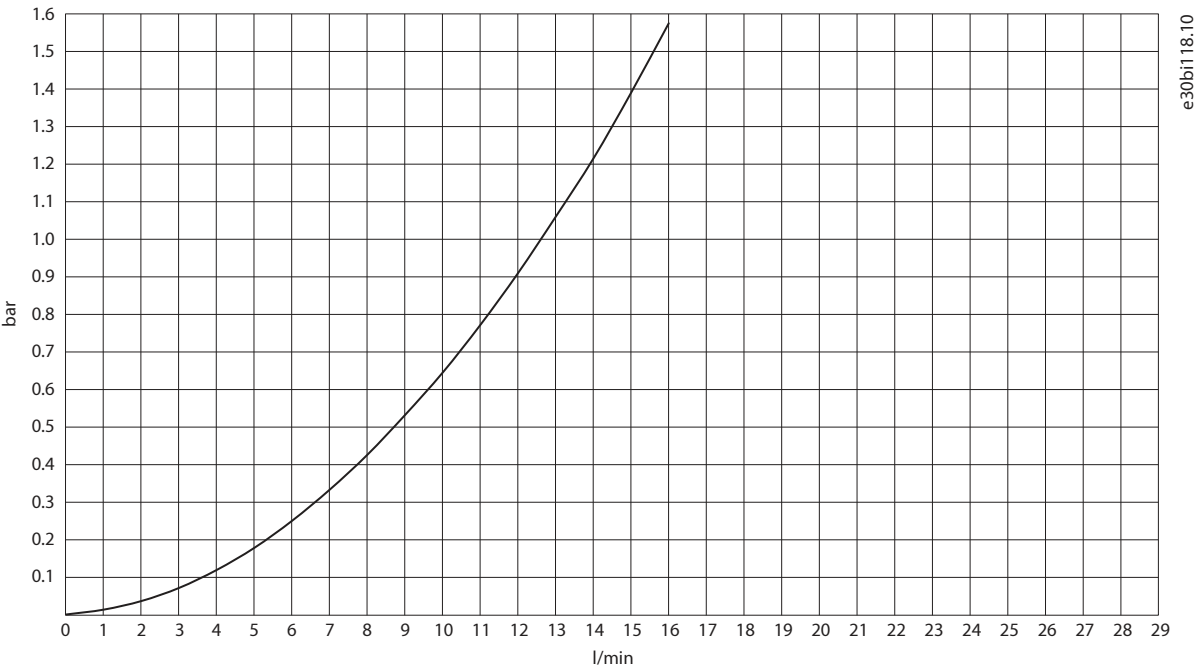
Figure 12: Pressure Drop, L Filter OF7Z5, 690 V/1640 A
