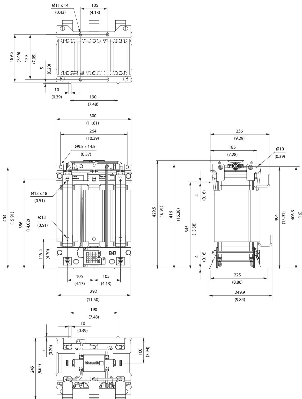
Figure 7: Dimensions of the L Filter, 1000 A
