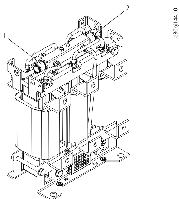
Figure 14: Inlet and Outlet Connectors of the L Filter
