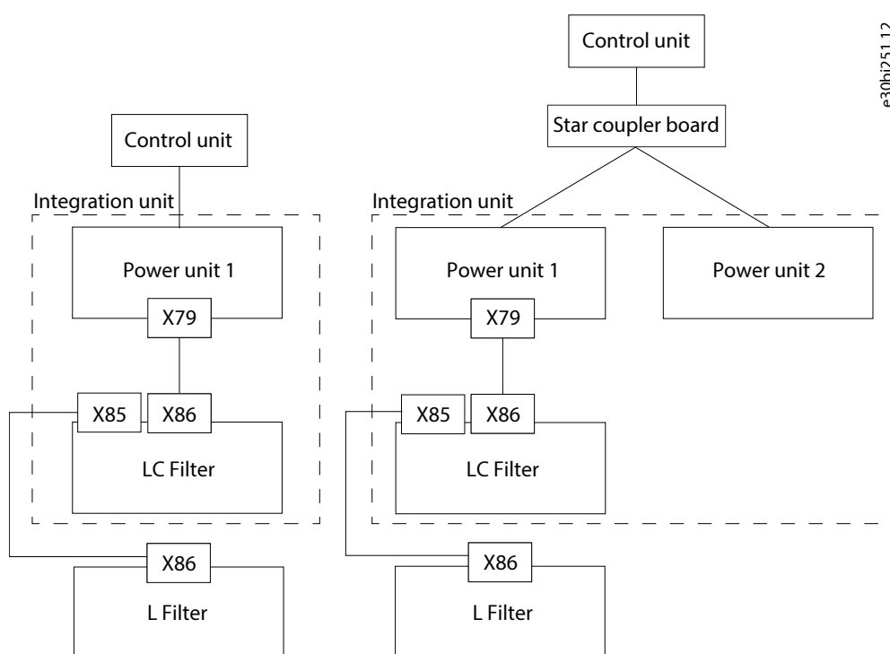
Figure 18: AuxBus Topology for AFE and Grid Converter Modules AR10L and AR12L
