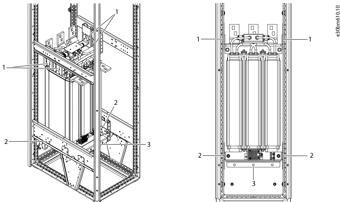
Figure 5: Installing the L Filter into a Cabinet (1640 A, 2300 A)
