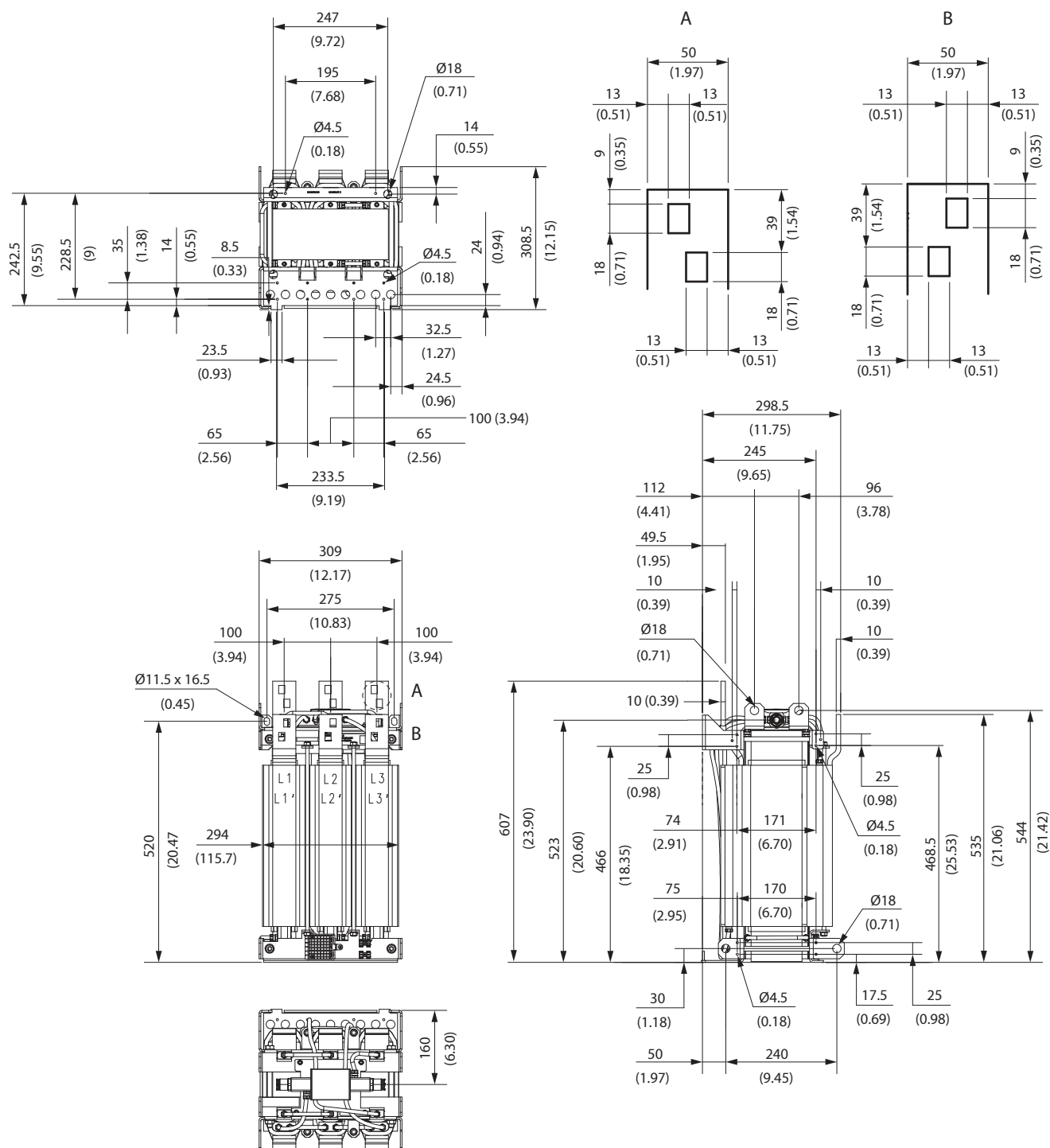
Figure 8: Dimensions of the L Filter, 1640 A
