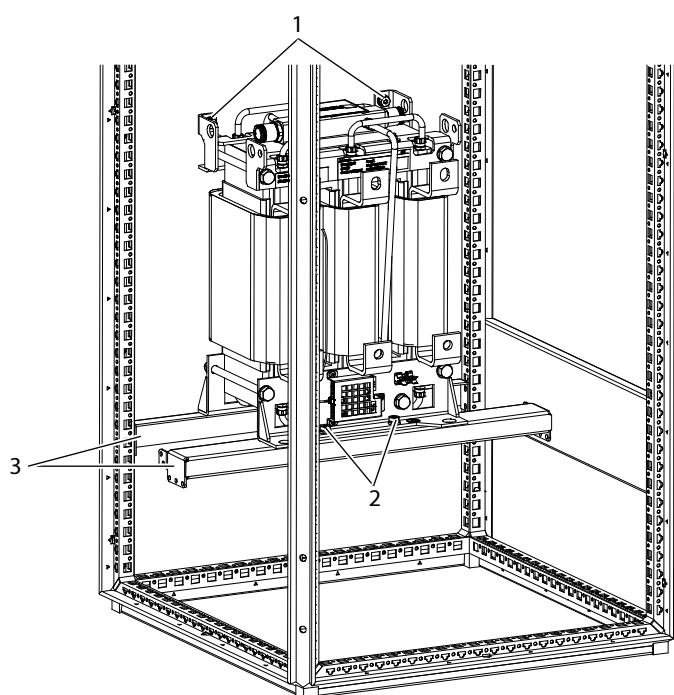
Figure 4: Installing the L Filter into a Cabinet (400 A, 1000 A)
