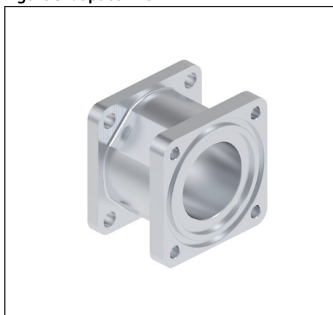
Figure 31: Spacer kit
