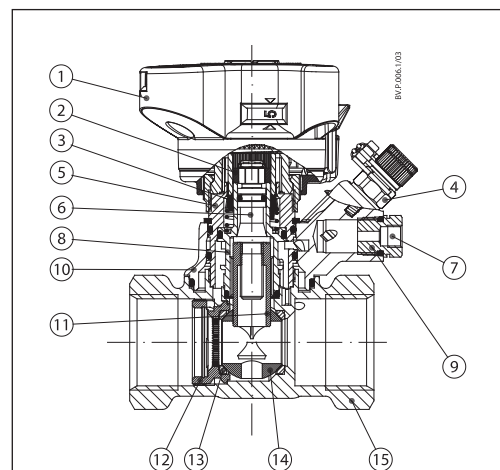
Obr. 7 ASV–BD DN 15–50
