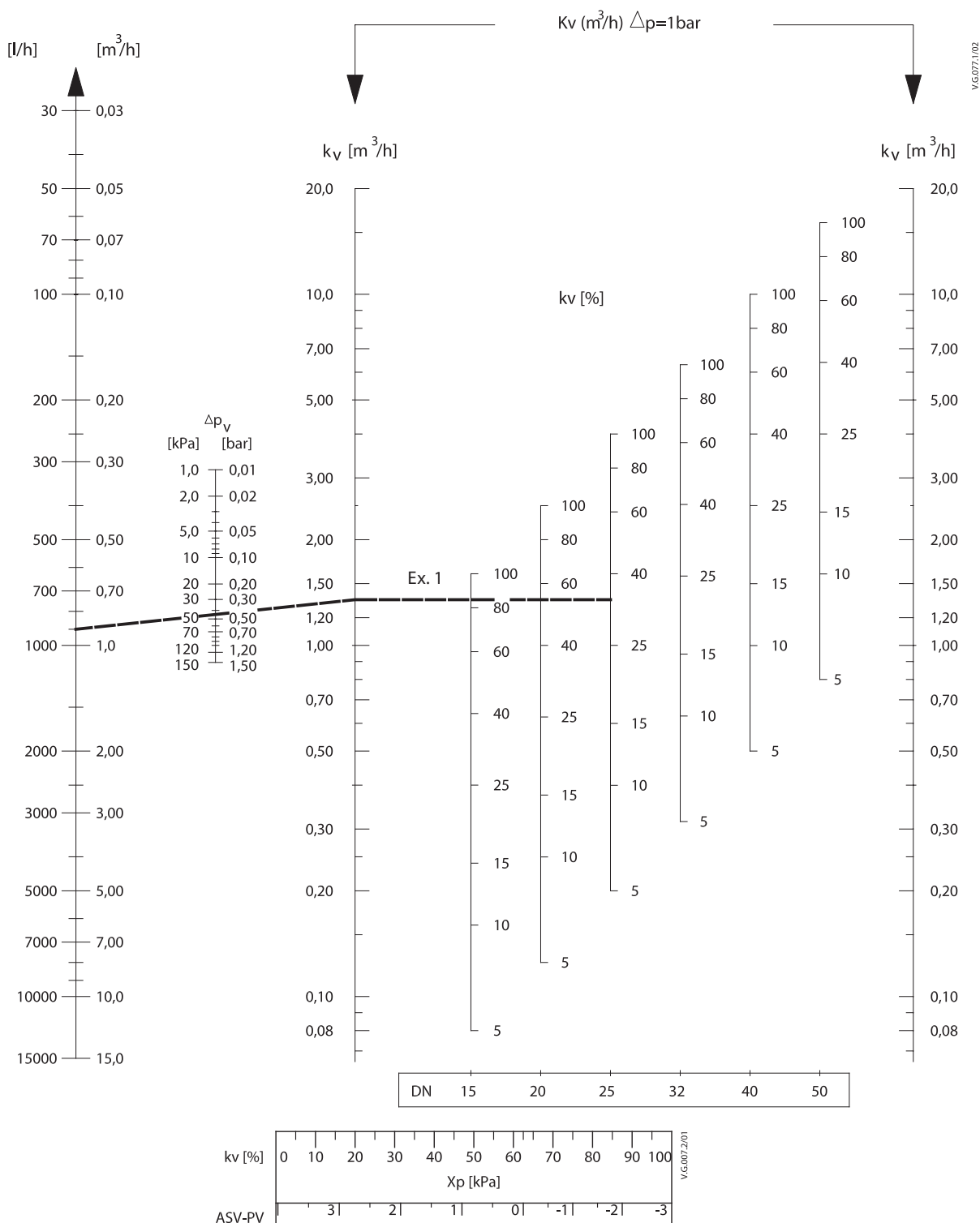
Fig. A – Diagrama de dimensionare ASV–PV DN 15 – 50
