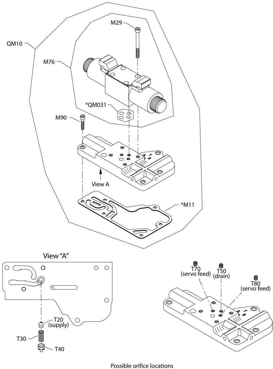
Possible orifice locations
