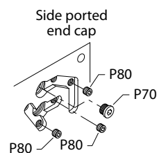
View "A" with pressure limiter port A only, CW rotation
