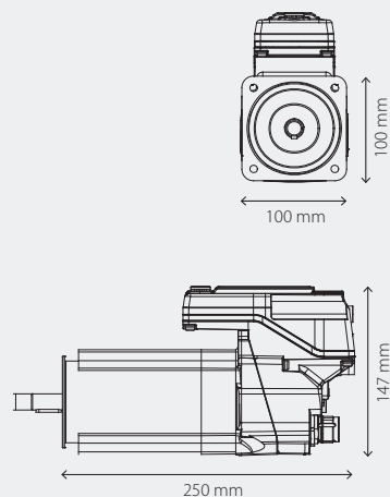
Example frame size 3 (-05T0+FN30) ISD 520
