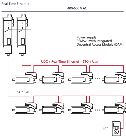
Example of system topology using ISD 520
