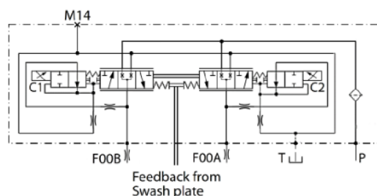
NFPE schematic
