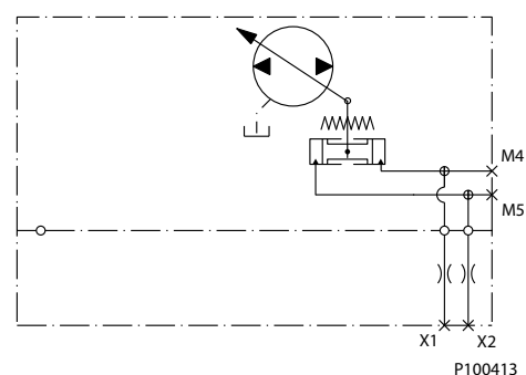
Non-feedback proportional hydraulic control schematic
