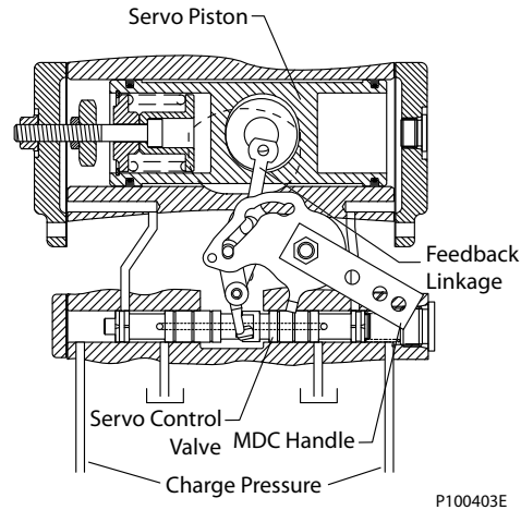
Cross-section of MDC
