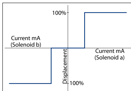
Pump displacement to Electrical signal
