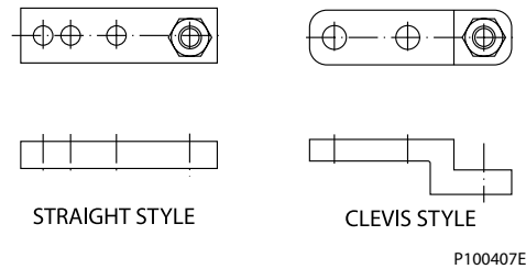
MDC Handle Options
