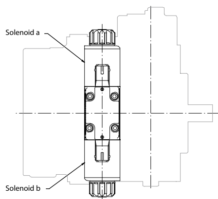
FNR on Series 42 (for 41/51cc)
