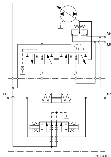
Pump Flow Direction with EDC
