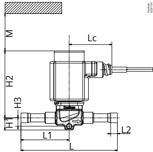
Figure: EVRC and Cable coil
