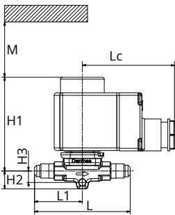
Figure: EVR and Terminal box coil
