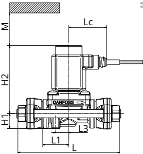
Figure: EVR and Cable coil
