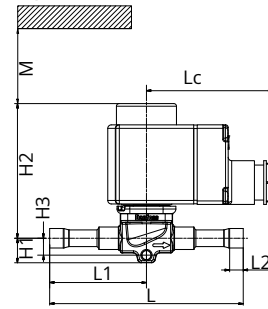
Figure: EVR and Terminal box coil
