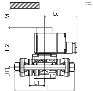
Figure: EVR and Terminal box coil
