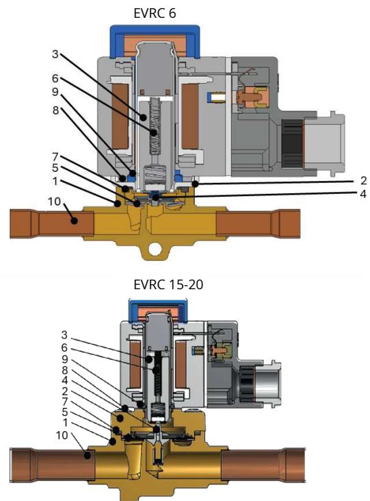
Figure: EVRC 6, 15 and 20 Solder connection
