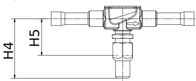
Figure: Manual stem
