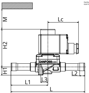
Figure: EVR and Terminal box coil
