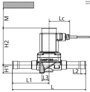
Figure: EVR and Cable coil
