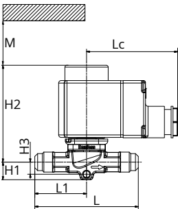
Figure: EVR and Terminal box coil
