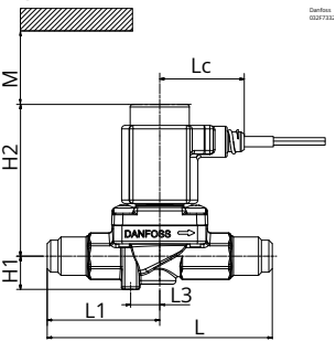
Figure: EVR and Cable coil
