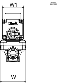
Figure: End view
