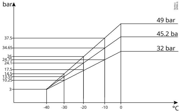
Figure: Max. working pressure in bar in relation to media temperature in °C.
