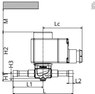
Figure: EVRC and Terminal box coil
