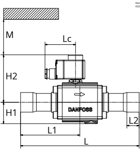
Figure: EVR and Terminal box coil
