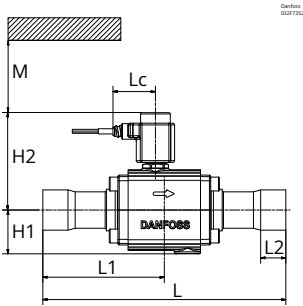
Figure: EVR and Cable coil
