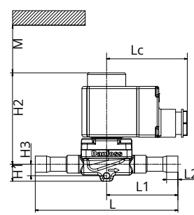
Figure: EVR and Terminal box coil
