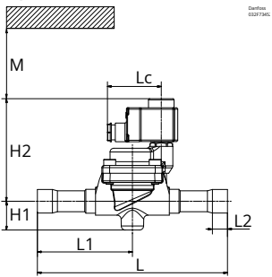
Figure: EVR and Terminal box coil
