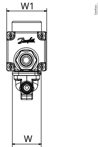
Figure: End view
