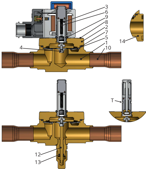
Figure: EVR 20 - EVR 22 Solder and flange connection
