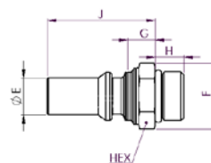
Figure 4 Male ORB ISO 11926-3
