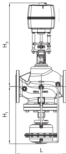
AMV(E) 65X/AFQM 2 DN 65-250, PN 16/25/40
