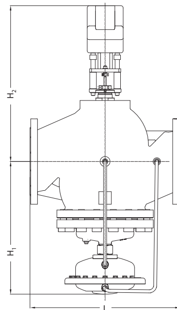
AFQM, DN150-250, PN16 + AMV(E)85,86
