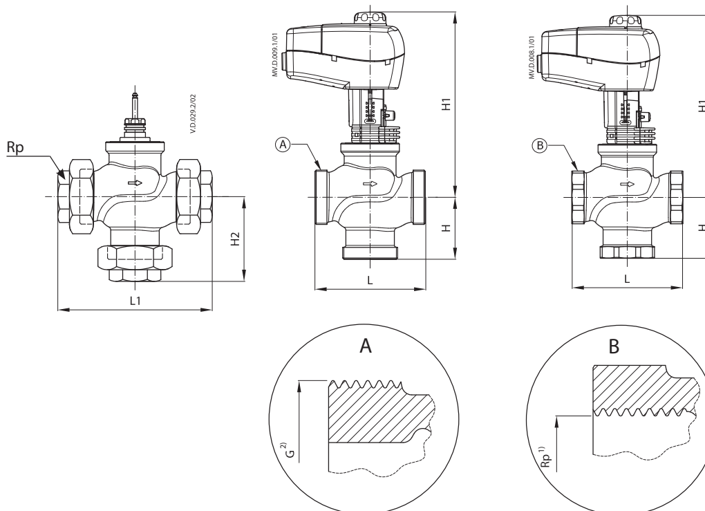
VRB3
