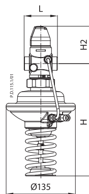
AVPQ DN 15-50 \Delta p_s = 0,3-2,0 бар
