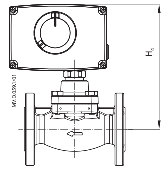
VB2 + AMV(E) 20/30, 23/33
