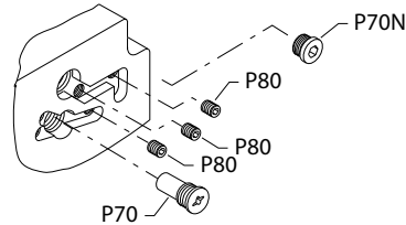
View "A" of end cap with pressure limiter port B, CW pump rotation.
