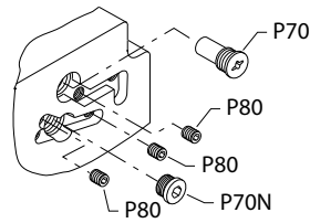
View "A" of end cap with pressure limiter port B, CCW pump rotation.
