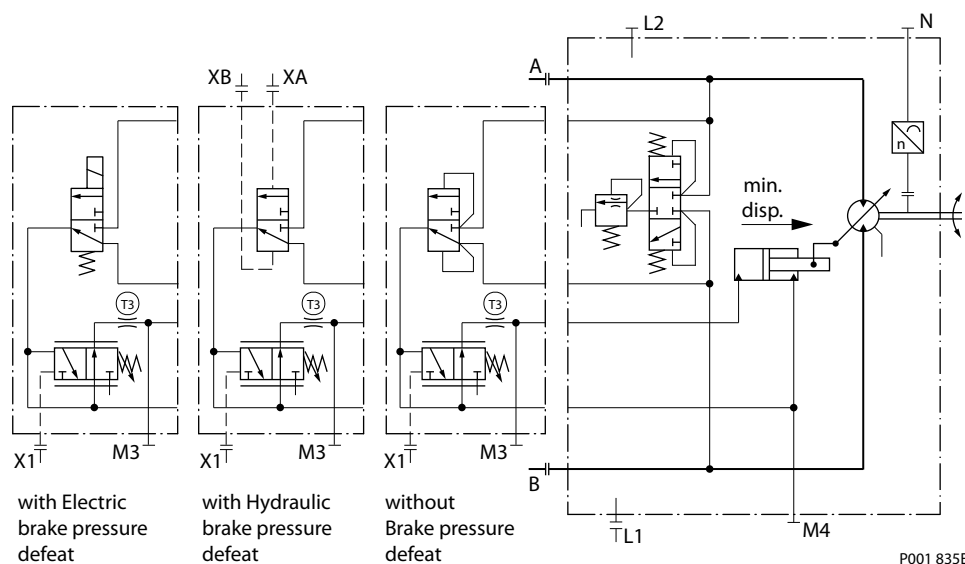
Circuit diagram – motor with two-position control TH**
