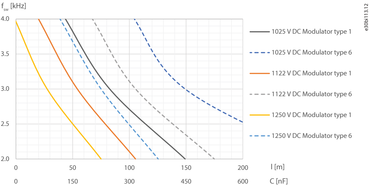
Figure 96: Safe Operation Area: 820 A dU/dt Filter, 100% Flow
