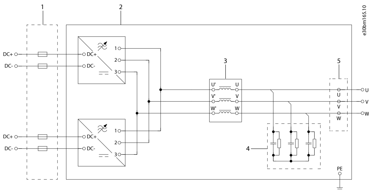
Figure 190: Wiring Diagram, INU IR12L with Sine-wave Filter
