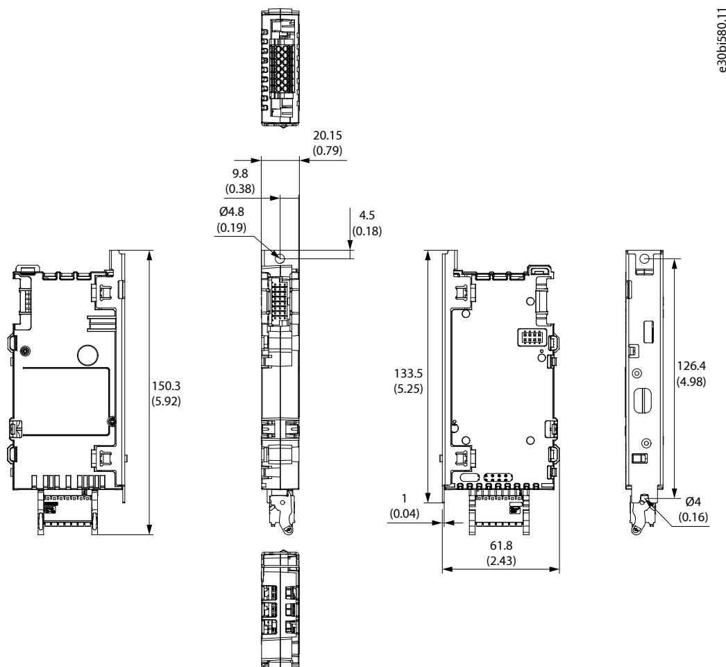
Figure 176: Dimensions of an Option Board in mm (in)
