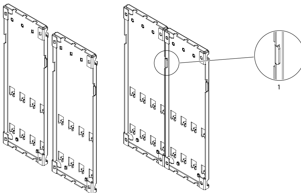
Figure 131: Attaching Mounting Plates to Each Other
