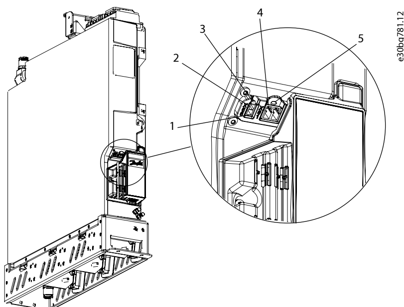
Figure 76: Auxiliary Power Connection for the Power Unit
