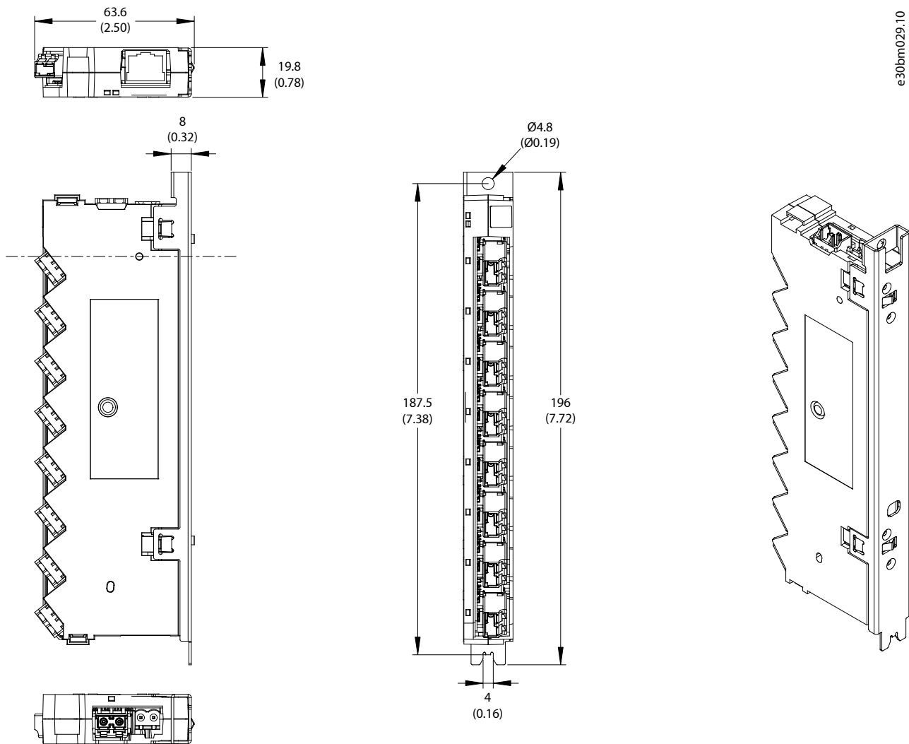
Figure 178: Dimensions of the 8-port Star Coupler Board in mm (in)
