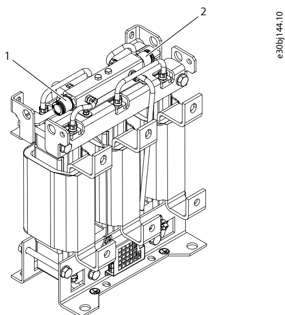
Figure 149: Inlet and Outlet Connectors of the L Filter
