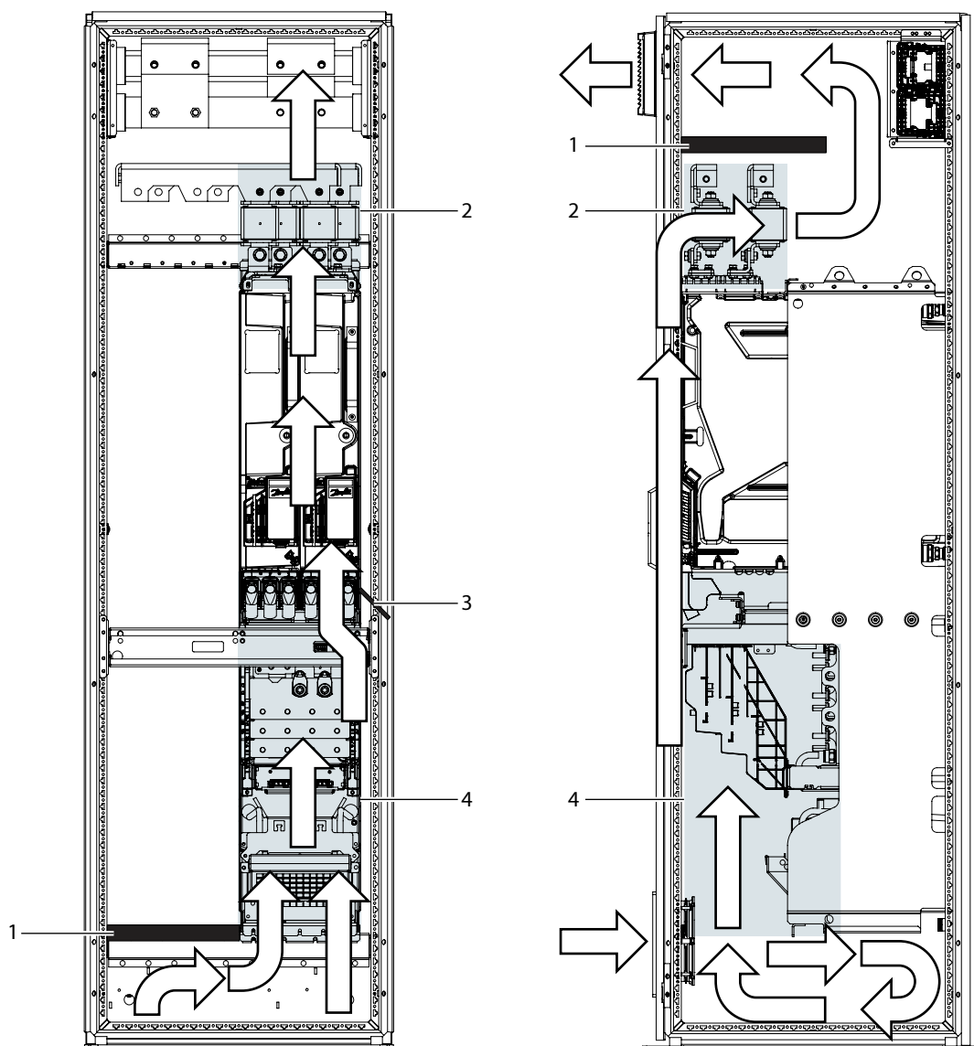
Figure 59: Example of Air Circulation Inside an Enclosure
