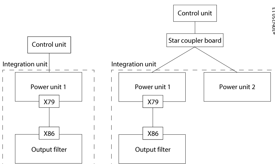
Figure 109: AuxBus Topology for Inverter Modules IR10L and IR12L
