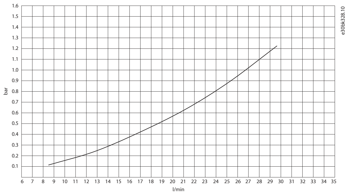
Figure 46: Unit Pressure Drop with Water, DC/DC Converter DR10L with DC Filter (+AED1)
