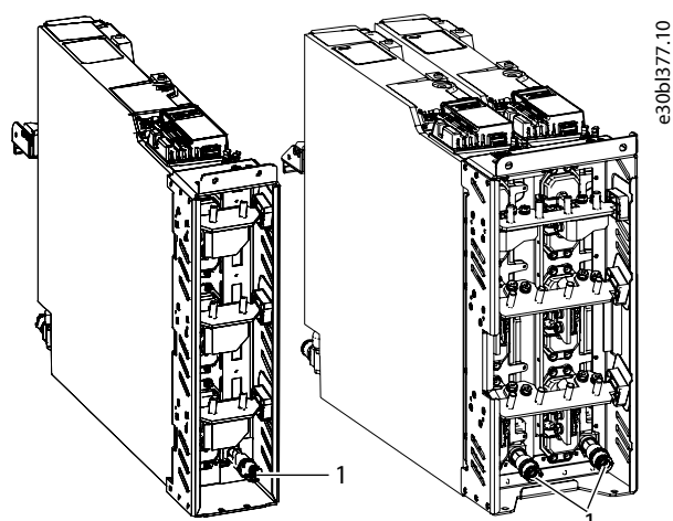
Figure 51: Inlet Connectors of IM10L (left) and IM12L (right)
