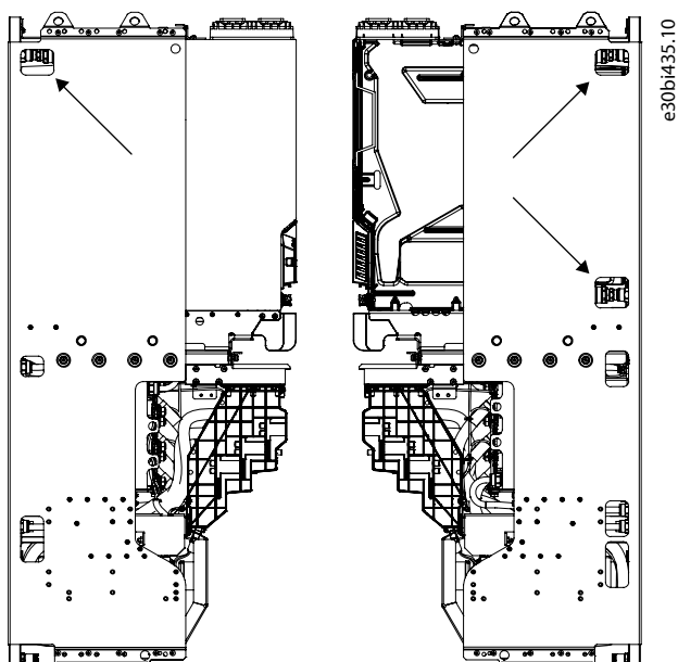
Figure 146: Cooling Connectors on the System Module
