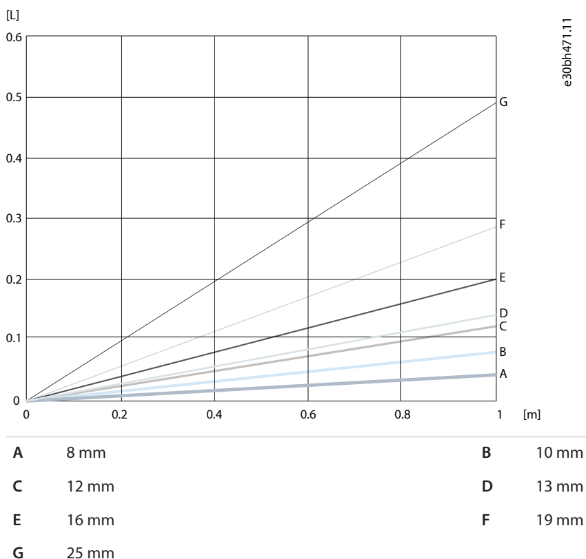
Figure 26: Volume of the Pipe with Different Inside Diameters, 8–25 mm
