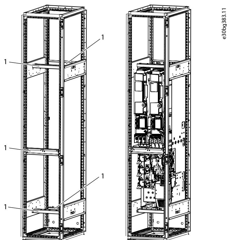
Figure 17: The Mounting Brackets and the Installation of System Modules with the Integration Unit into the Cabinet
