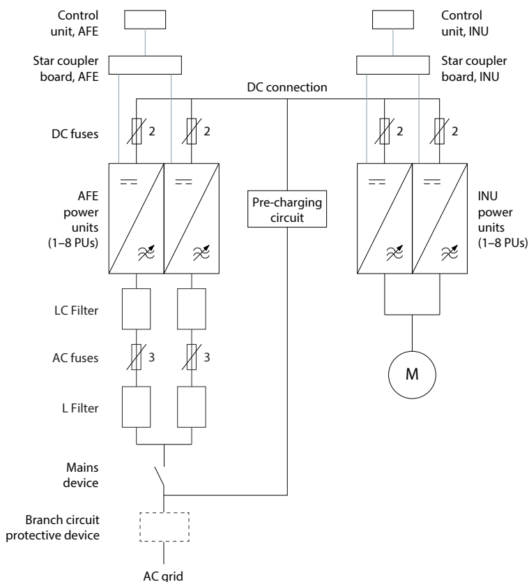
Figure 61: DC Connections of Parallel Power Units
