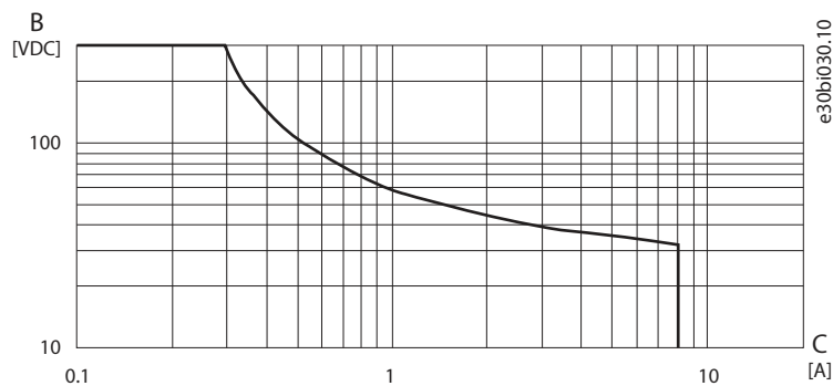
Figure 129: Maximum DC Load Breaking Capacity
