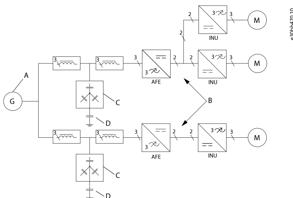
Figure 77: AFE Modules in IT System
