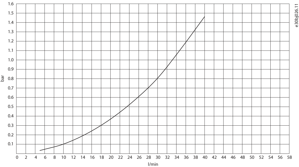
Figure 29: Unit Pressure Drop with Water, IM12L/AM12L/DM12L
