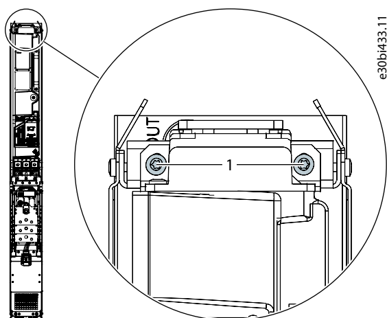
Figure 143: System Module Mounting Screws
