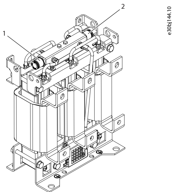
Figure 55: Inlet and Outlet Connectors of the L Filter
