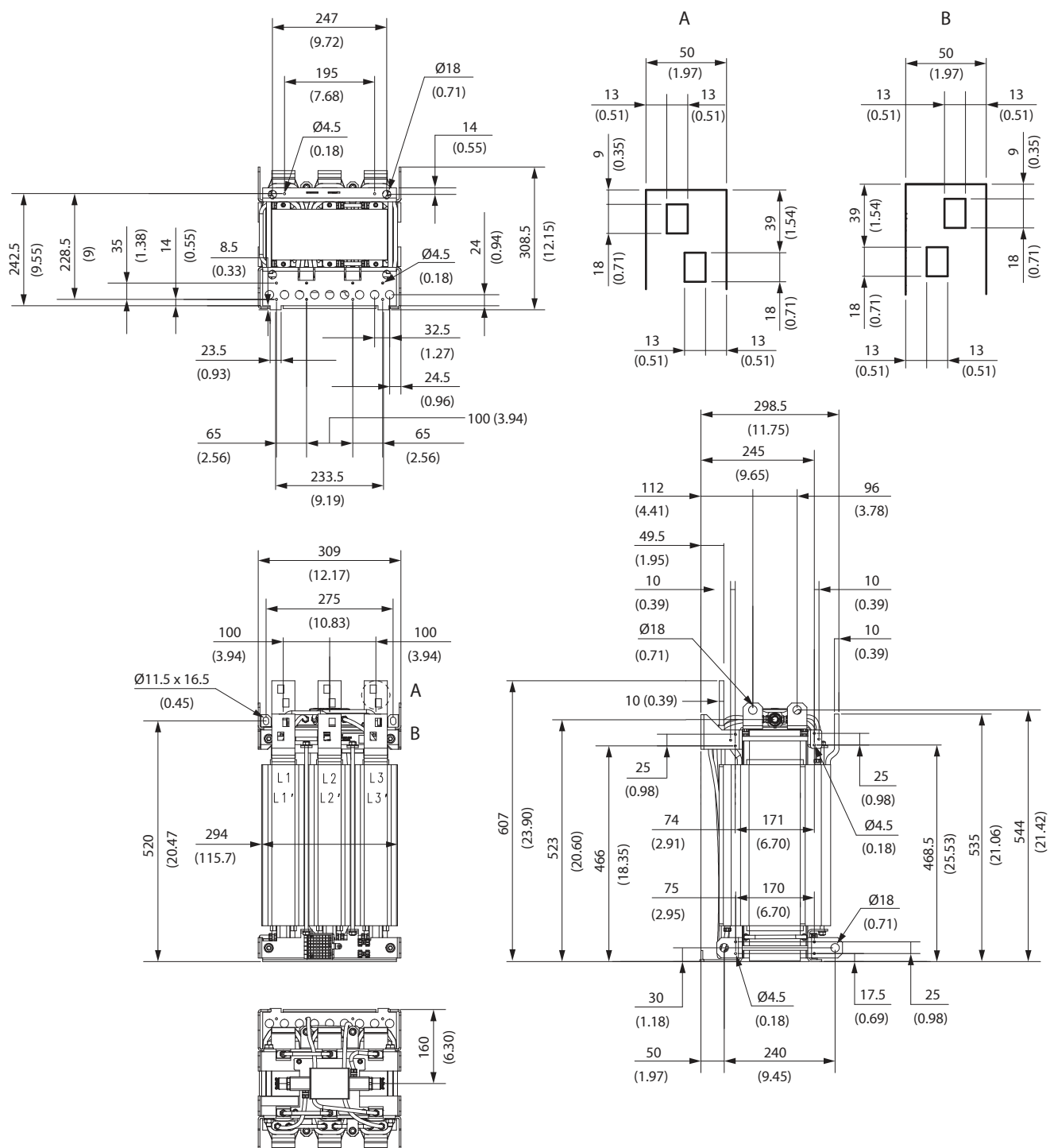
Figure 163: Dimensions of the L Filter, 1640 A
