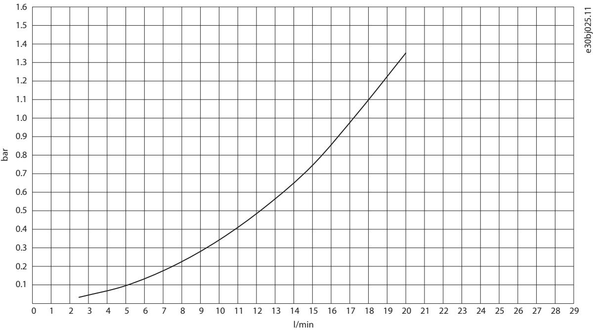
Figure 28: Unit Pressure Drop with Water, IM10L/AM10L/DM10L
