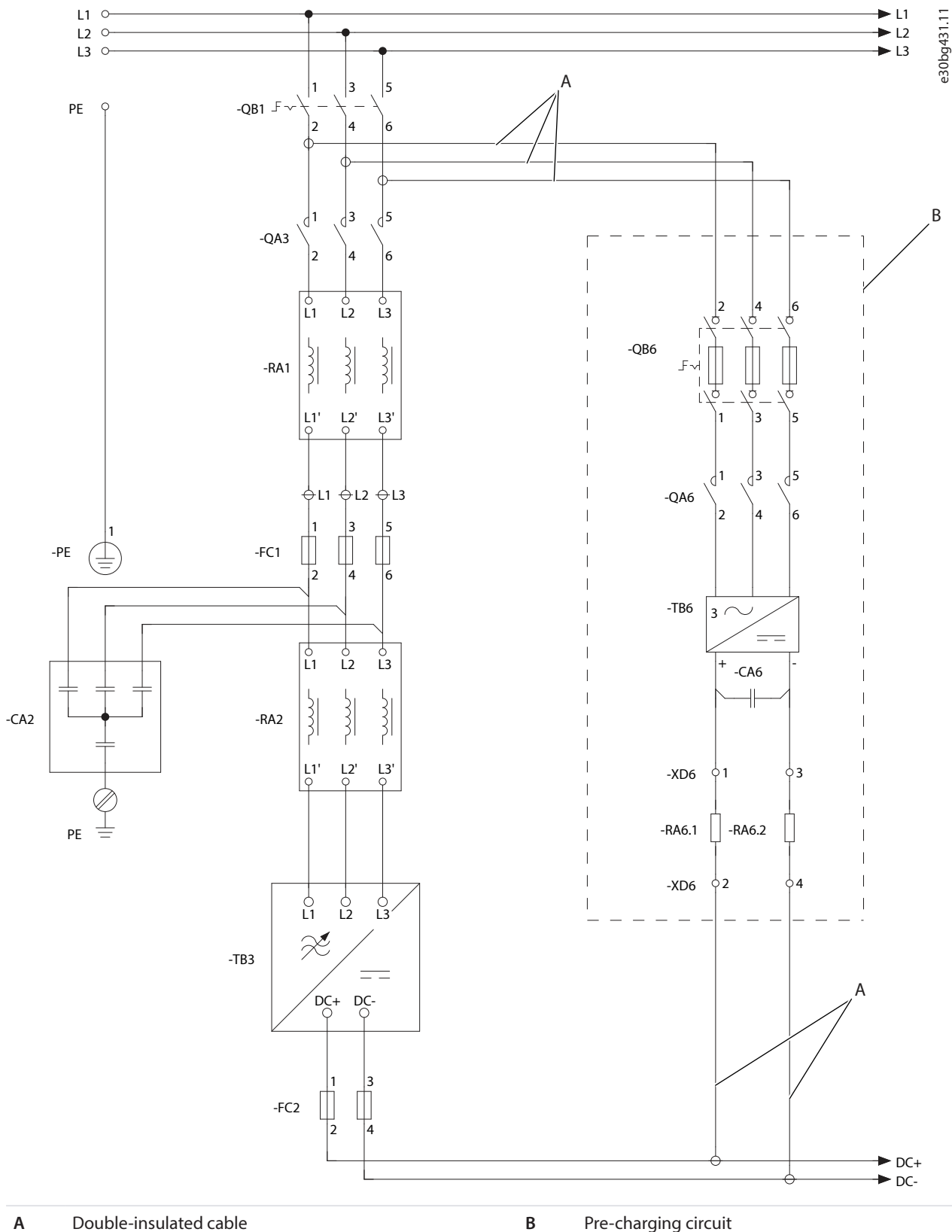
Figure 193: Pre-charging Circuit Diagram, AR10L
