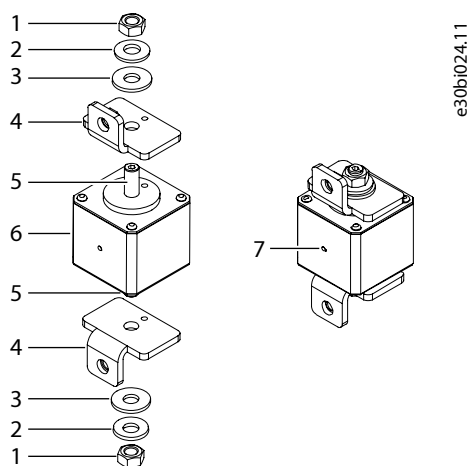
Figure 73: Installing Busbars to the DC Fuses
