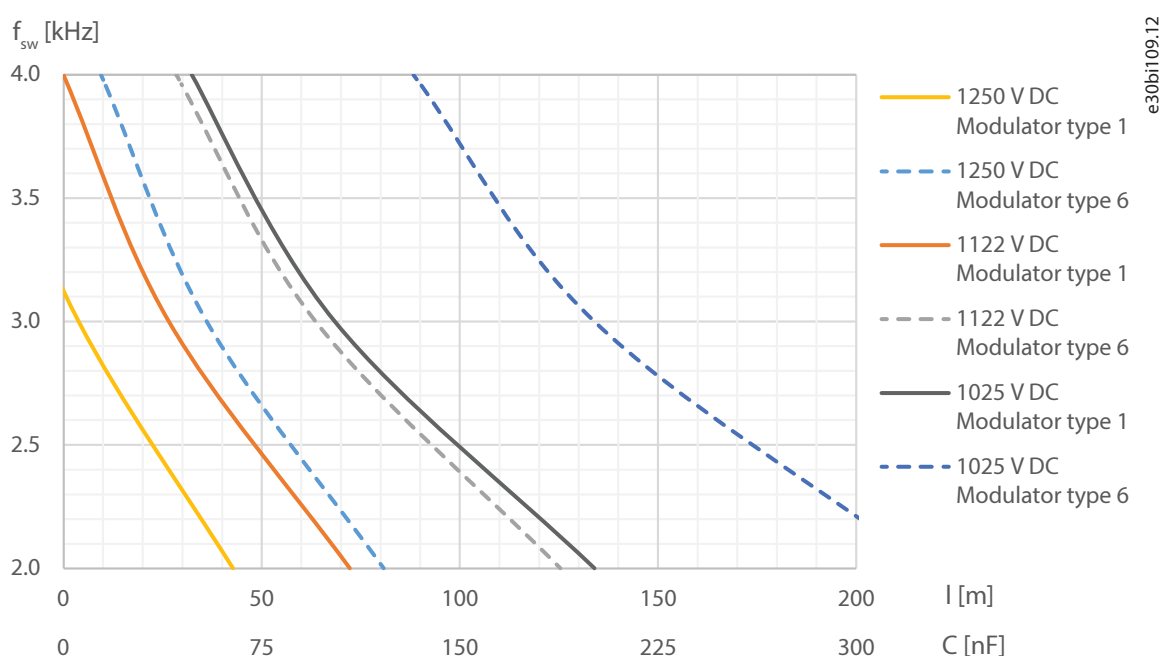
Figure 88: Safe Operation Area: 416 A dU/dt Filter, 100% Flow
