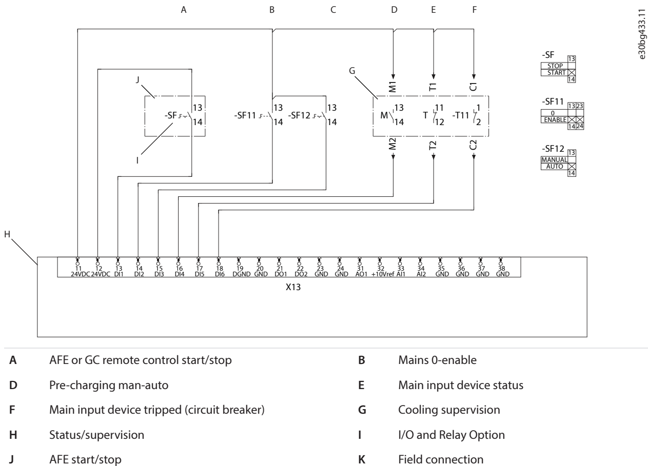
Figure 195: Pre-charging Control Circuit Diagram
