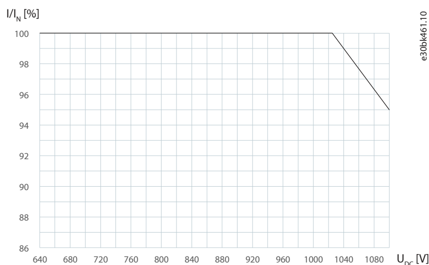
Figure 117: DC-bus Voltage Derating
