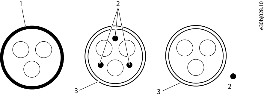
Figure 63: Recommended Cable Types for Mains and Motor Cabling
