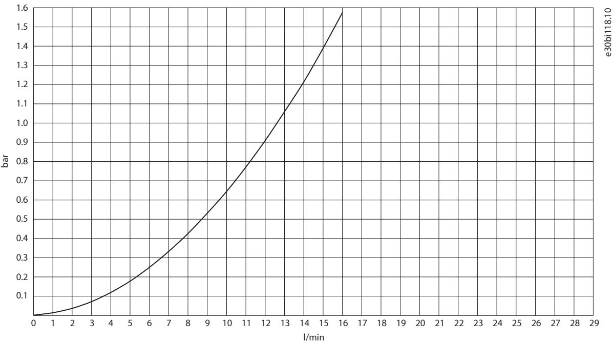
Figure 44: Pressure Drop, Grid-side L Filter OF7Z5, 690 V/1640 A
