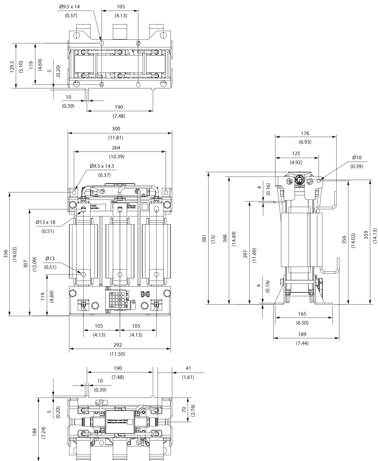
Figure 161: Dimensions of the L Filter, 400 A
