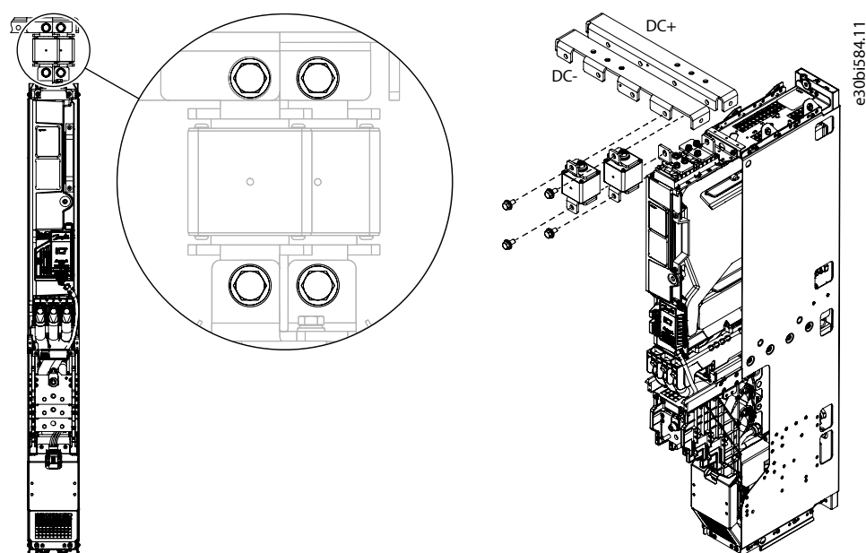
Figure 75: Installing DC Fuse Assemblies
