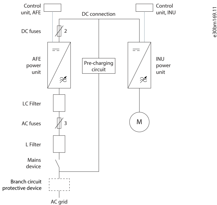
Figure 60: DC Connections of Single Power Units
