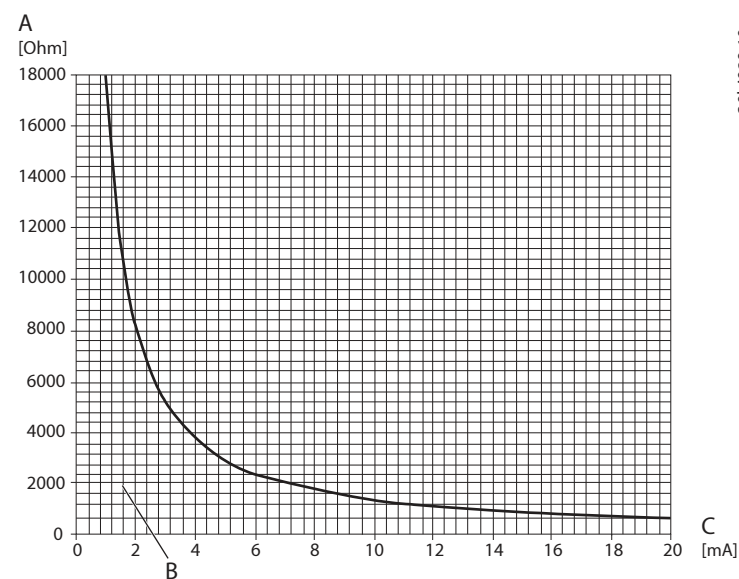
Figure 128: Allowed Load Resistance of Analog Output in Current Mode
