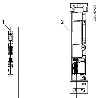
Figure 124: Control Connection
