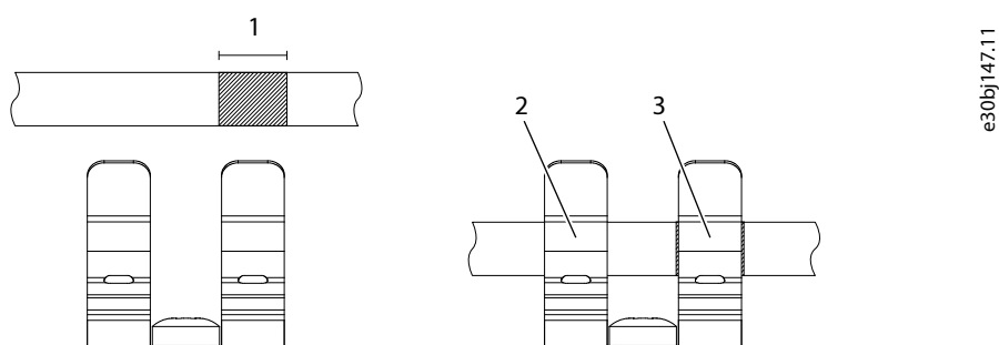
Figure 135: Stripping the Cable and Using the Grounding Plates
