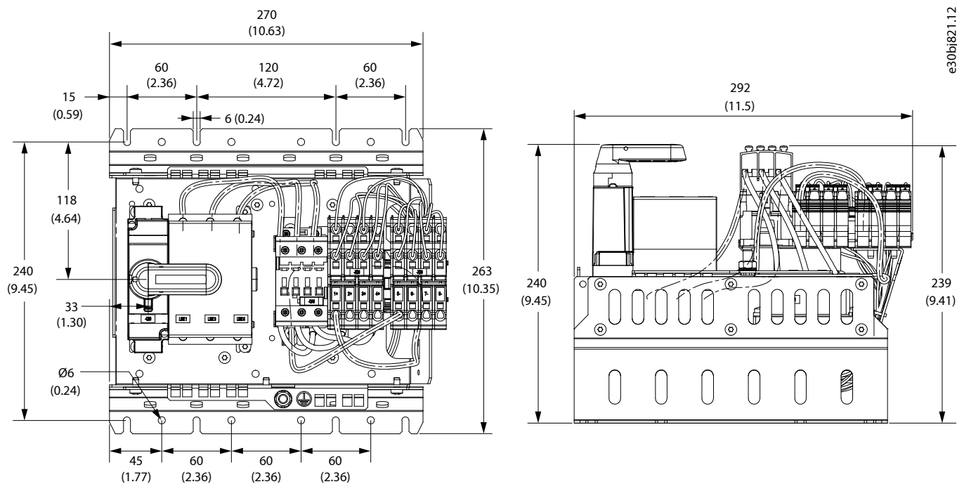
Figure 180: Dimensions of the Pre-charging Unit in mm (in), IEC
