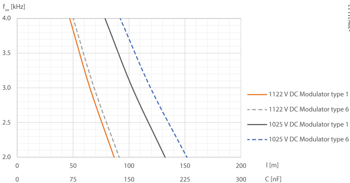
Figure 104: Safe Operation Area: 416 A Common-mode Filter, 100% Flow
