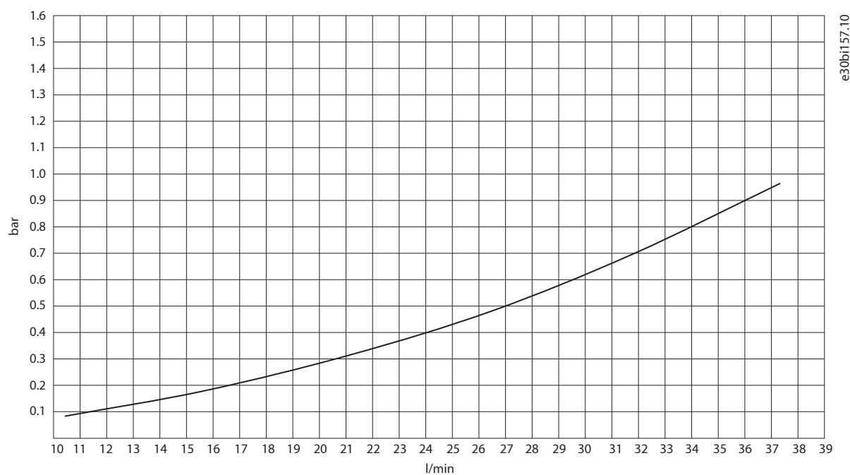
Figure 31: Unit Pressure Drop with Water, IR10L with dU/dt and Common-mode Filter (+AEU1, +AEU2)
