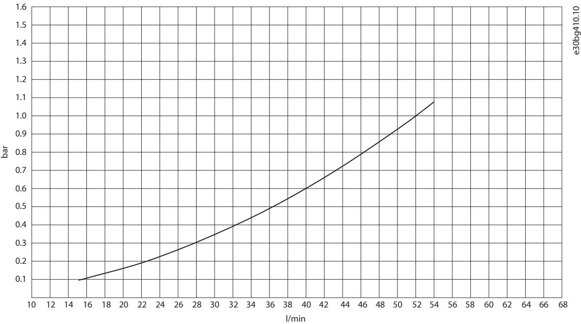
Figure 36: Unit Pressure Drop with Water, AFE AR12L (+AEZ1) and INU IR12L with Sine-wave Filter (+AES1, +AEZ1)
