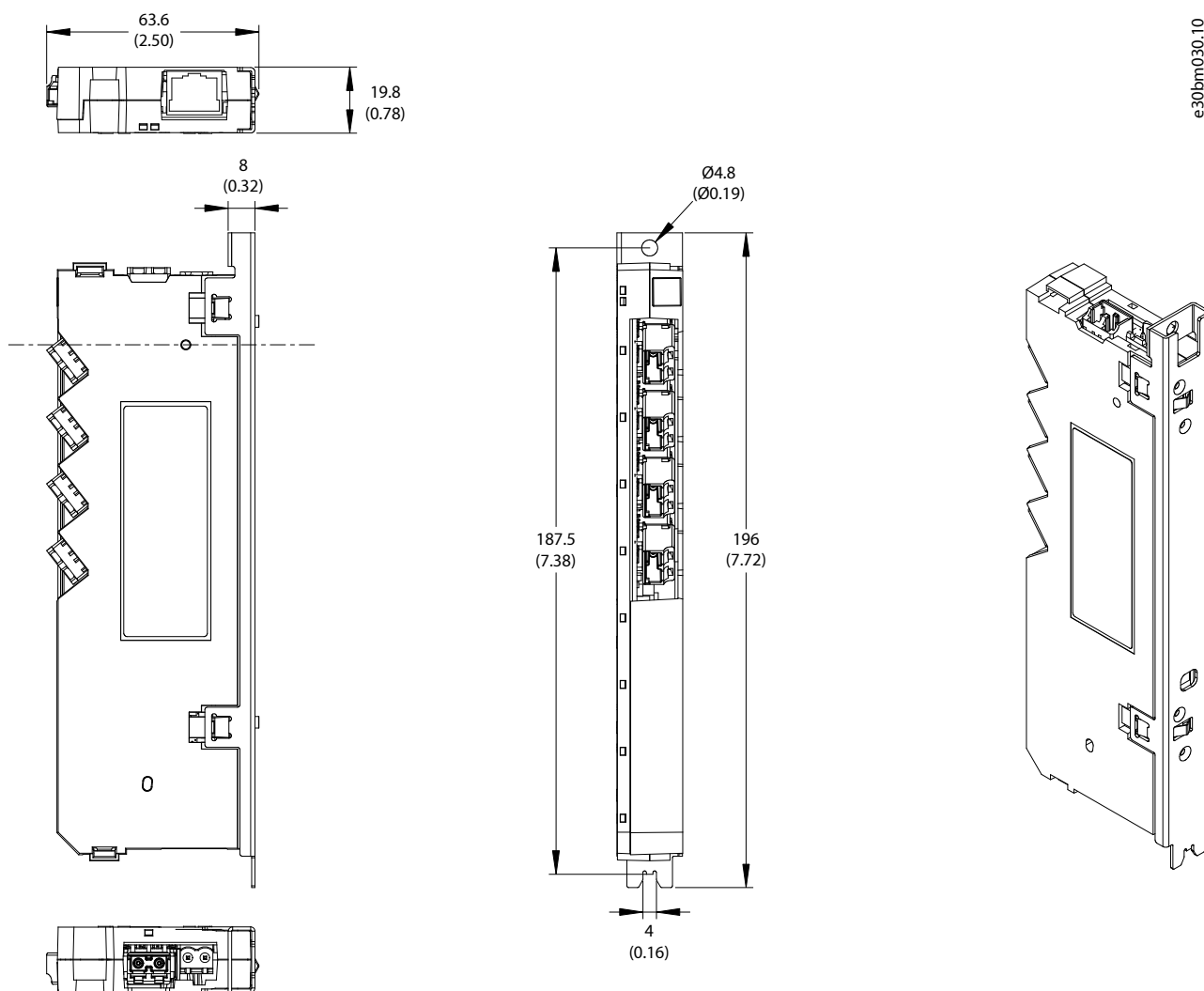
Figure 177: Dimensions of the 4-port Star Coupler Board in mm (in)
