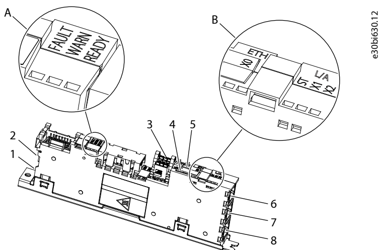
Figure 119: The Control Board
