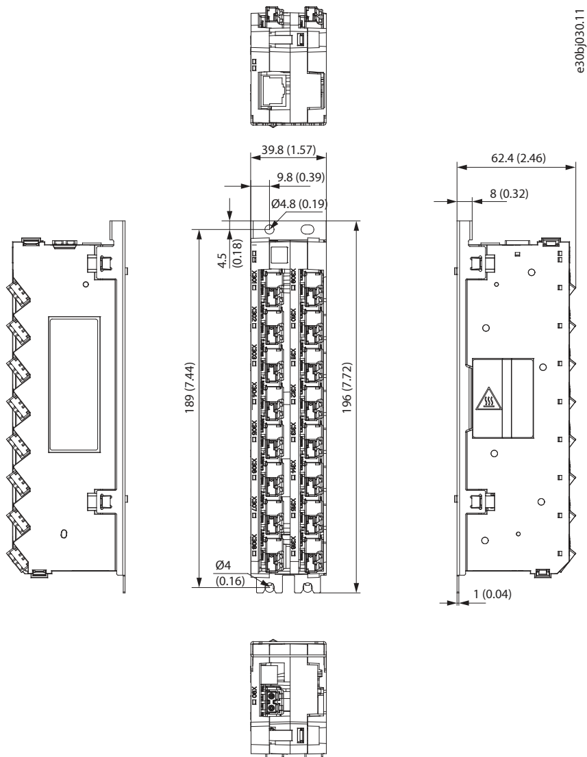
Figure 179: Dimensions of the 16-port Star Coupler Board in mm (in)
