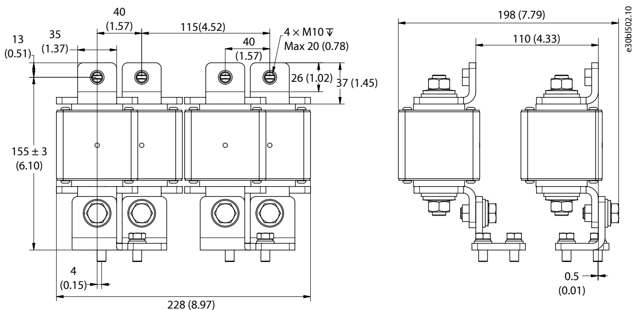
Figure 183: Dimensions of the DC Fuses, AR12L, IR12L, DR12L, AM12L, IM12L, DM12L, in mm (in)
