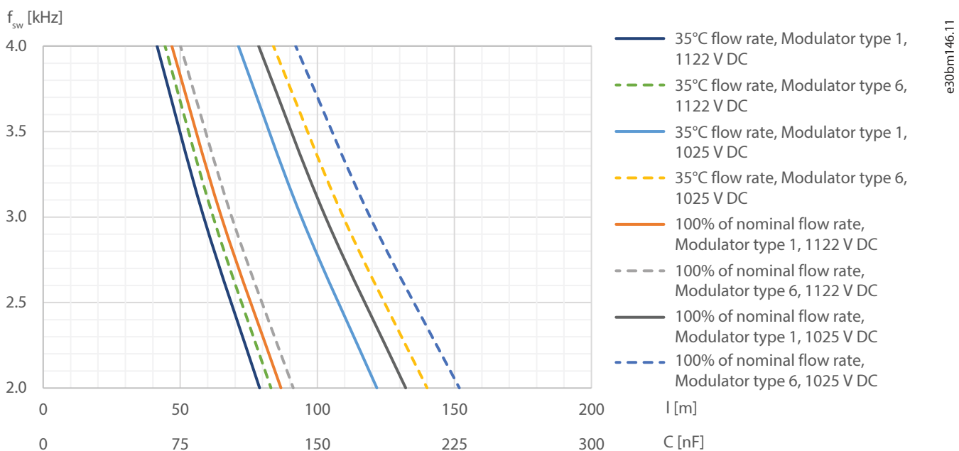
Figure 105: Safe Operation Area: 416 A Common-mode Filter, with Different Flow Rates
