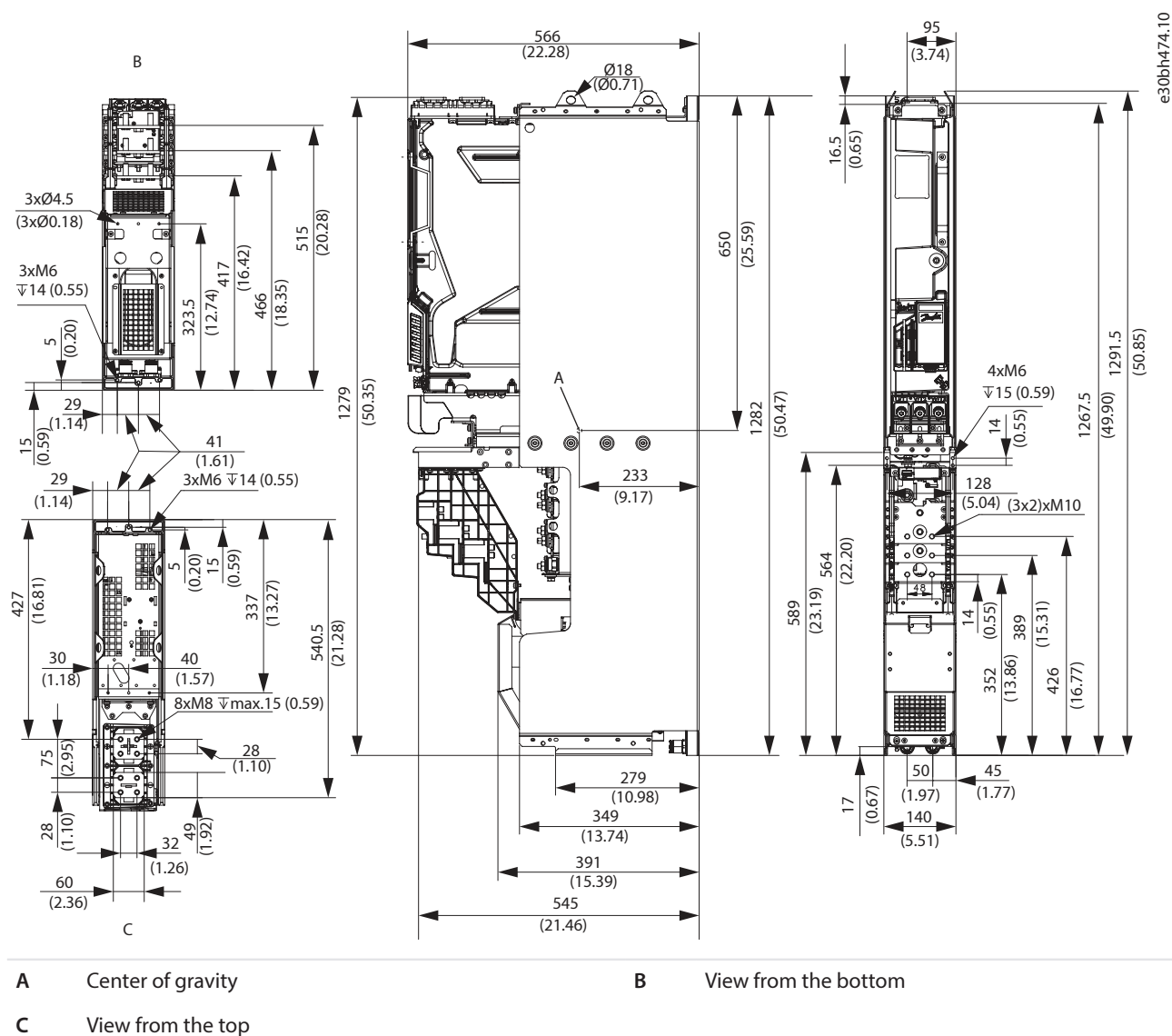
Figure 152: Dimensions of INU, IR10L, in mm (in)
