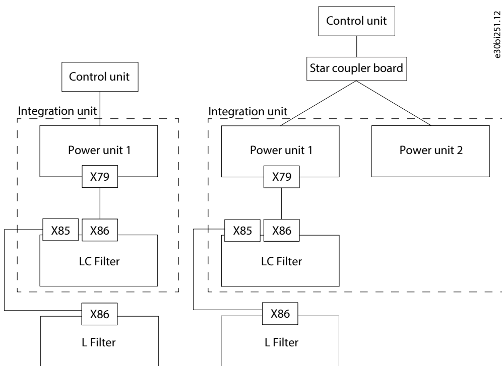
Figure 110: AuxBus Topology for AFE and Grid Converter Modules AR10L and AR12L
