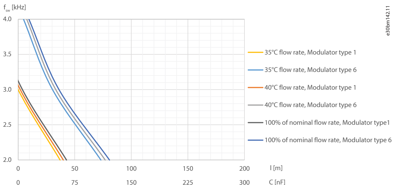
Figure 91: Safe Operation Area with Different Flow Rates: 416 A dU/dt Filter, 1250 V DC
