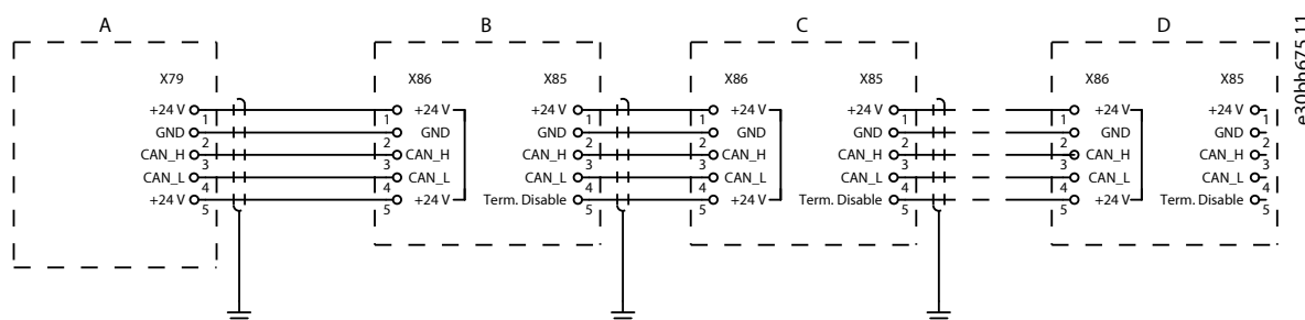
Figure 112: AuxBus Circuit Diagram
