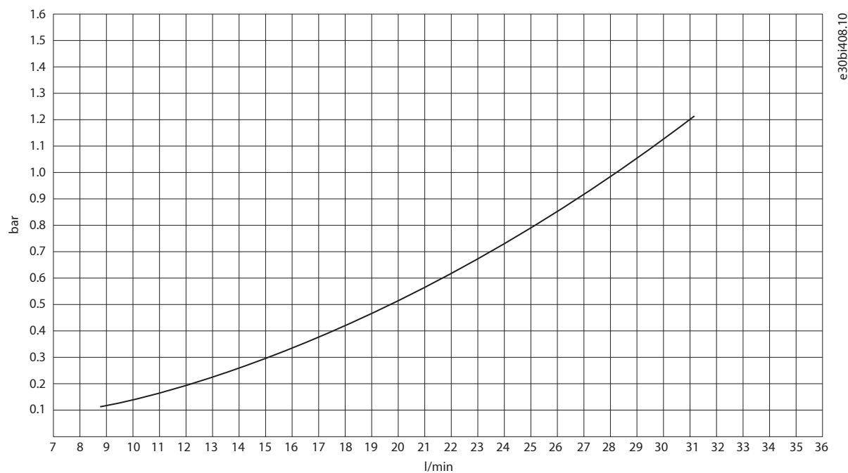
Figure 30: Unit Pressure Drop with Water, AFE AR10L
