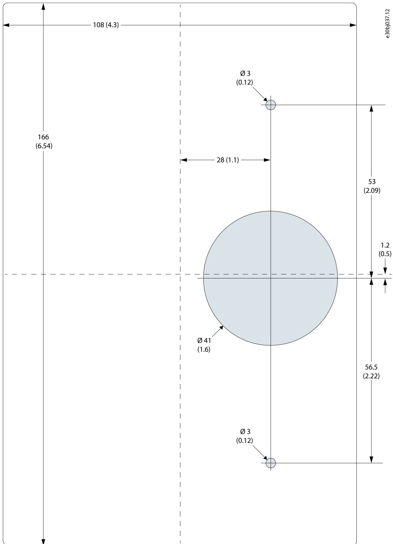
Figure 185: Surface Mounting Kit Drilling Template, mm (in)
