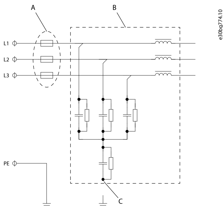
Figure 78: Diagram of the LC Filter
