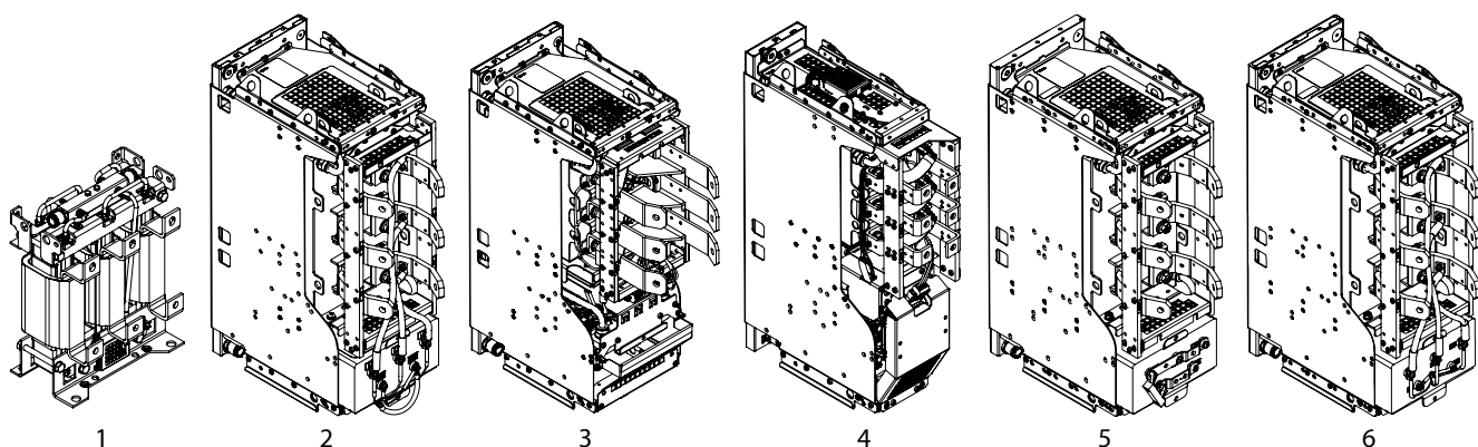
Figure 3: Liquid-cooled Filter Modules
