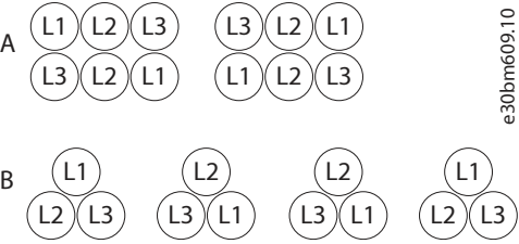
Figure 67: Single-core Cabling: Four Conductors per Phase or Four Circuits
