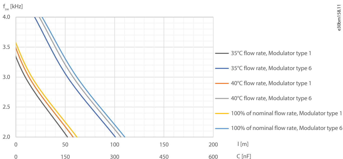
Figure 103: Safe Operation Area with Different Flow Rates: 820 A dU/dt Filter, Low Output Frequency Range, 1250 V DC
