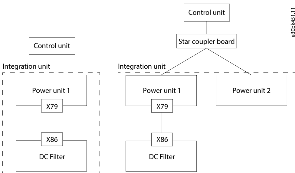
Figure 111: AuxBus Topology for DC/DC Converter Modules DR10L and DR12L
