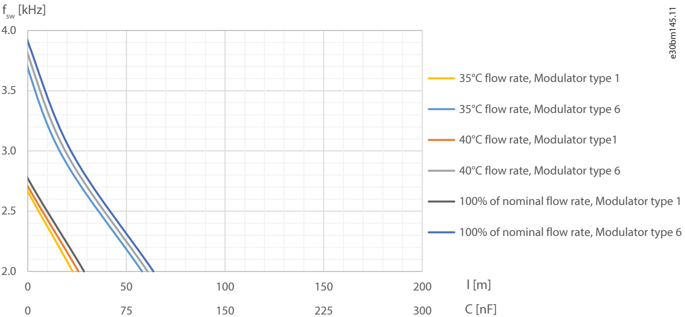
Figure 95: Safe Operation Area with Different Flow Rates: 416 A dU/dt Filter, Low Output Frequency Range, 1250 V DC
