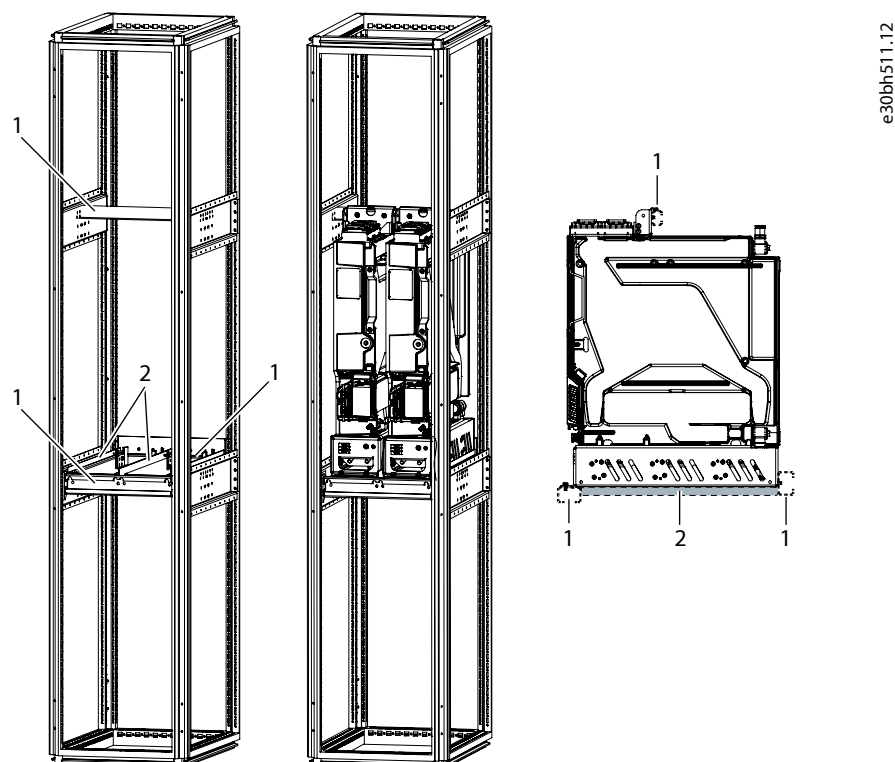
Figure 13: The Mounting Brackets and the Installation of System Modules into the Cabinet
