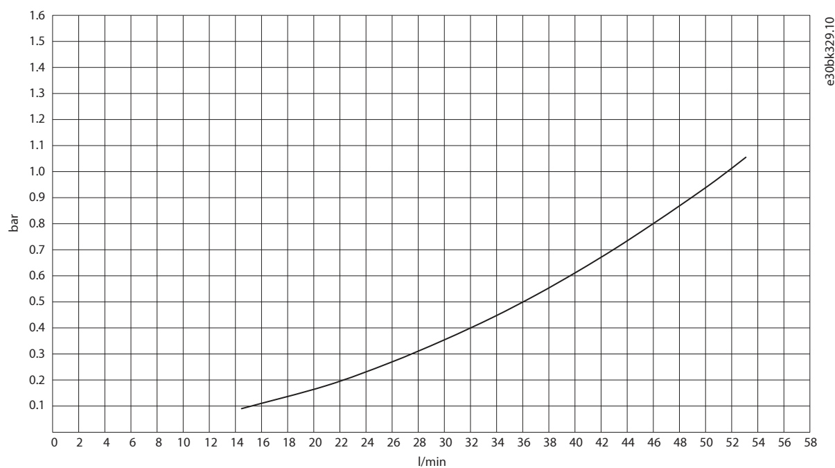
Figure 47: Unit Pressure Drop with Water, DC/DC Converter DR12L with DC Filter (+AED1)
