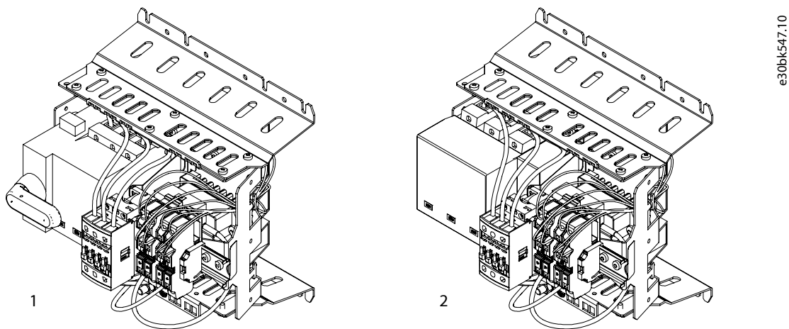
Figure 113: Pre-charging Units
