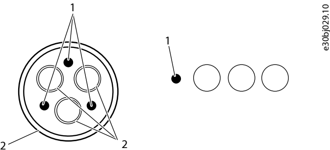
Figure 64: Not Recommended Motor Cable Types
