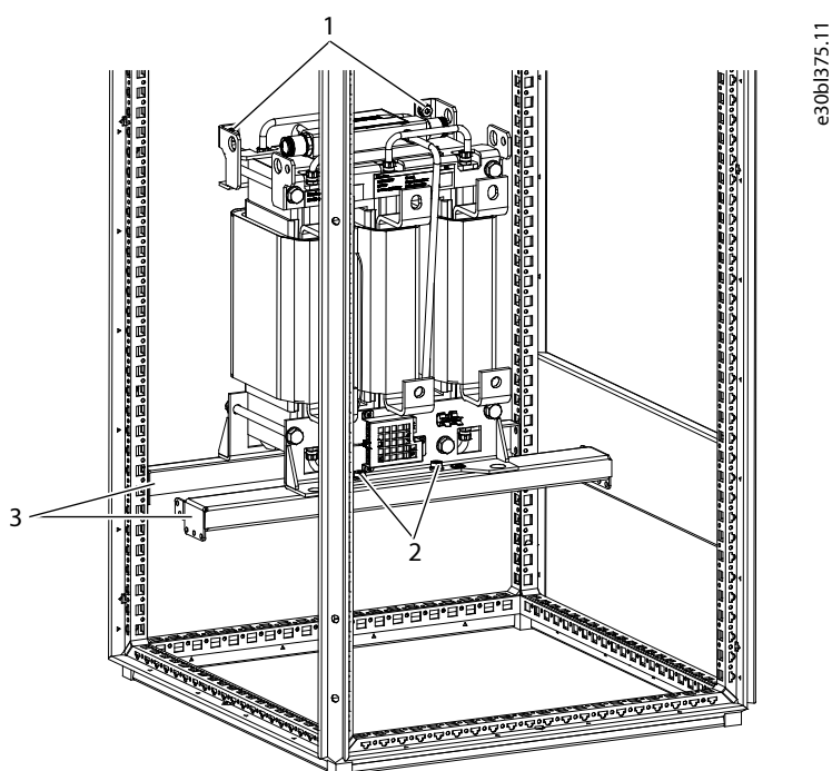
Figure 21: Installing the L Filter into a Cabinet (400 A, 1000 A)
