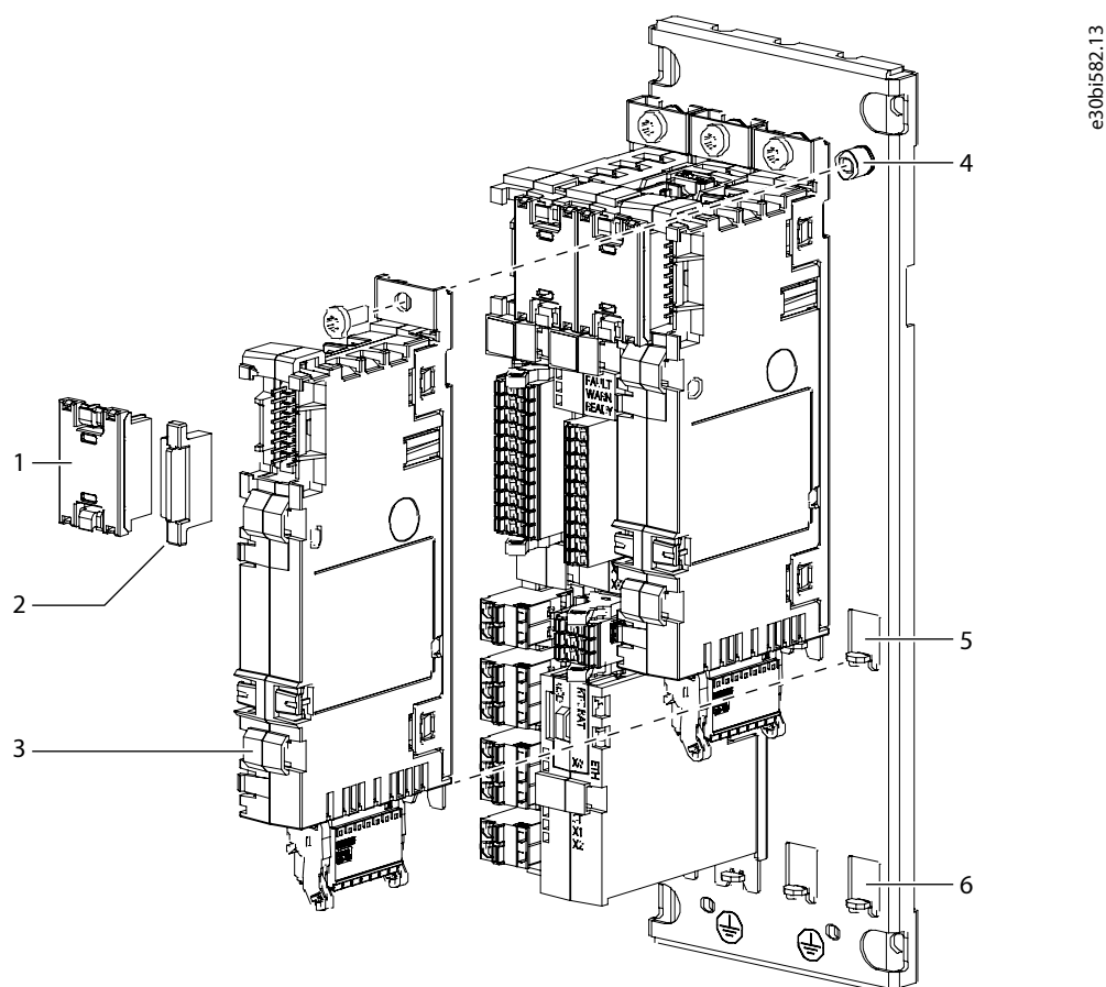
Figure 132: Installing a Board to the Modular Control Unit Mounting Plate
