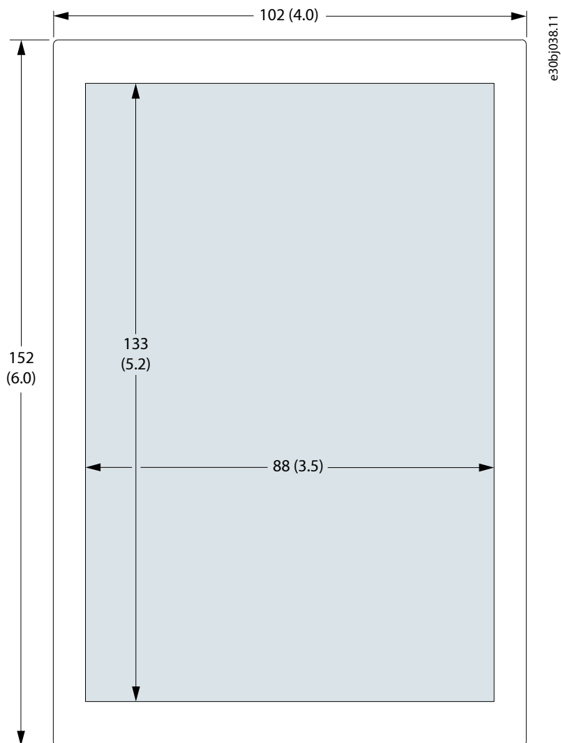
Figure 184: Flush Mounting Kit Drilling Template, mm (in)
