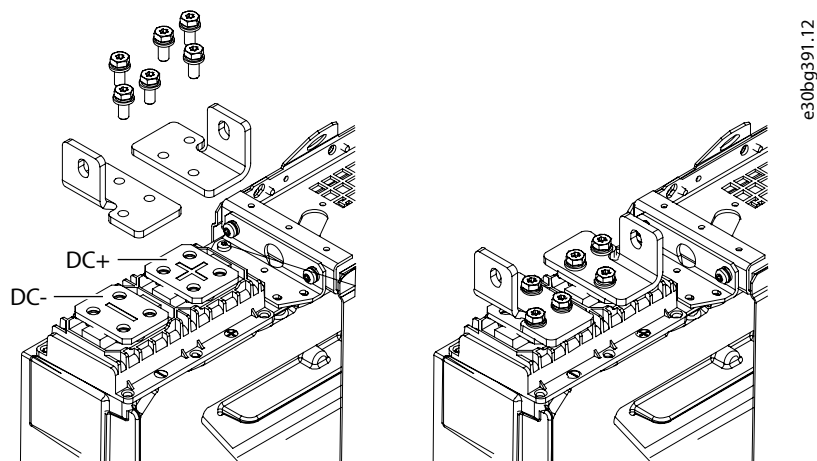
Figure 74: Installing DC-terminal Busbars to the DC Terminals
