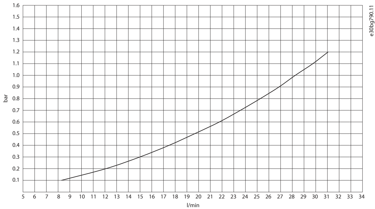
Figure 35: Pressure Drop with Water, dU/dt Filter OF7U1 (+AEU1), 416 A, and dU/dt and CM Filter OF7U2 (+AEU2), 416 A
