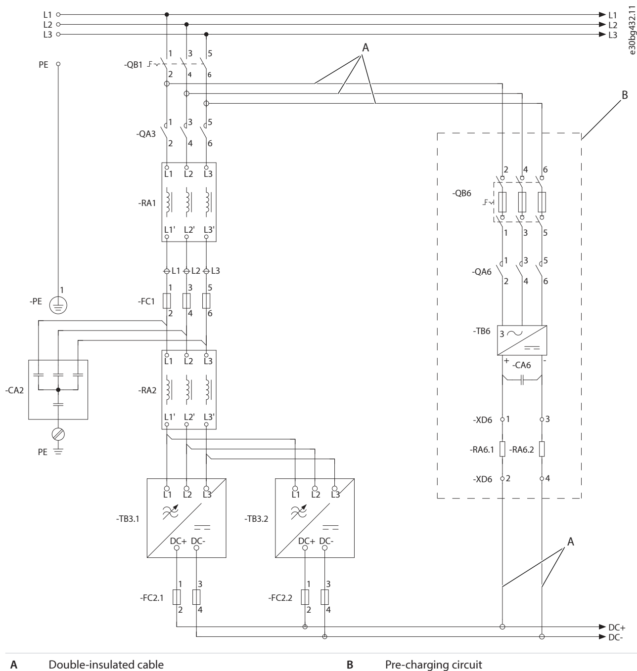
Figure 194: Pre-charging Circuit Diagram, AR12L
