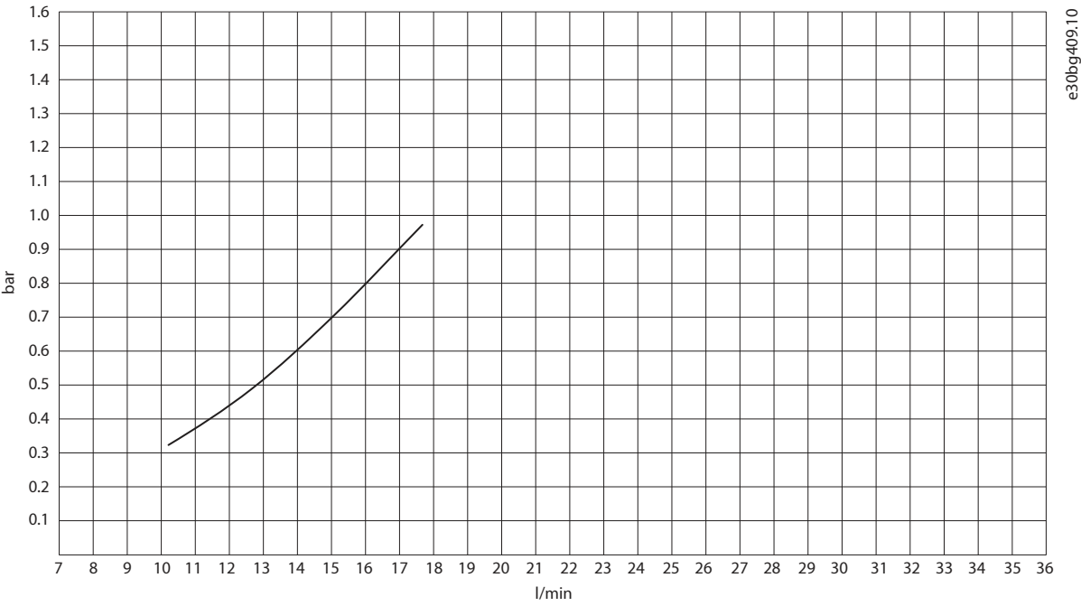
Figure 33: Unit Pressure Drop with Water, INU IR10L without Filters (+AE10)
