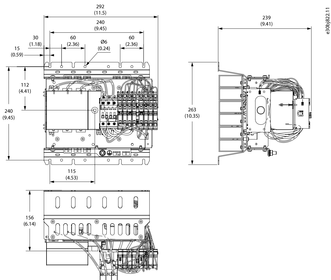
Figure 181: Dimensions of the Pre-charging Unit in mm (in), UL
