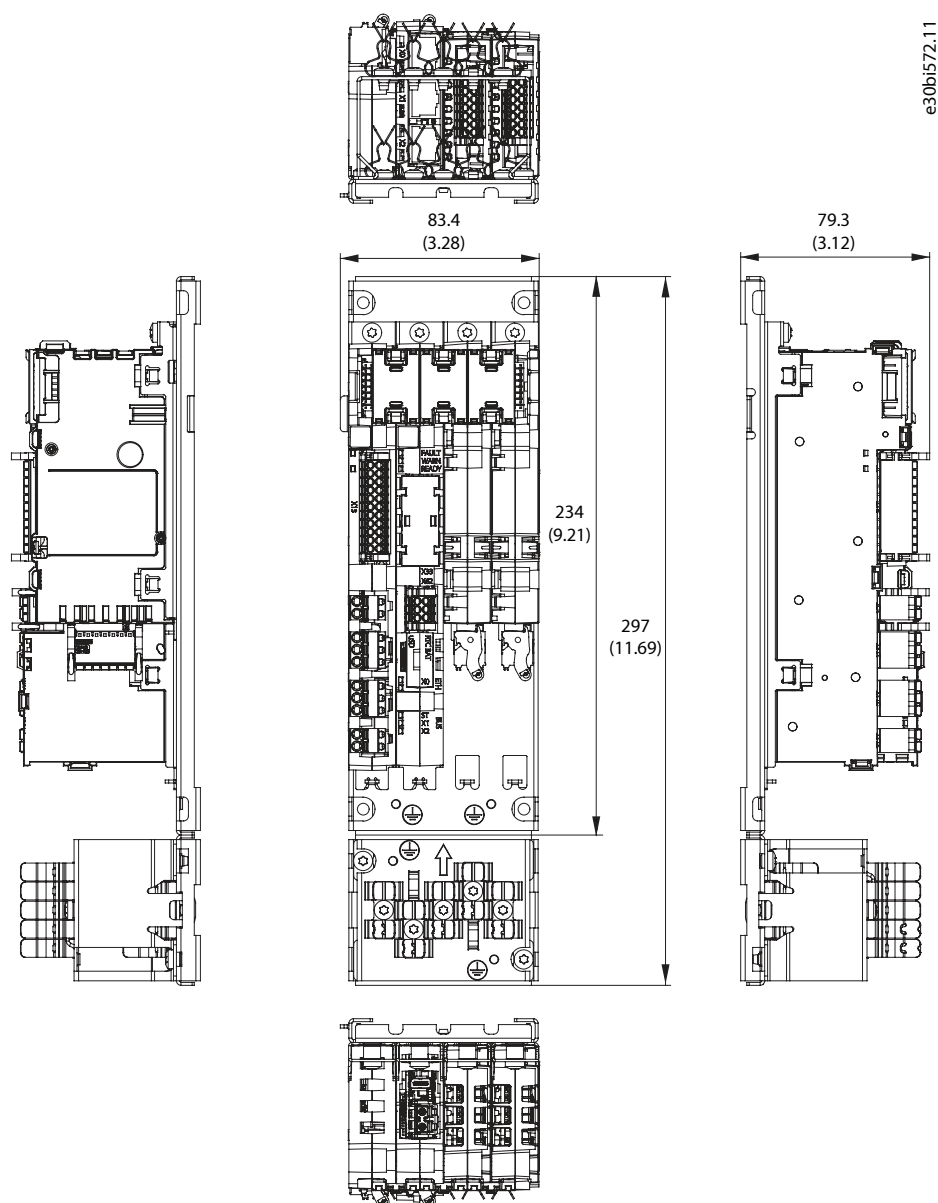
Figure 170: Dimensions of the Control Unit in mm (in), Example Configuration
