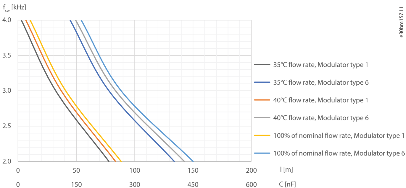
Figure 102: Safe Operation Area with Different Flow Rates: 820 A dU/dt Filter, Low Output Frequency Range, 1122 V DC
