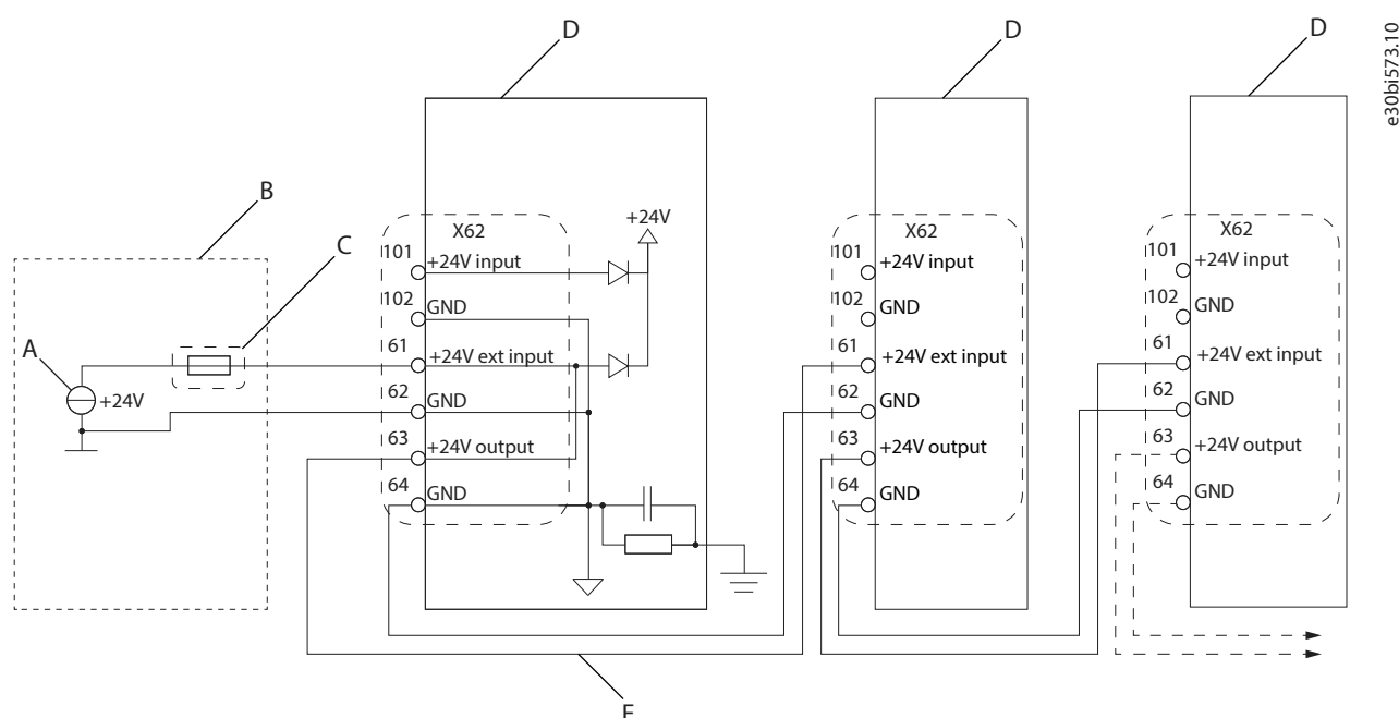
Figure 198: Wiring Diagram of a Daisy-chained +24 V Supply for the Control Units
