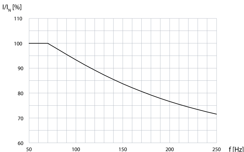
Figure 87: Output Frequency Derating
