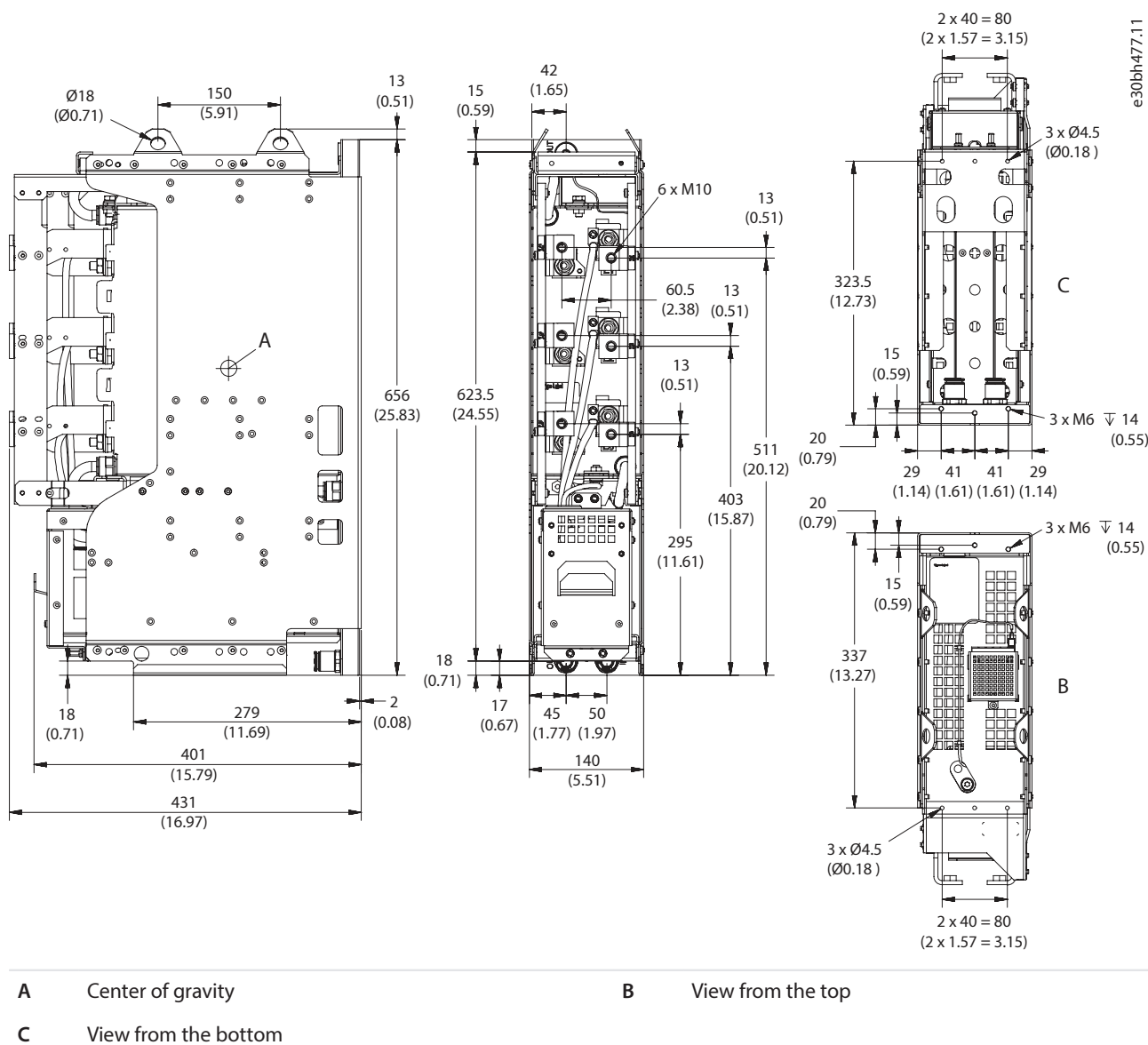
Figure 159: Dimensions of the LC Filter for AM10L, in mm (in)
