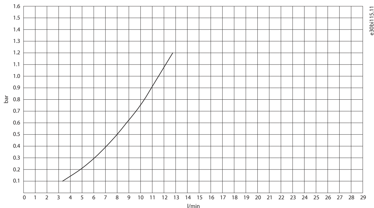
Figure 42: Pressure Drop, Grid-side L Filter OF7Z5, 690 V/400 A
