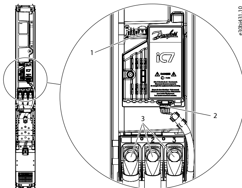
Figure 141: Disconnecting the Cables from the System Module
