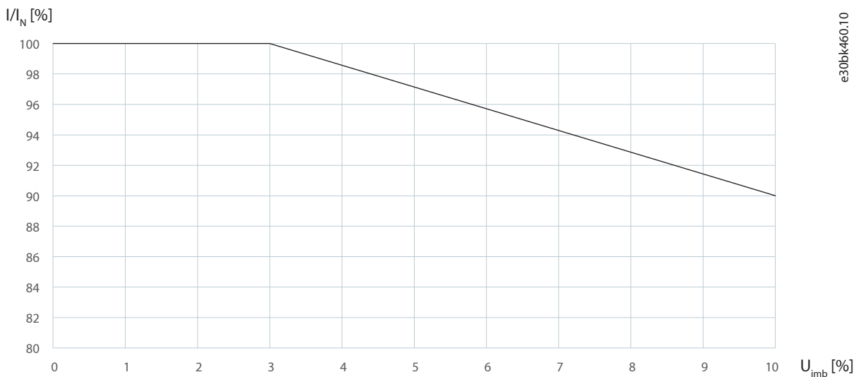
Figure 116: Voltage Imbalance Derating
