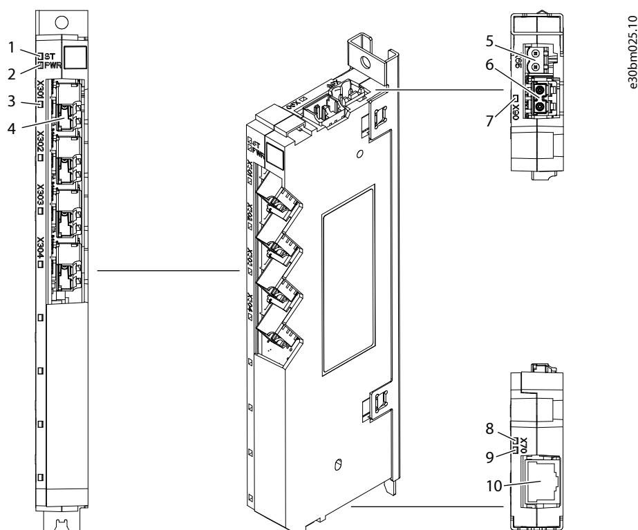
Figure 121: Terminal and Indicator Light Locations on the 4-port Star Coupler Board
