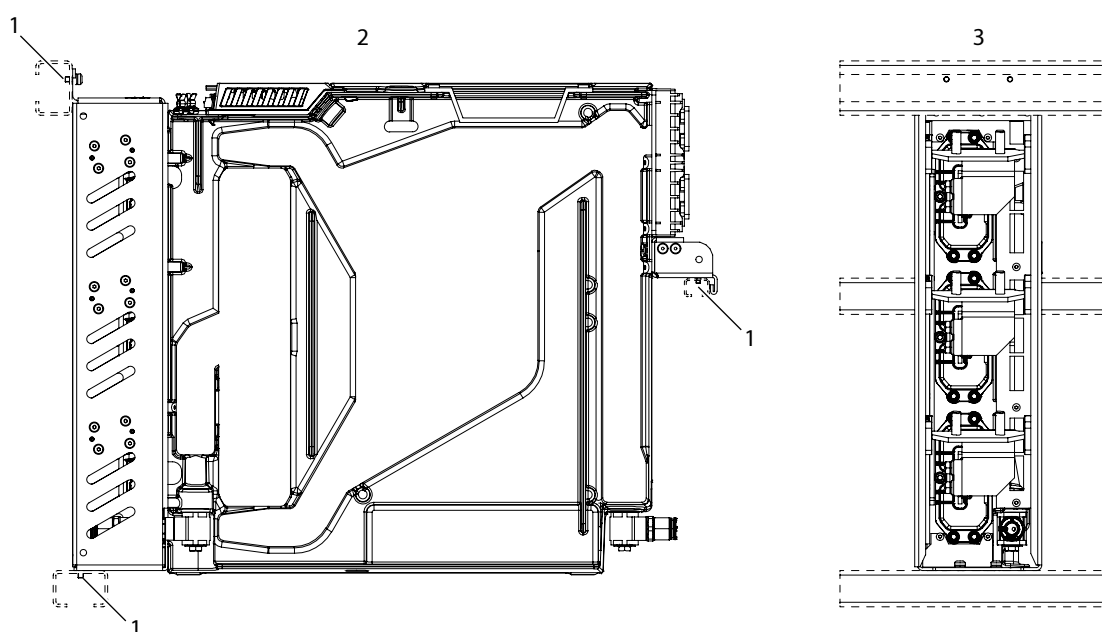
Figure 15: Mounting Holes of the System Module on its Backside
