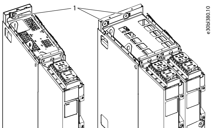
Figure 54: Optional Outlet Connectors of IR10L (left) and IR12L (right)
