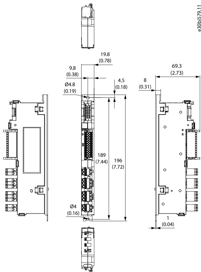
Figure 175: Dimensions of the I/O and Relay Option in mm (in)
