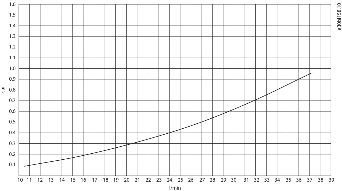
Figure 32: Unit Pressure Drop with Water, IR10L with dU/dt Filter (+AEU1)
