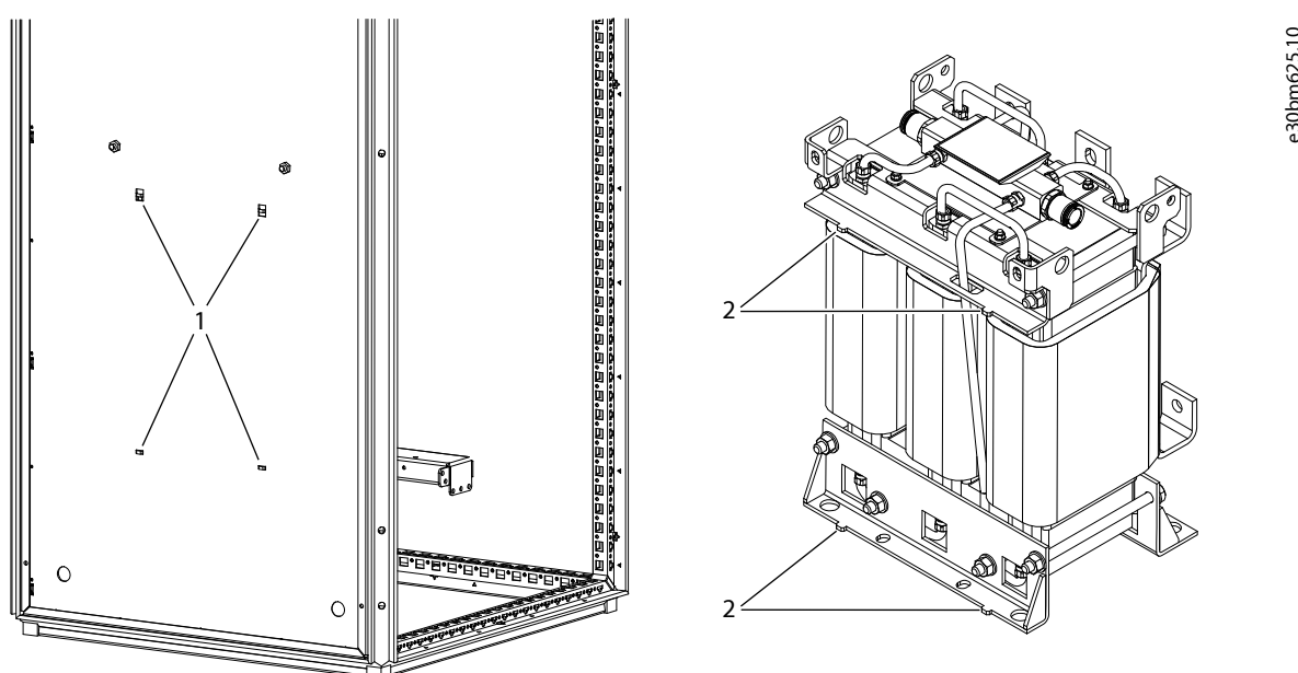
Figure 20: Aligning the Filter Pins with the Back Wall
