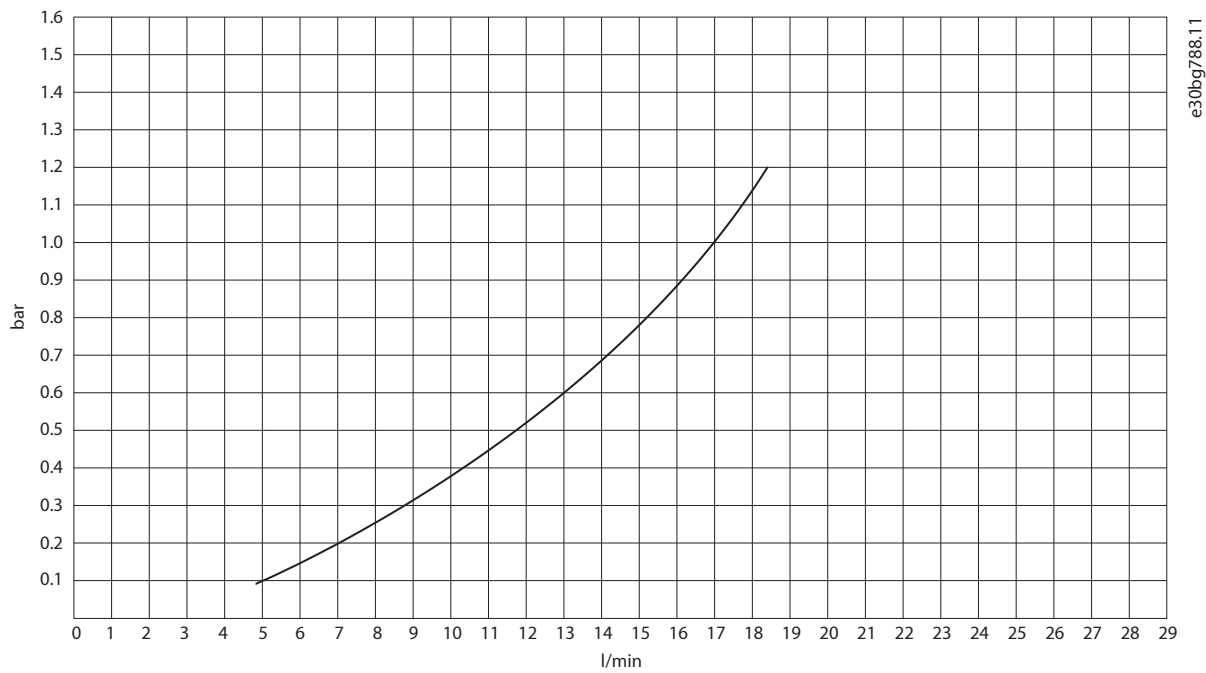
Figure 39: Pressure Drop with Water, LC Filter for AFE OF7Z1 (+AEZ1), 760 A
