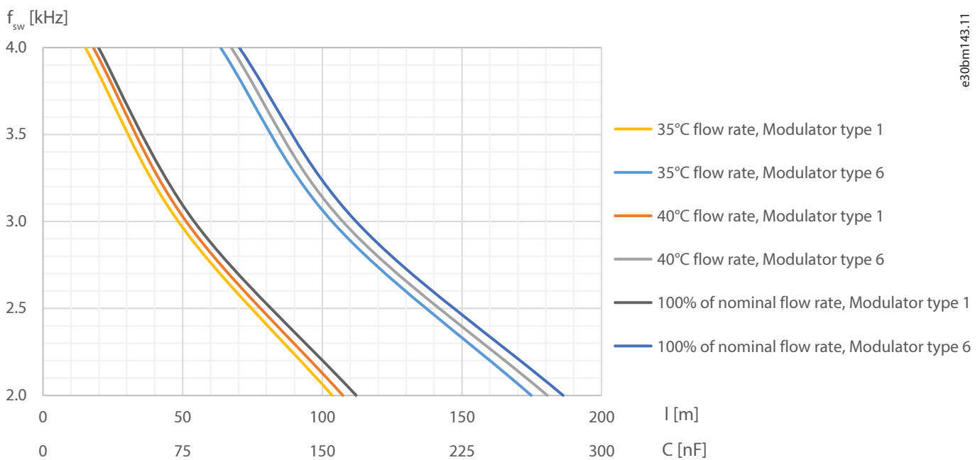
Figure 93: Safe Operation Area with Different Flow Rates: 416 A dU/dt Filter, Low Output Frequency Range, 1025 V DC
