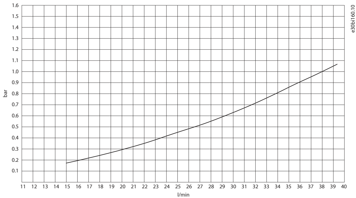
Figure 38: Unit Pressure Drop with Water, INU IR12L without Filters (+AE10)
