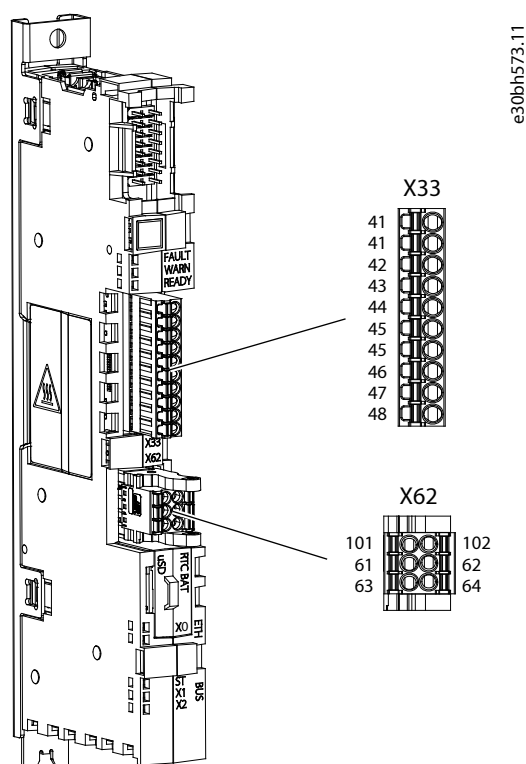
Figure 120: Control Board Terminal Block and Terminal Numbering
