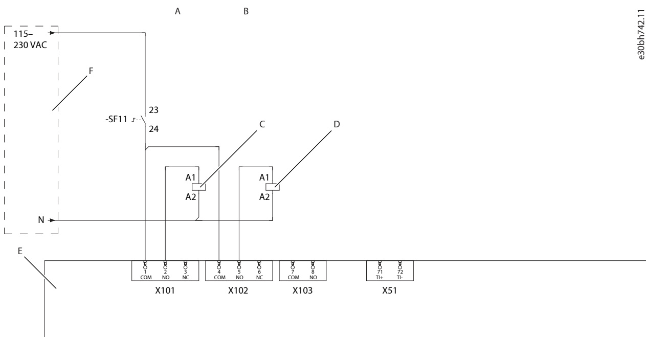
Figure 196: Pre-charging Control Circuit Diagram
