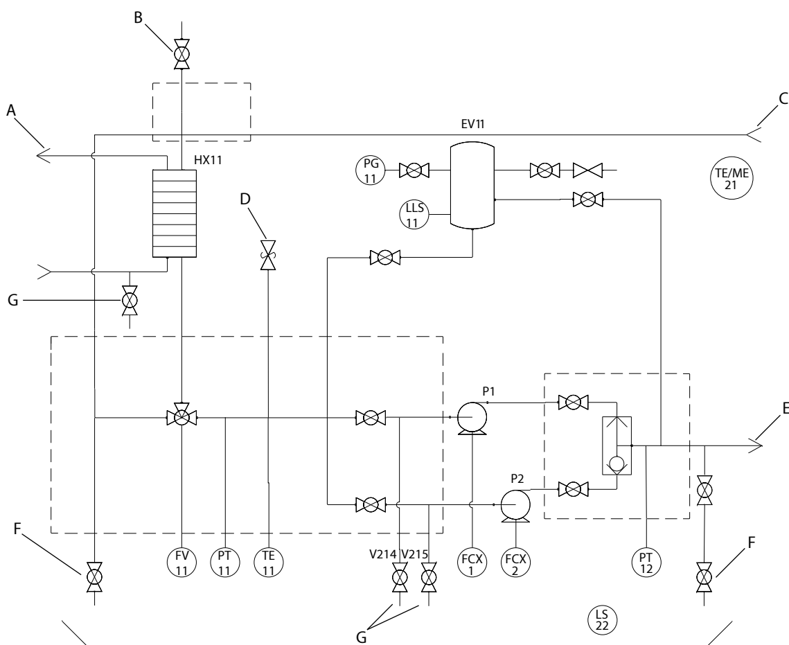
Figure 23: Example PID Diagram of the Cooling Circuit
