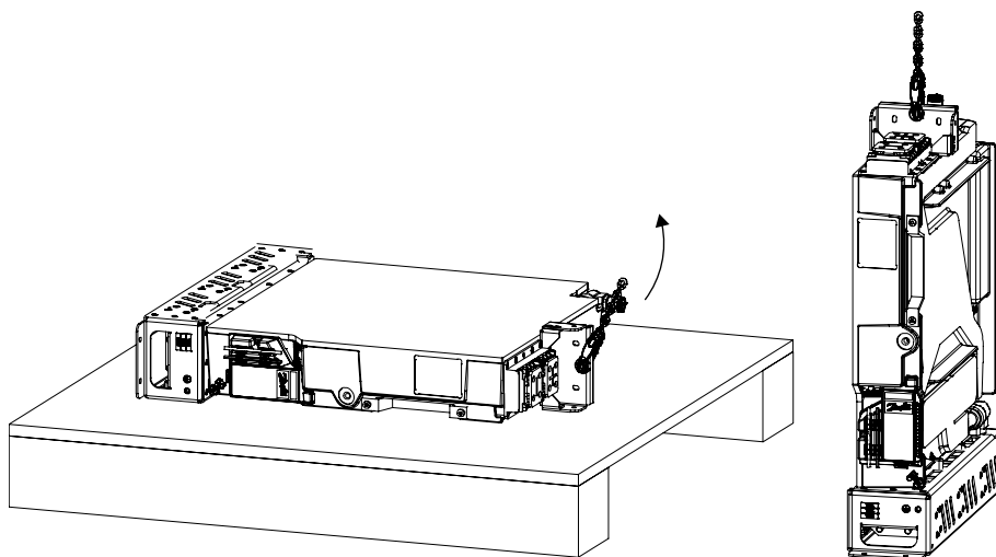
Figure 9: Lifting the System Module
