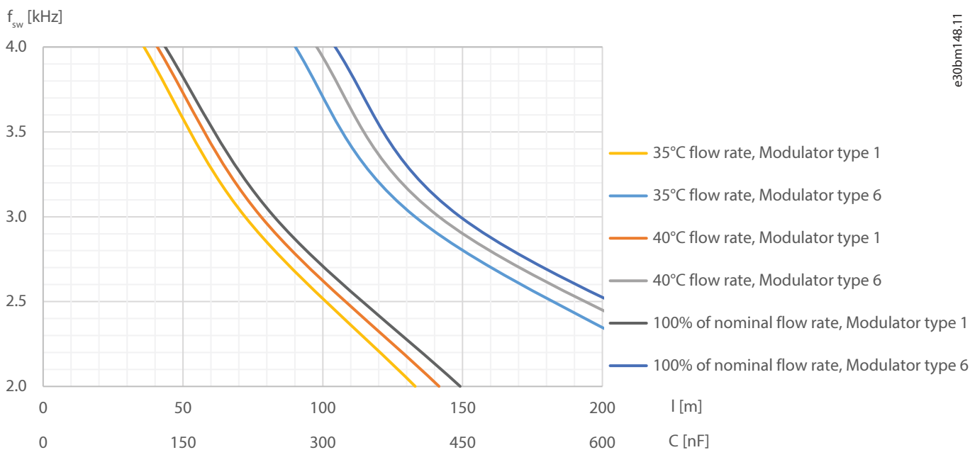
Figure 97: Safe Operation Area with Different Flow Rates: 820 A dU/dt Filter, 1025 V DC
