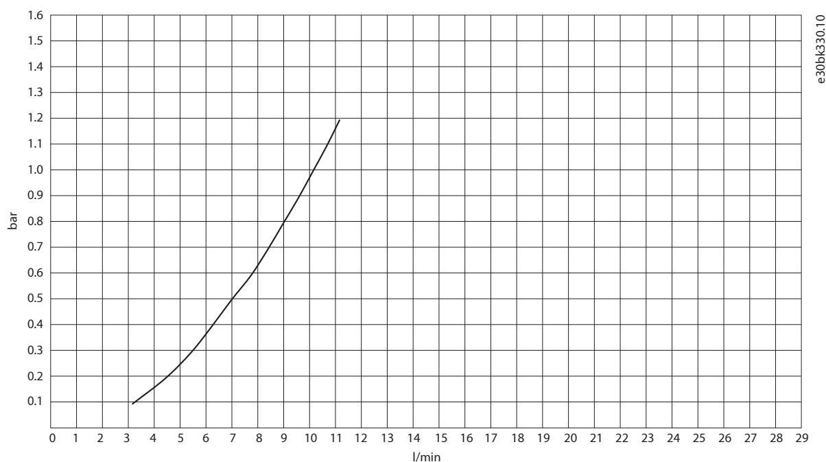
Figure 48: Pressure Drop with Water, DC Filter for DC/DC Converter OF7D1, 570 A
