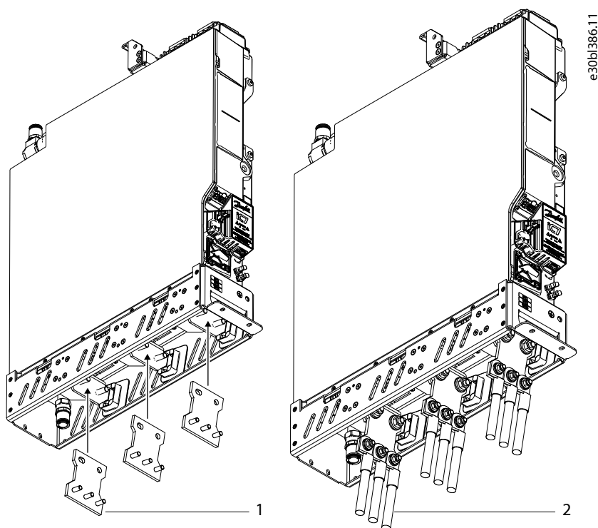
Figure 72: Installation of Cables with the Power Terminal Adapter, Example of IM10L
