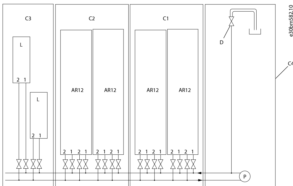
Figure 24: L Filter Cooling Connection Example, 4 x AR12L and 2 x L Filter 1640 A
