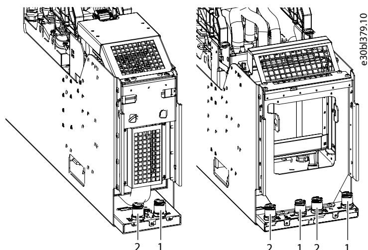
Figure 53: Inlet and Outlet Connectors of IR10L (left) and IR12L (right)
