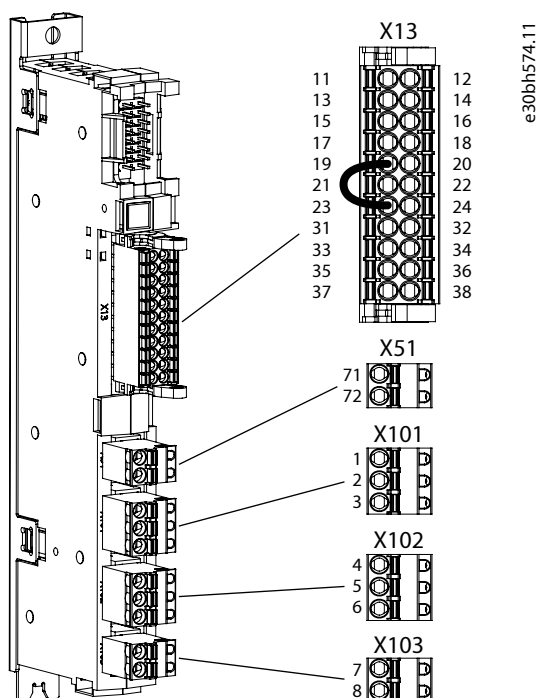
Figure 127: I/O and Relay Option Terminal Block and Terminal Numbering
