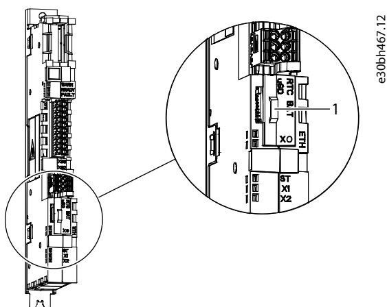
Figure 138: Location of the RTC Battery
