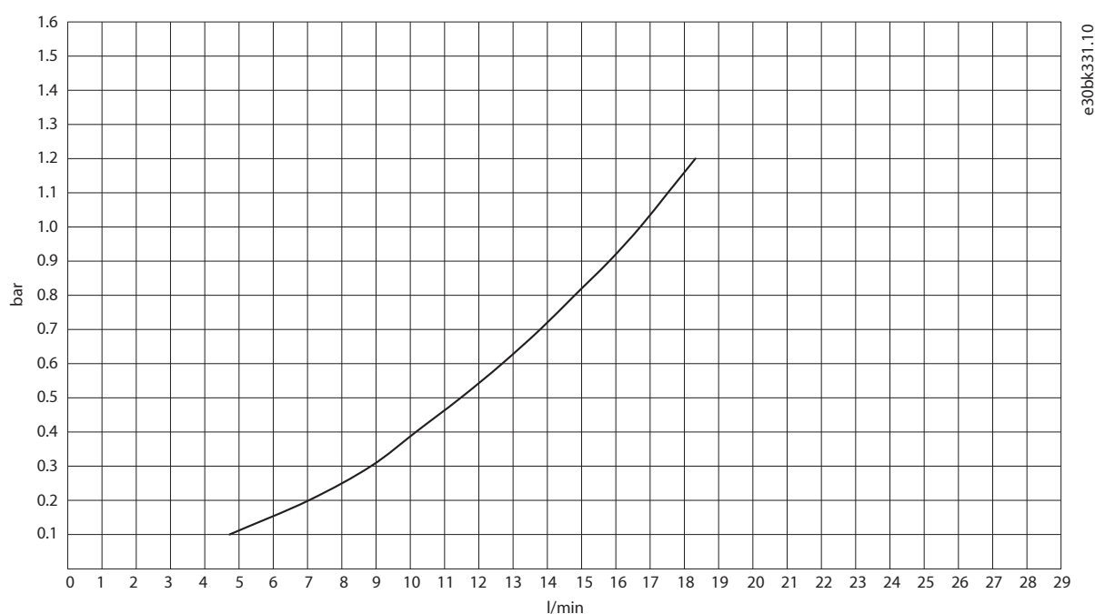
Figure 49: Pressure Drop with Water, DC Filter for DC/DC Converter OF7D1, 1200 A
