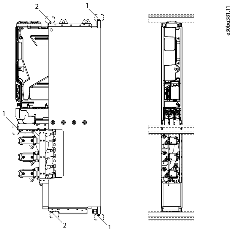
Figure 16: Mounting Holes of the System Module, AFE with the Integration Unit
