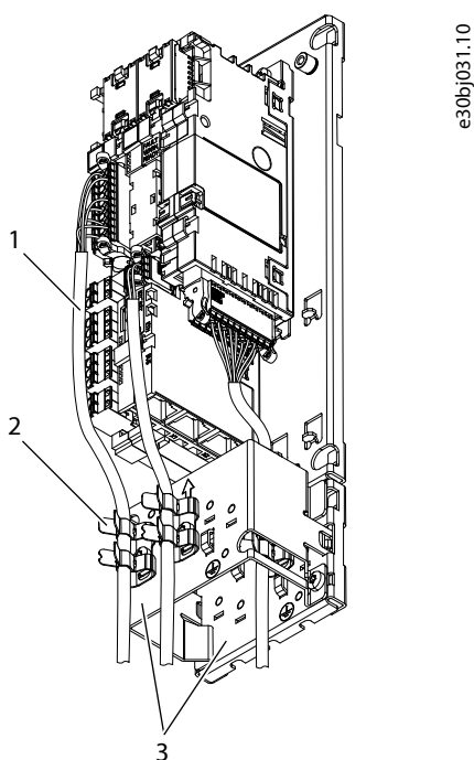
Figure 134: Example of Installing the Control Cables
