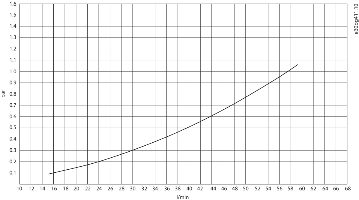
Figure 37: Unit Pressure Drop with Water, INU IR12L with dU/dt Filter (+AEU1)
