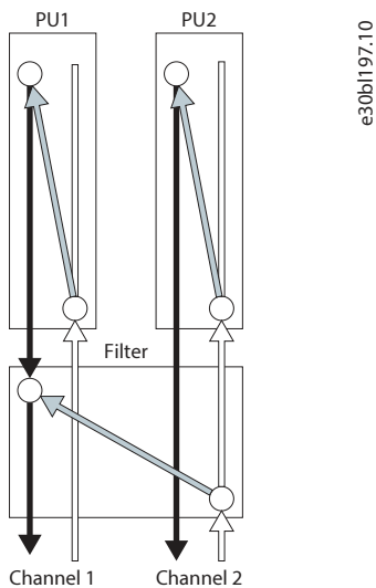
Figure 25: Coolant Flow in Parallel Power Units
