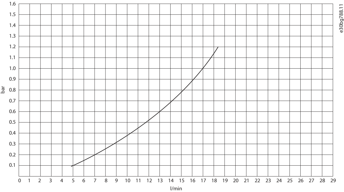
Figure 41: Pressure Drop with Water, Sine-wave Filter OF7S1SM (+AES1), 800 A
