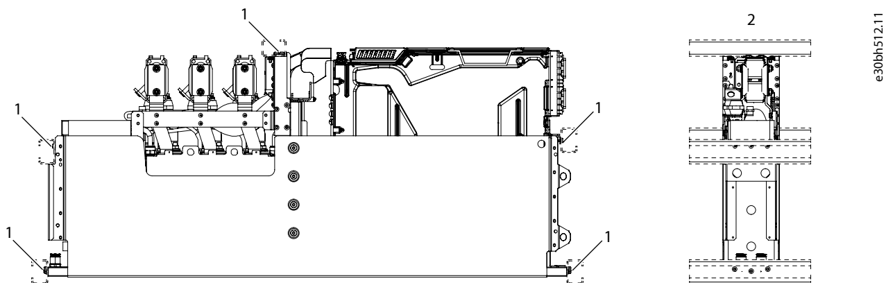
Figure 19: Mounting Holes of the System Module with the Integration Unit on its Backside
