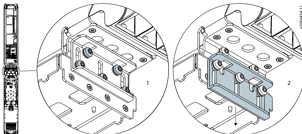
Figure 144: Releasing the Locking Plate
