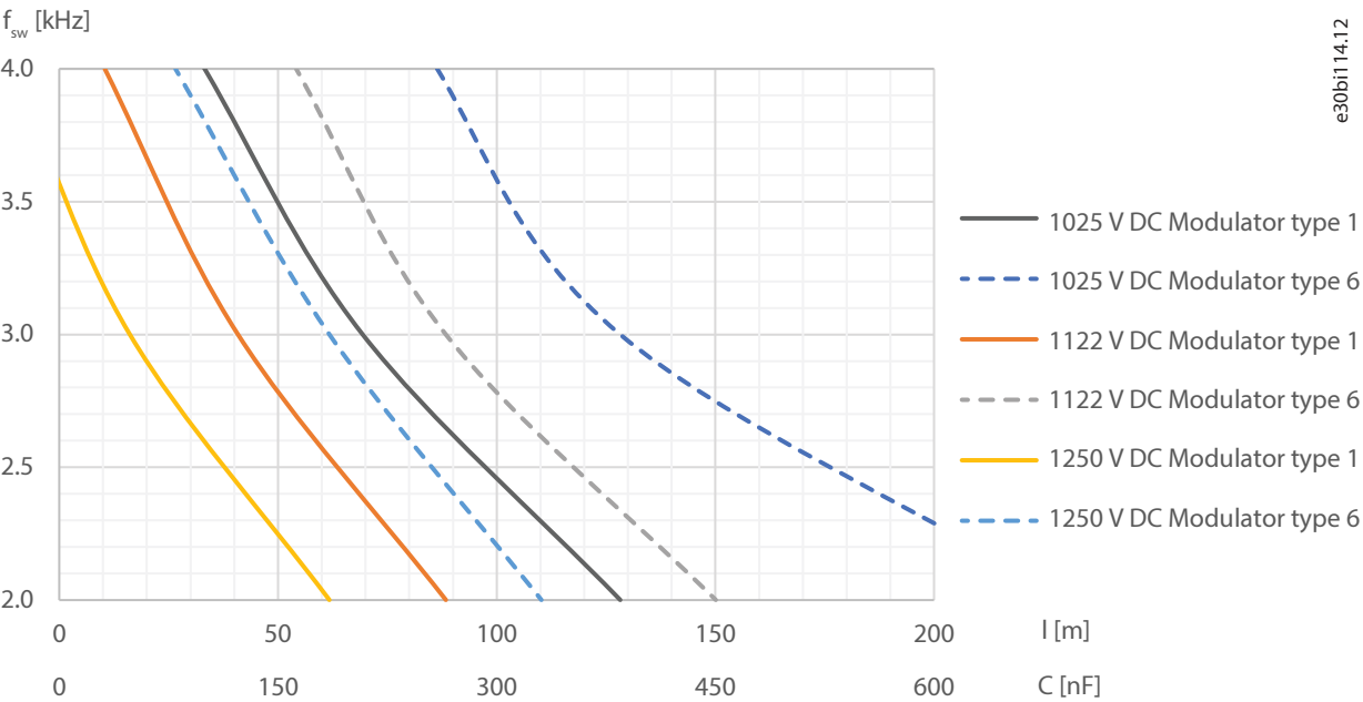
Figure 100: Safe Operation Area: 820 A dU/dt Filter, Low Output Frequency Range, 100% Flow
