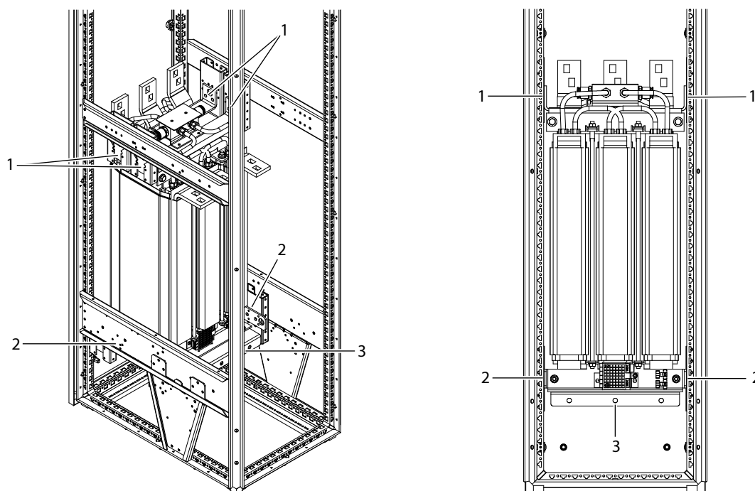
Figure 22: Installing the L Filter into a Cabinet (1640 A, 2300 A)
