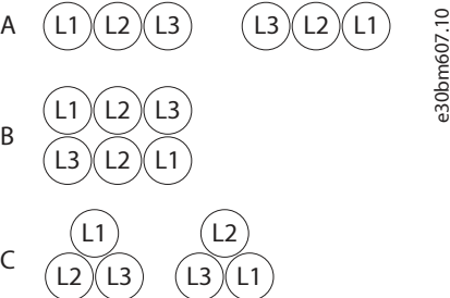
Figure 65: Single-core Cabling: Two Conductors per Phase or Two Circuits
