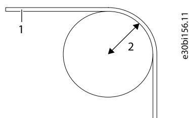
Figure 136: Bending Radius of the Fiber Cables
