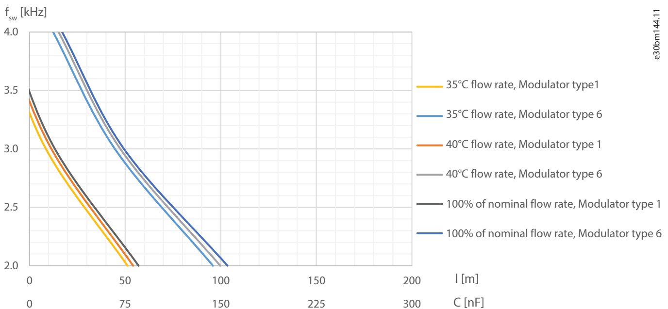
Figure 94: Safe Operation Area with Different Flow Rates: 416 A dU/dt Filter, Low Output Frequency Range, 1122 V DC
