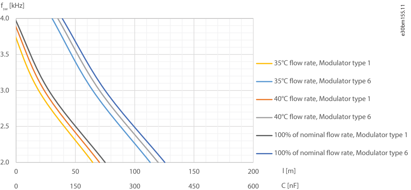
Figure 99: Safe Operation Area with Different Flow Rates: 820 A dU/dt Filter, 1250 V DC
