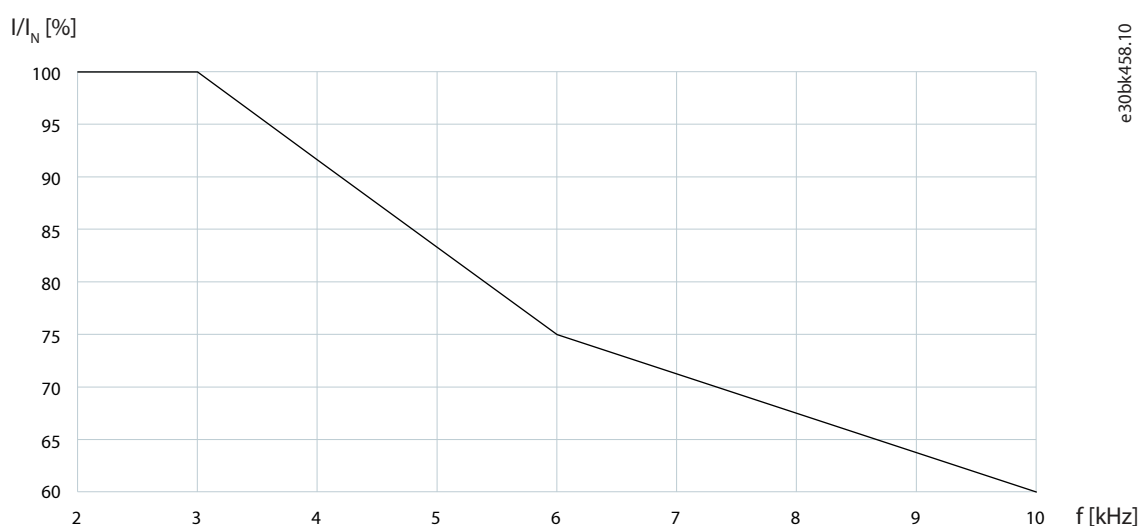
Figure 114: Switching Frequency Derating
