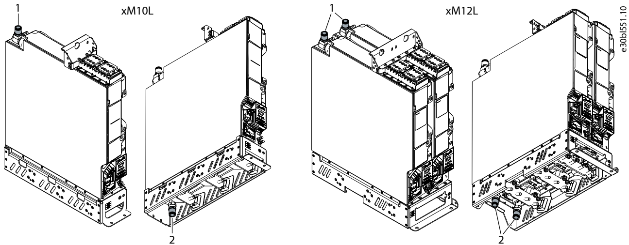
Figure 147: Inlet and Outlet Connectors of System Modules xM10L and xM12L
