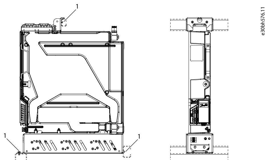
Figure 12: Mounting Holes of the System Module in Vertical Position
