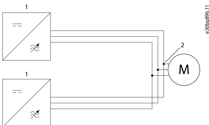
Figure 70: Recommended Installation
