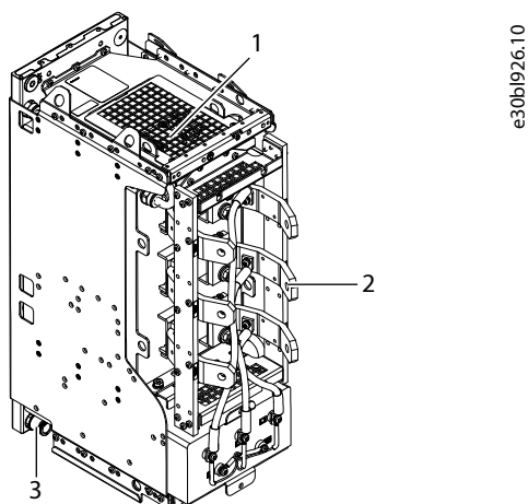
Figure 108: Liquid-cooled Sine-wave Filter
