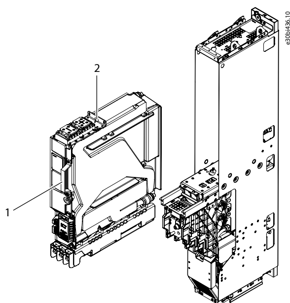
Figure 145: Lifting the System Module from the Integration Unit
