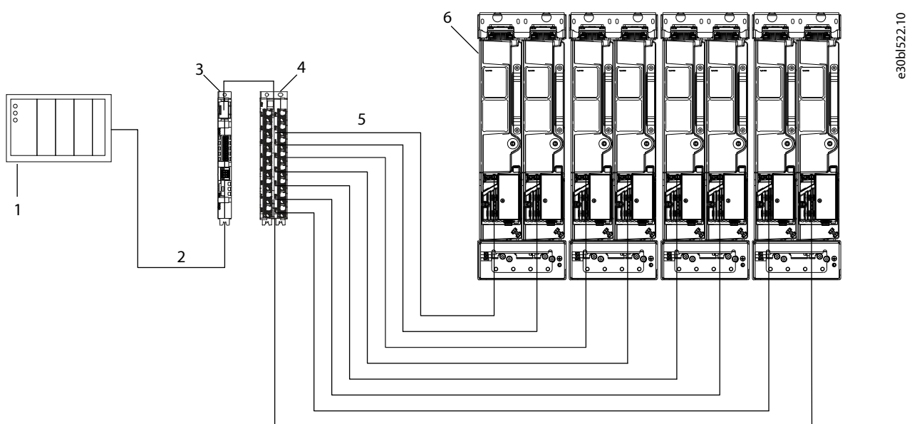
Figure 133: Connecting the Fieldbus Cable and the Fiber Cables
