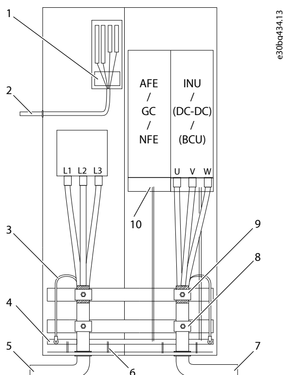
Figure 69: Cabling Principle
