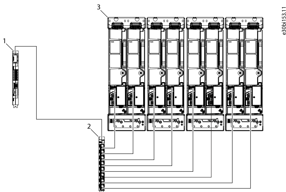
Figure 126: Example Control Connection with a Star Coupler Board: 8 Power Units in Parallel, Star Coupler Board near the Power Units
