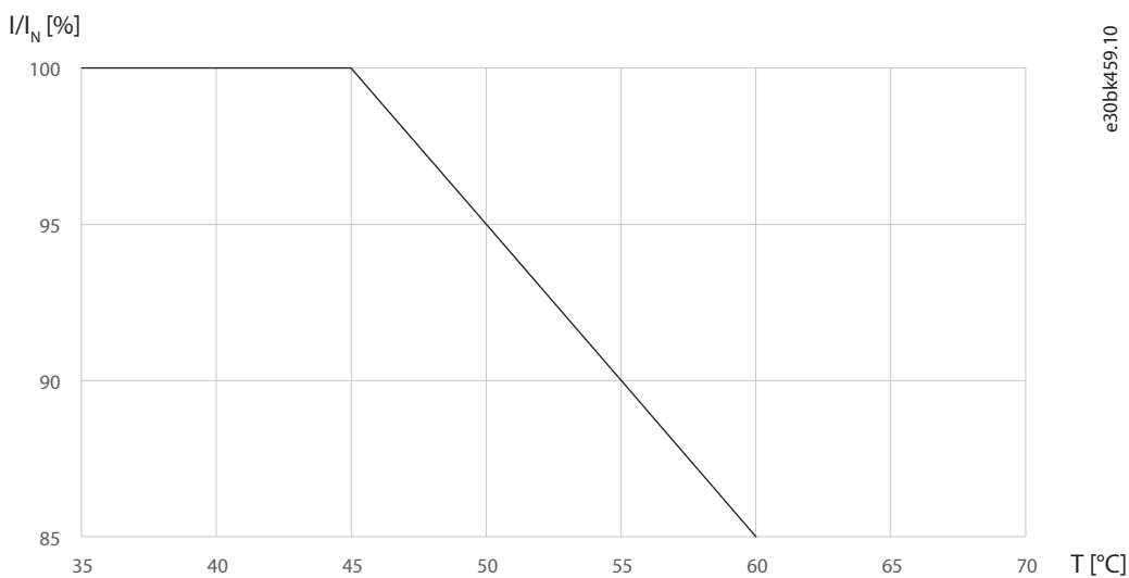
Figure 115: Coolant Temperature Derating
