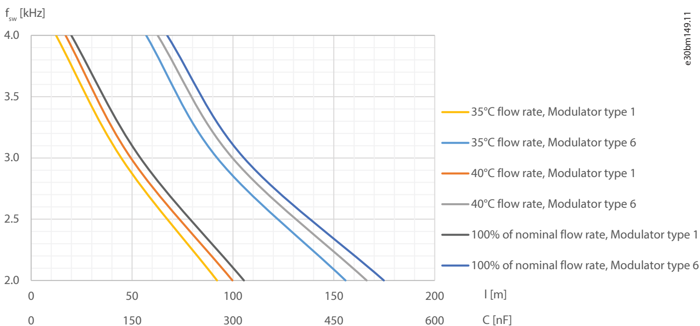
Figure 98: Safe Operation Area with Different Flow Rates: 820 A dU/dt Filter, 1122 V DC
