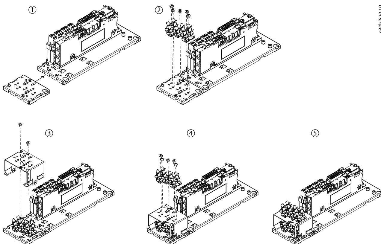
Figure 130: Assembling the Mounting Plate
