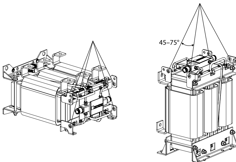
Figure 11: Example: Lifting the L Filter
