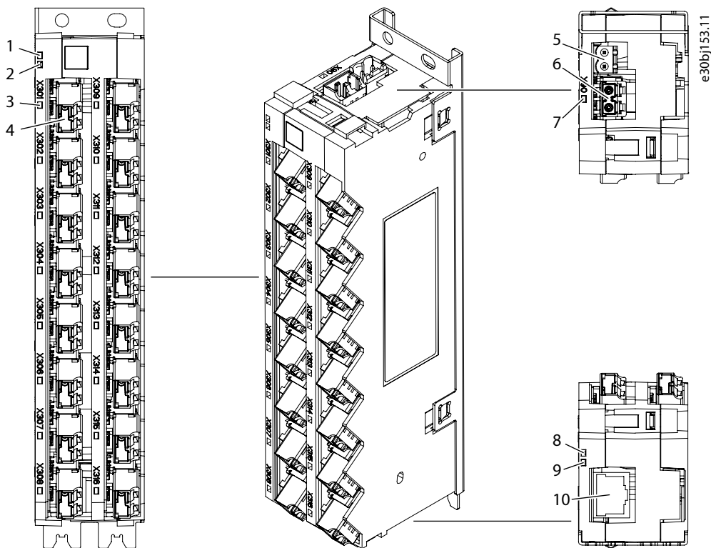
Figure 123: Terminal and Indicator Light Locations on the 16-port Star Coupler Board
