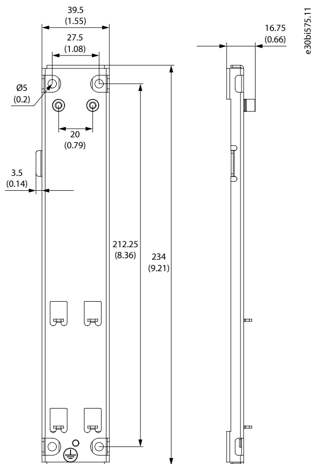
Figure 171: Dimensions of the Modular Control Unit Mounting Plate in mm (in), 2 Places
