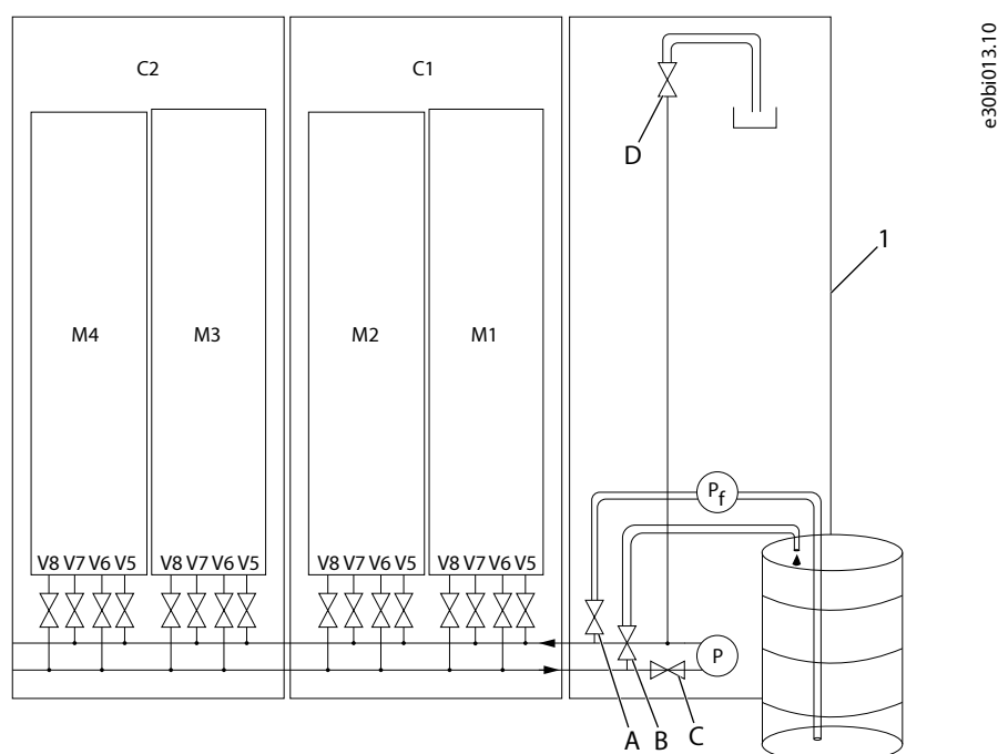
Figure 57: Example of Filling the Cooling System with Liquid
