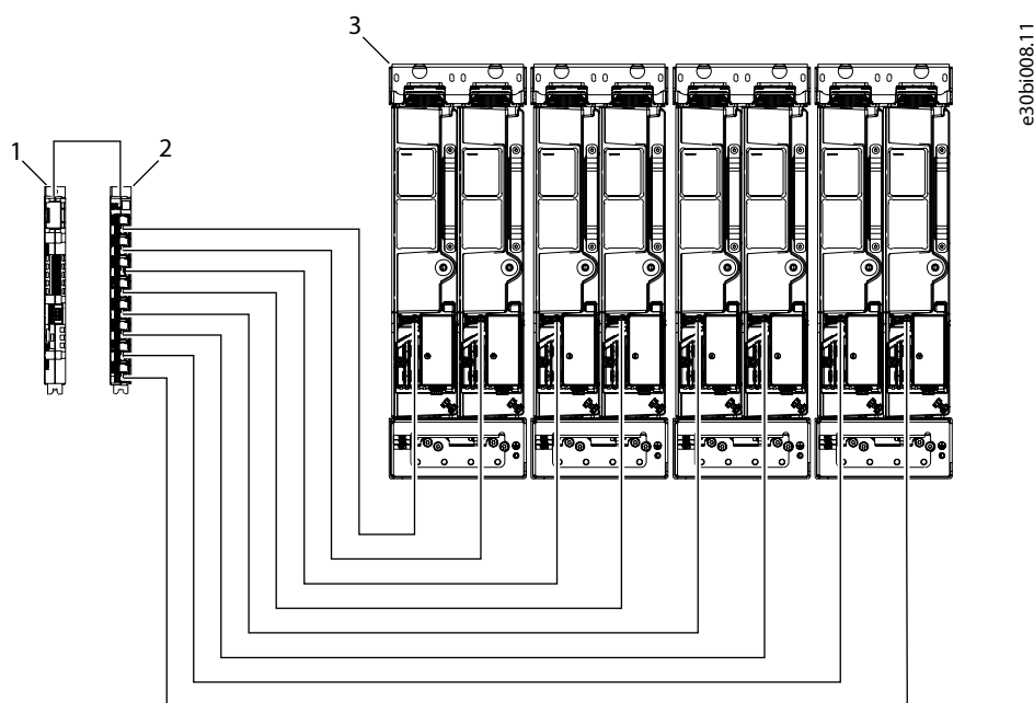
Figure 125: Example Control Connection with a Star Coupler Board: 8 Power Units in Parallel
