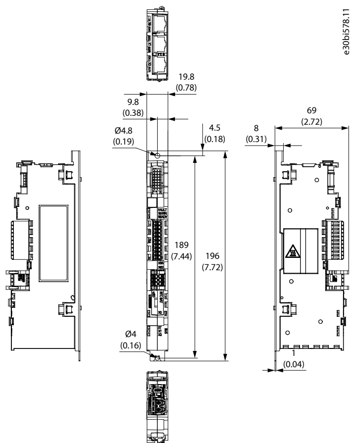
Figure 174: Dimensions of the Control Board in mm (in)
