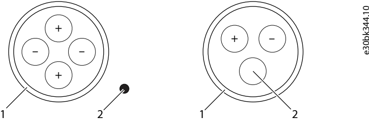
Figure 68: Recommended Cable Types for DC-source Cables
