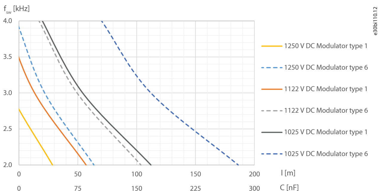
Figure 92: Safe Operation Area: 416 A dU/dt Filter, Low Output Frequency Range, 100% Flow
