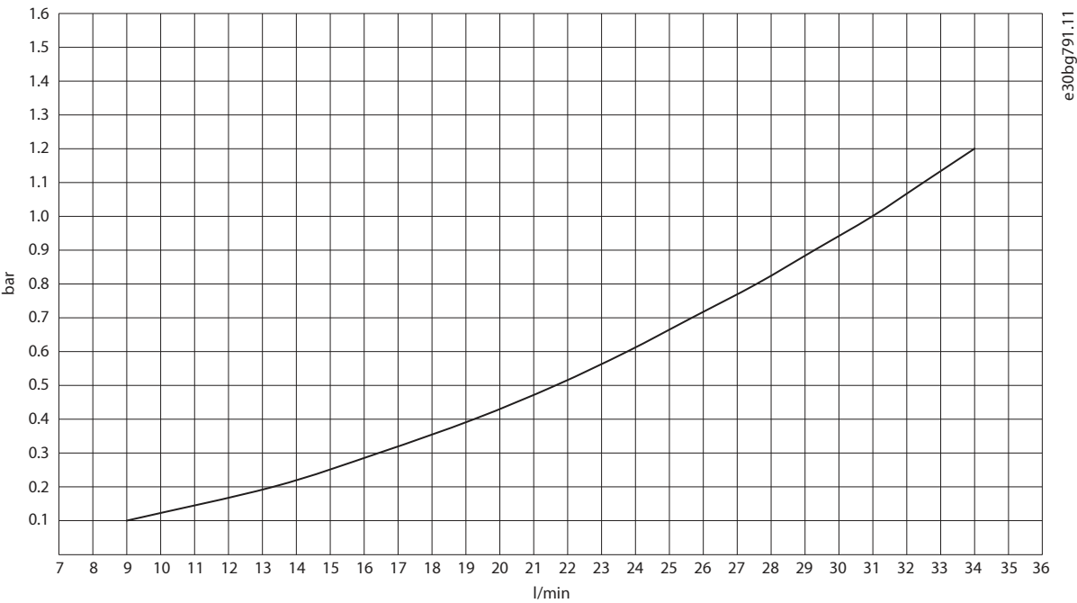
Figure 40: Pressure Drop with Water, dU/dt Filter OF7U1 (+AEU1), 820 A
