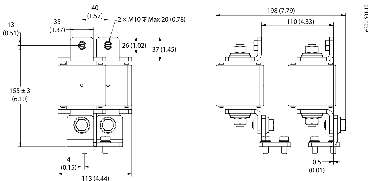
Figure 182: Dimensions of the DC Fuses, AR10L, IR10L, DR10L, AM10L, IM10L, DM10L, in mm (in)
