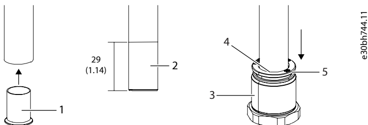
Figure 50: Inserting a Pipe into the Cooling Circuit Connector, mm (in)
