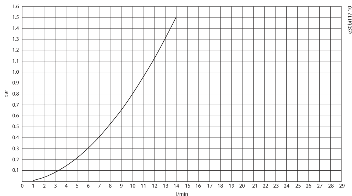
Figure 43: Pressure Drop, Grid-side L Filter OF7Z5, 690 V/1000 A
