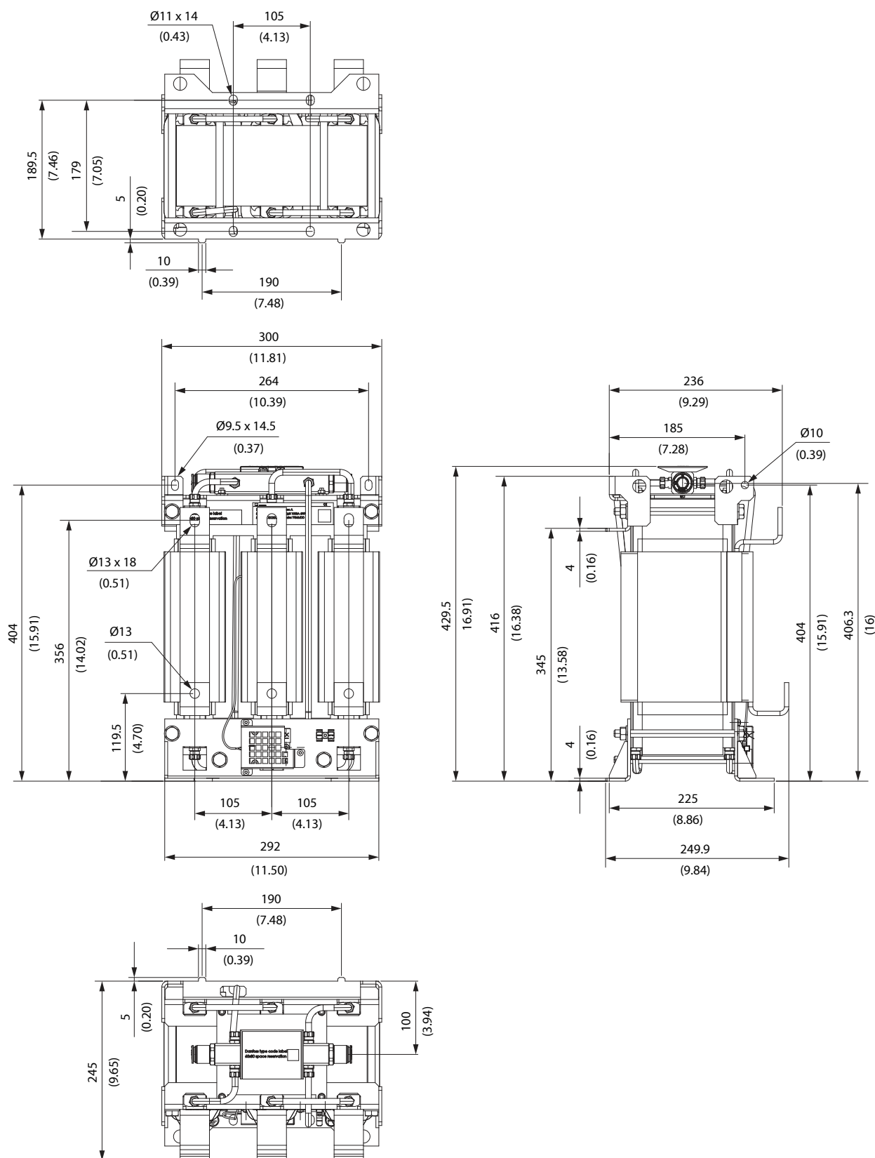
Figure 162: Dimensions of the L Filter, 1000 A
