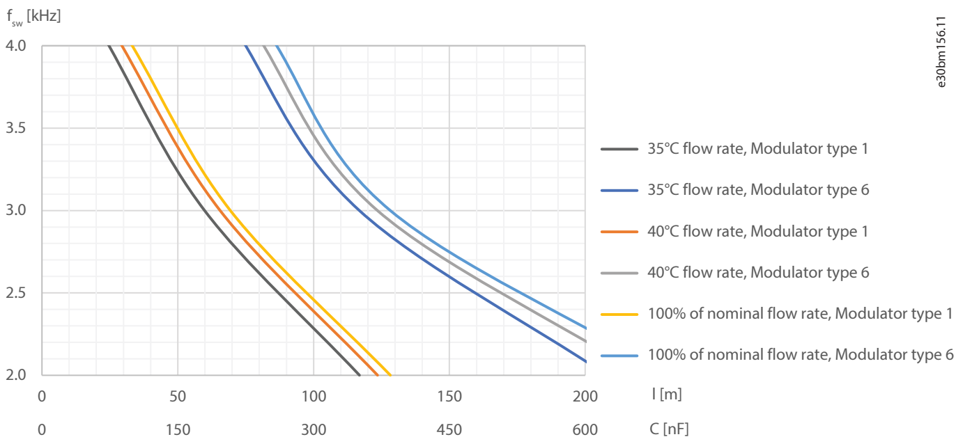
Figure 101: Safe Operation Area with Different Flow Rates: 820 A dU/dt Filter, Low Output Frequency Range, 1025 V DC
