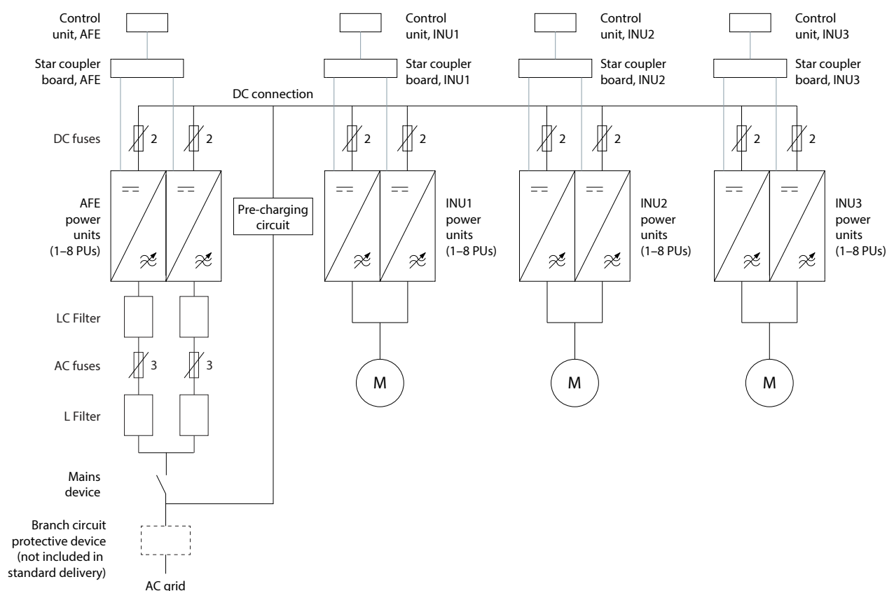
Figure 62: DC Connections of a Drive Lineup
