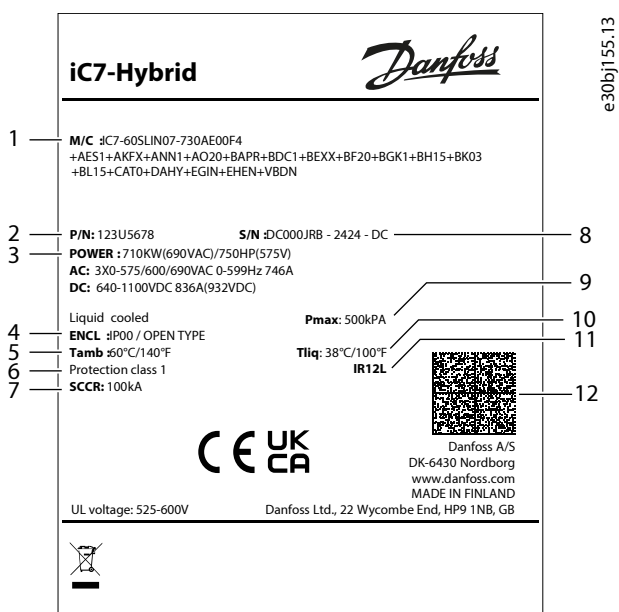
Figure 8: Product Label for iC7 Series Liquid-cooled System Modules
