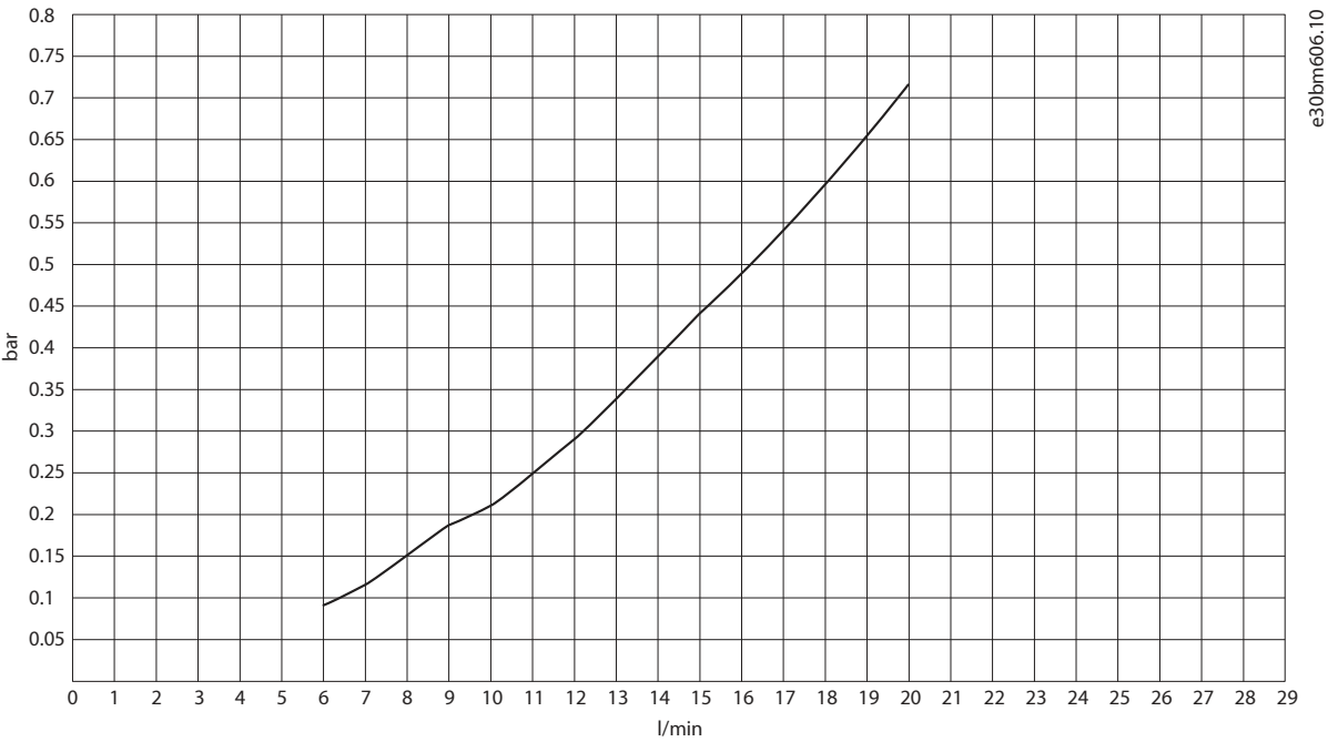
Figure 45: Pressure Drop, Grid-side L Filter OF7Z5, 690 V/2300 A
