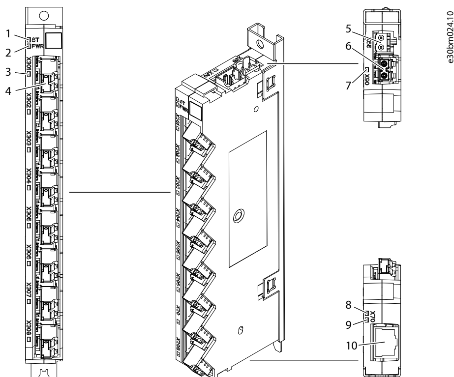
Figure 122: Terminal and Indicator Light Locations on the 8-port Star Coupler Board
