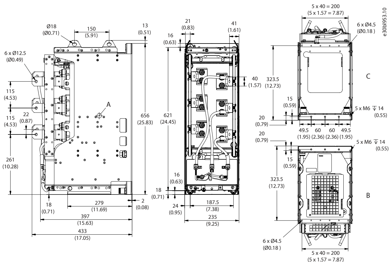
Figure 169: Dimensions of the Sine-wave Filter, in mm (in)
