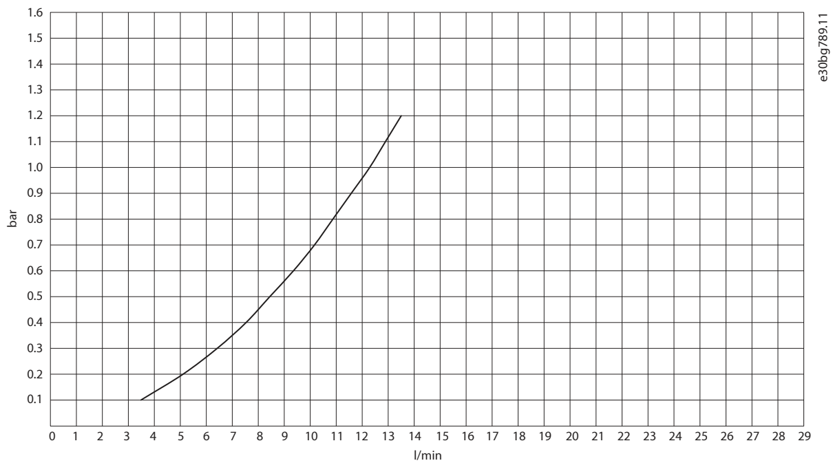
Figure 34: Pressure Drop with Water, LC Filter for AFE OF7Z1 (+AEZ1), 380 A
