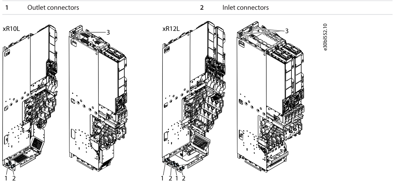
Figure 148: Inlet and Outlet Connectors of System Modules with Integration Units xR10L and xR12L
