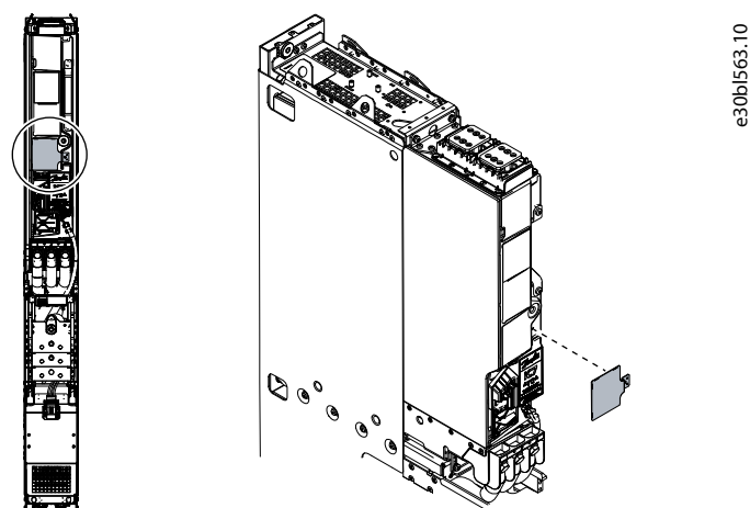
Figure 140: Mounting Location of the Product Label Plate
