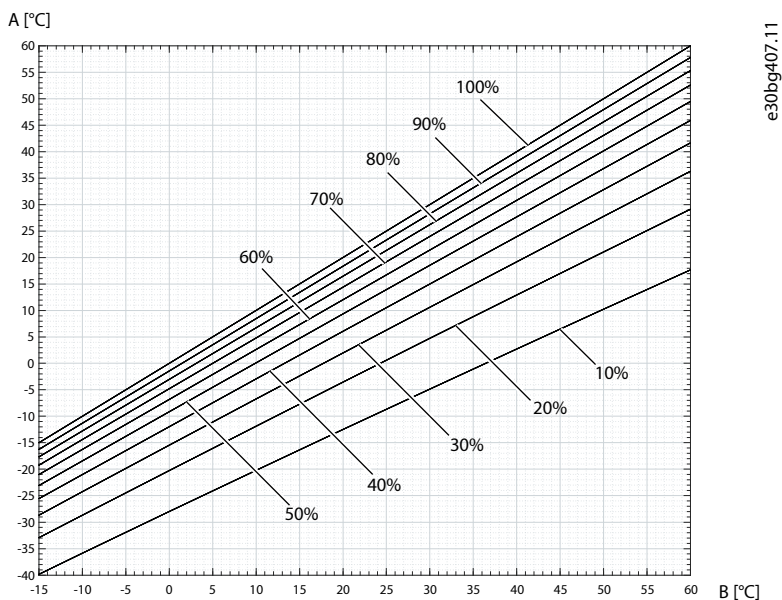
Figure 58: Dewpoint Temperature at Relative Humidity 100...10%
