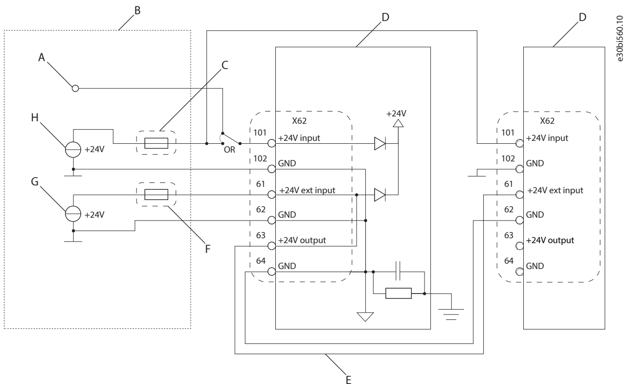
Figure 197: Wiring Diagram of Redundant Supplies
